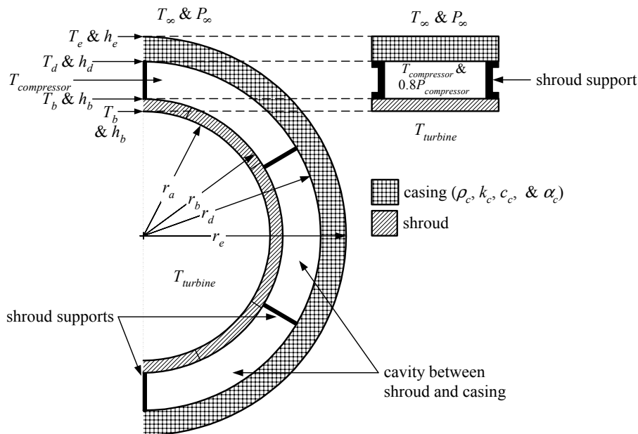
Figure 3. Shroud/casing schematic
