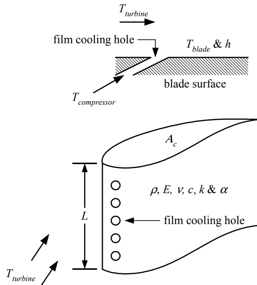
Figure 5. Blade schematic
