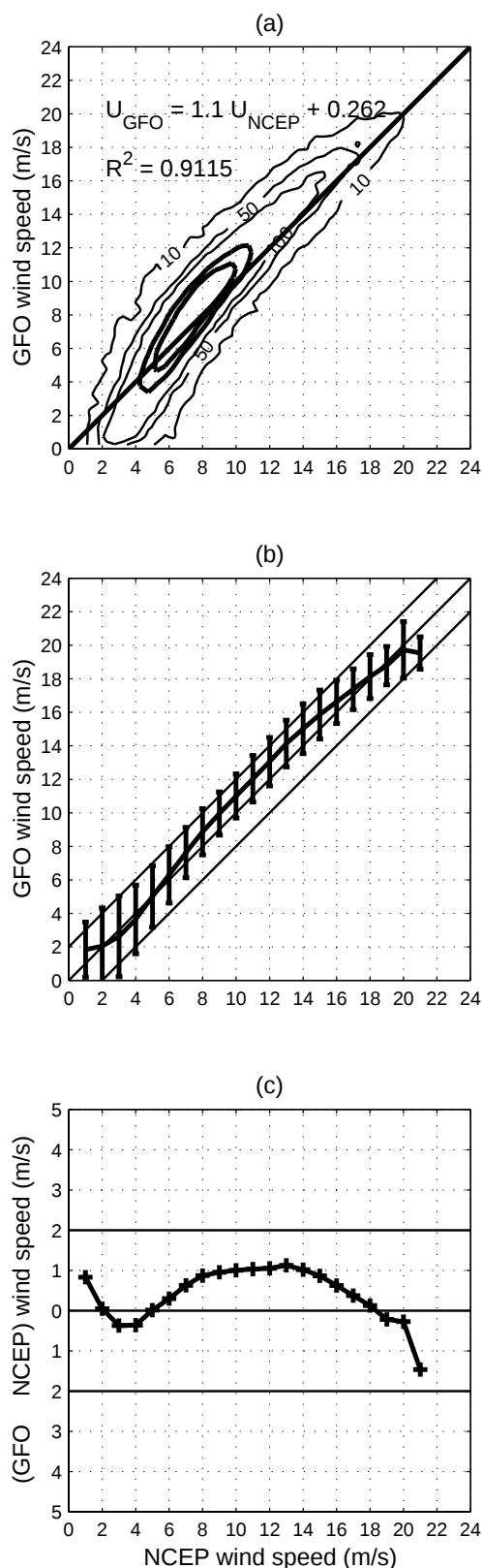
Figure 4-8 Comparison between GFO and NCEP Wind Speeds for Cycle #14
