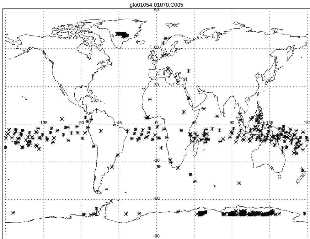
Figure 3-6 Attitude > .3, Cycle 5
