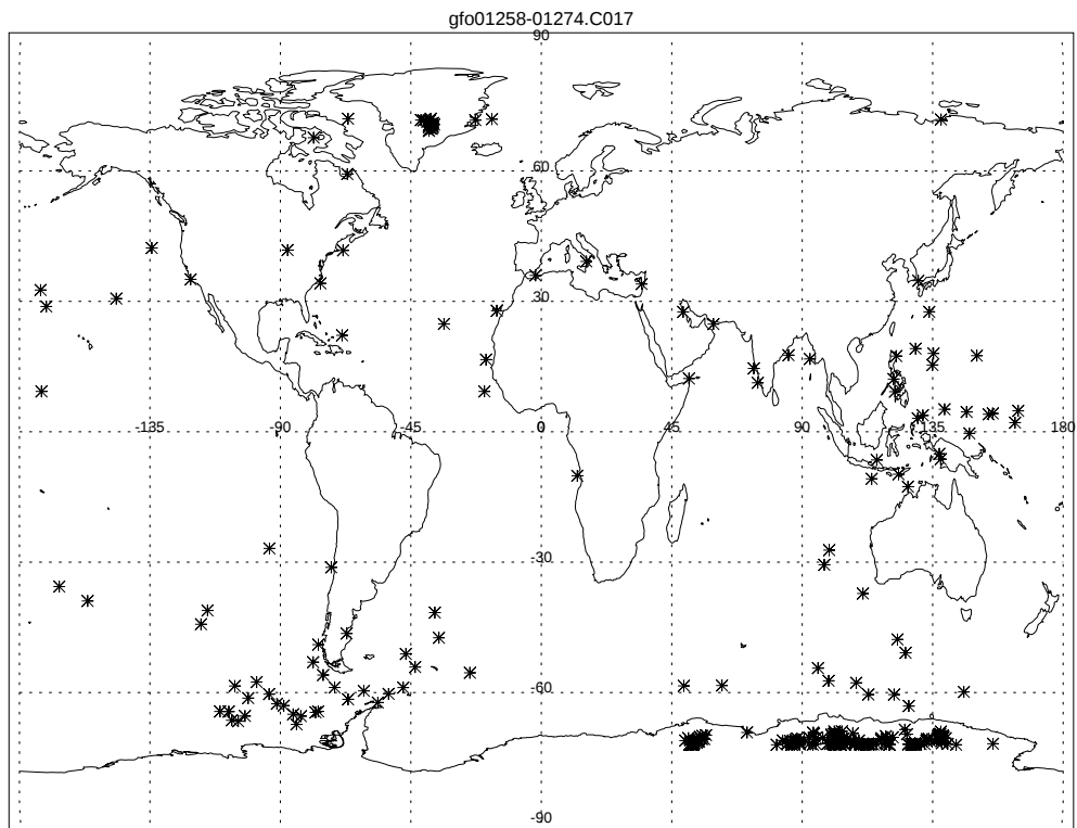
Figure 3-4 Attitude > .3, Cycle 17
