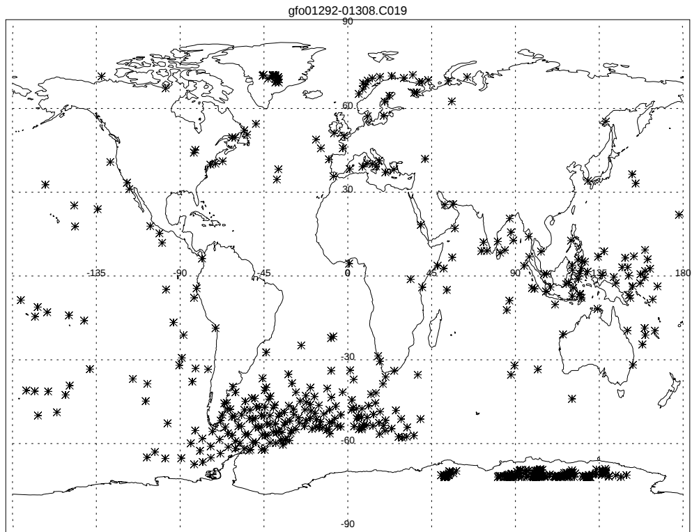
Figure 3-3 Attitude > .3, Cycle 19
