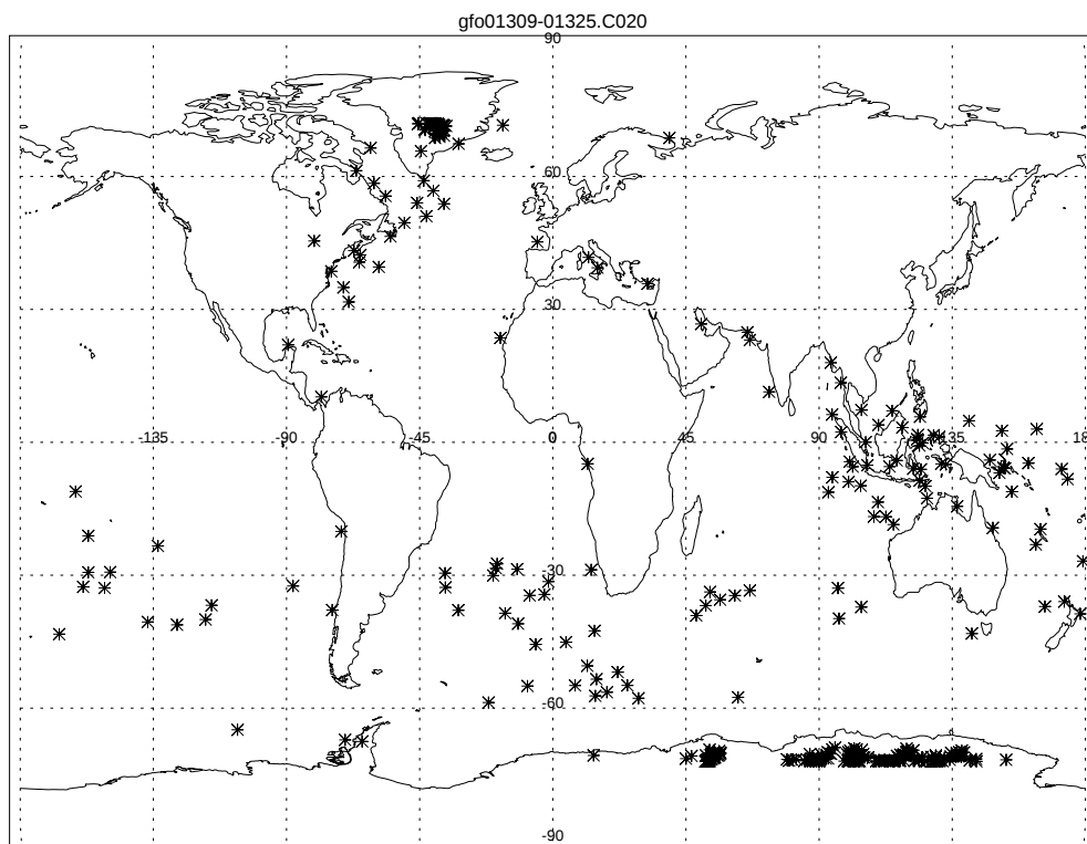
Figure 3-5 Attitude > .3, Cycle 20
