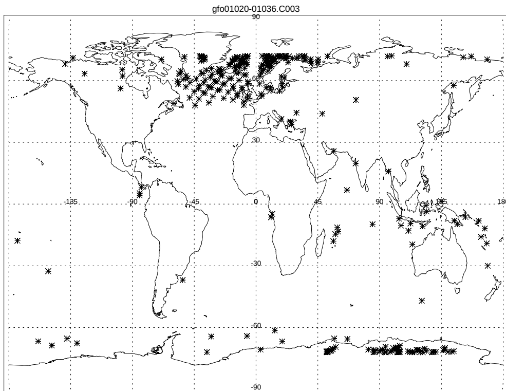
Figure 3-7 Attitude > .3, Cycle 3
