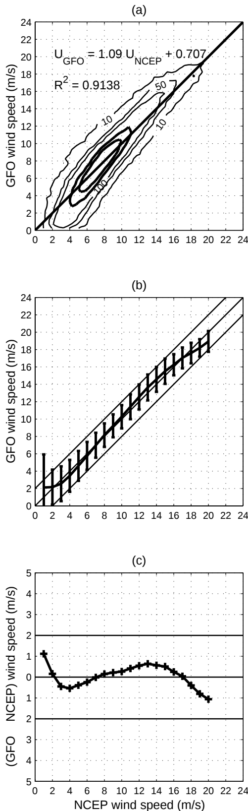
Figure 4-7 Comparison between GFO and NCEP Wind Speeds for Cycle #8
