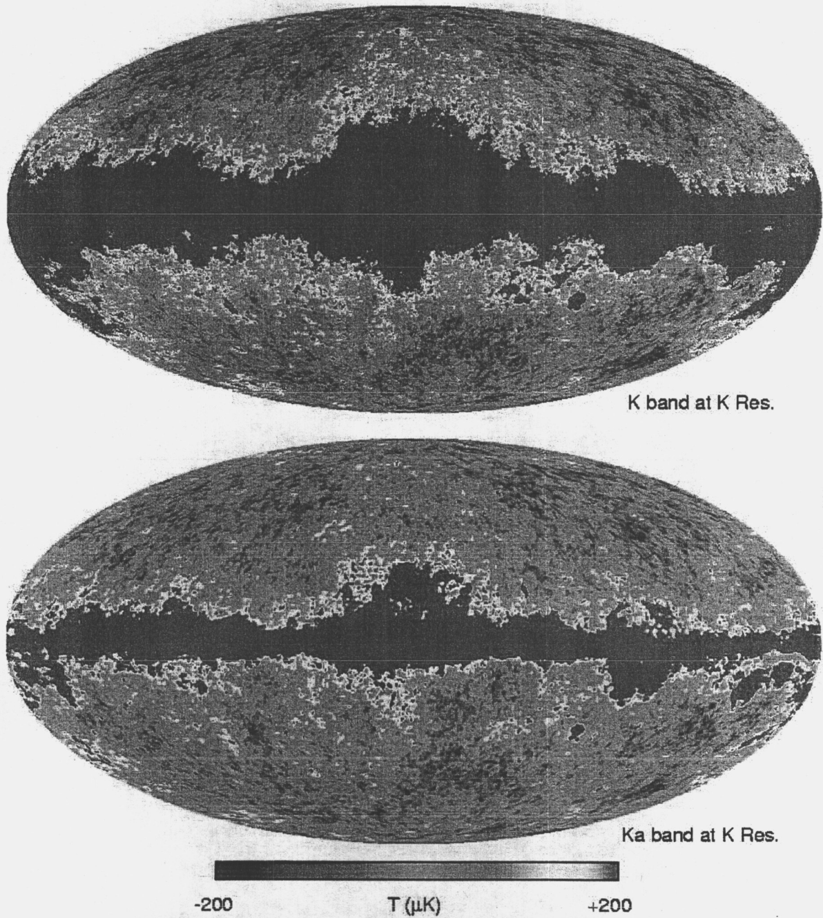
Fig. 5.— A comparison of the K-band map with the Ka-band map smoothed to K-band resolution, both in thermodynamic temperature, shows the dramatic reduction of Galactic contamination with increased frequency. The comparison also shows the similarity of the CMB fluctuation features at high Galactic latitude.
