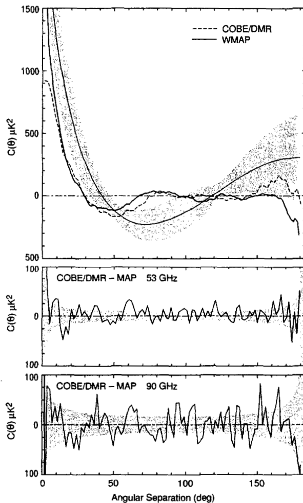
Fig. 13.— (top): CMB temperature correlation function of the WMAP and COBE data. The WMAP correlation function is computed using the Kp0 cut sky, and the COBE correlation function is computed using the “custom cut” sky. The running index \Lambda CDM model that is fit to the power spectrum is shown with a Monte Carlo determined grey band indicating one standard deviation. The model is, overall, an excellent fit to the WMAP power spectrum. However, a correlation plot emphasizes the low l power. The discrepancy between the model and data illustrates that there is surprisingly little anisotropy power in the WMAP and COBE maps at large angles. (bottom): The lower two plots display the correlation function of the difference between the COBE -DMR and WMAP maps with a |b| = 10^\circ Galactic plane cut. A synthesis of the WMAP Q and V band maps was made to approximate a 53 GHz-like map to compare with the COBE -DMR 53 GHz map. The COBE -DMR 90 GHz map is compared directly, without corrections, to the WMAP W-band map. These plots emphasize the consistency of the WMAP and COBE measurements. The slightly higher than expected deviations at 53 GHz are likely to be due to Galactic contamination, arising from outside the cut regions and from the construction of the synthesized WMAP 53 GHz map.
