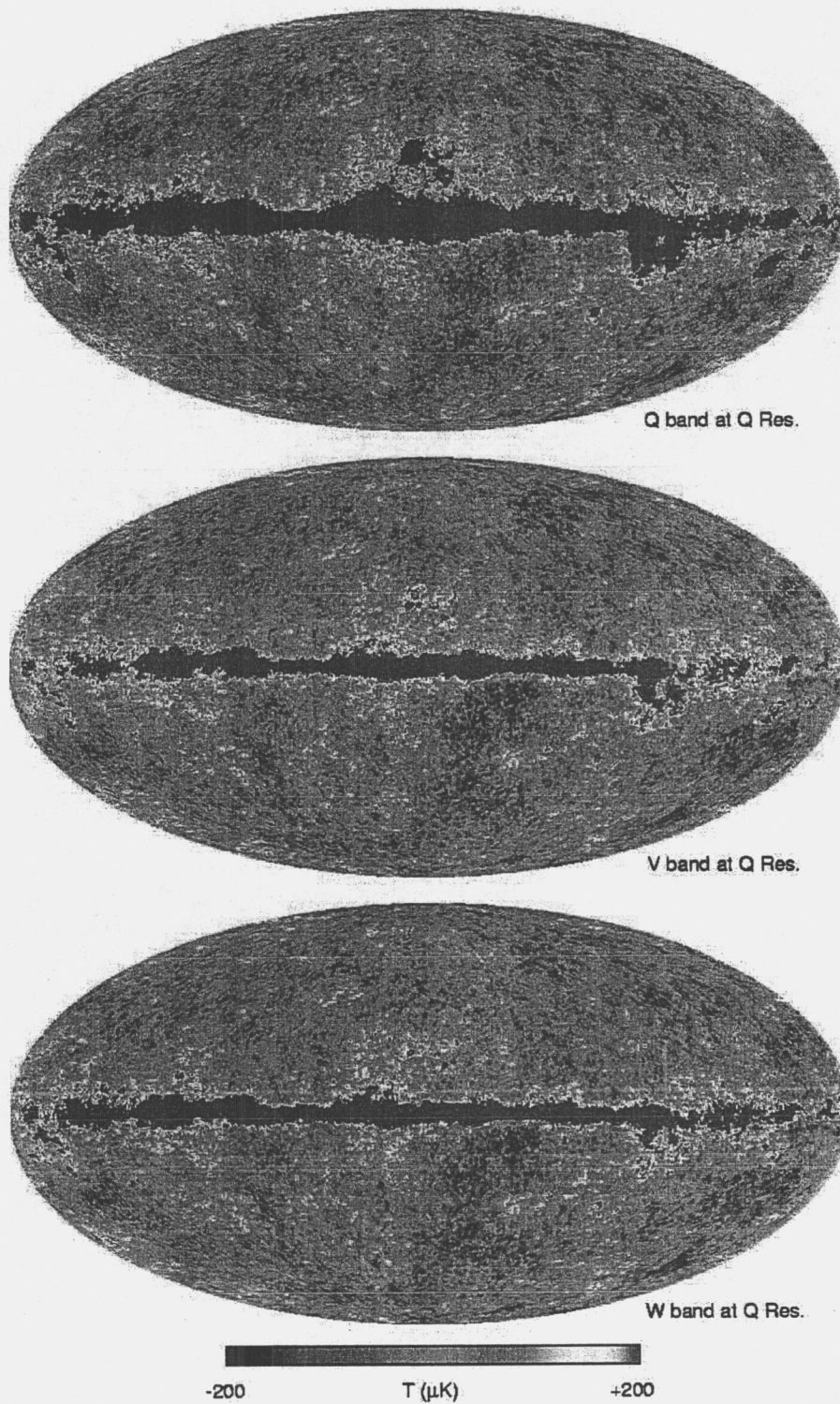
Fig. 6.— A comparison of the Q-band, V-band, and W-band maps. All three maps are smoothed to Q-band resolution and are in thermodynamic temperature. The reduction of Galactic contamination relative to K-band and Ka-band (Figure 5) is apparent. The maps show that the constant features across bands are CMB anisotropy while the thermodynamic temperature of the foregrounds depends on the band (frequency).
