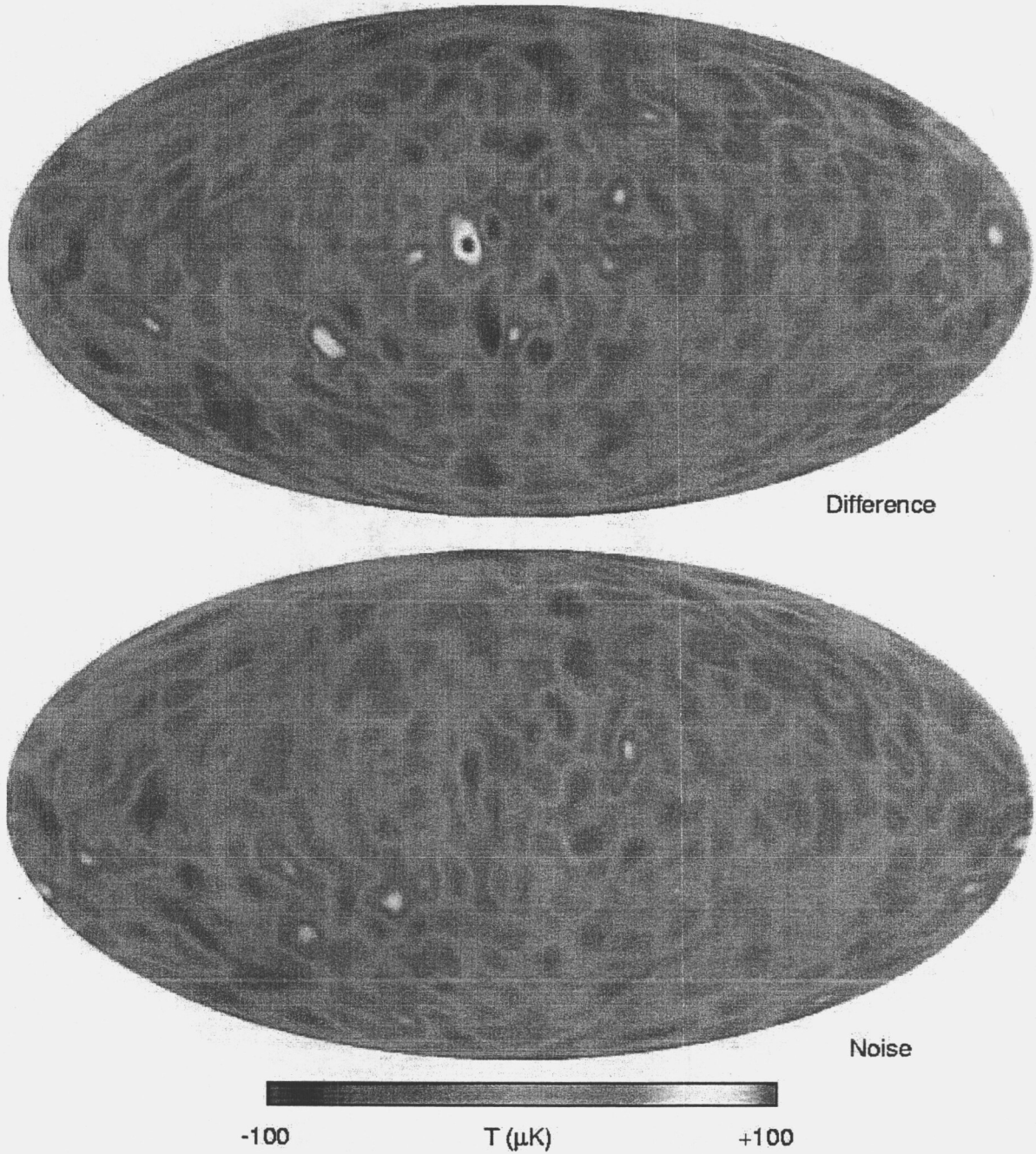
Fig. 9.— The difference map is shown between the COBE -DMR 53 GHz map and the combination Q-band/V-band maps from Figure 8. This is compared with a map of the noise level. The maps are consistent with one another with the exception of a feature in the galactic plane. This discrepancy is likely to be due to a spectral index that is sufficiently different from the assumed CMB spectrum used to combine the WMAP Q-band and V-band maps to mimic a 53 GHz map.
