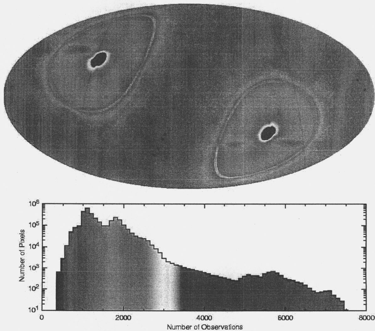
Fig. 3.— The number of independent observations per pixel in Galactic coordinates. The number of observations is greatest at the ecliptic poles and in rings around the ecliptic poles with diameters corresponding to the separation angle of the two optical boresight directions (approximately 141^\circ ). The observations are the most sparse in the ecliptic plane. Small area cuts are apparent where Mars, Saturn, Jupiter, Uranus, and Neptune data are masked so as not to contaminate CMB analyses. Jupiter data are used for beam mapping. The histogram of the sky sampling shows the departures from uniform sky coverage.
