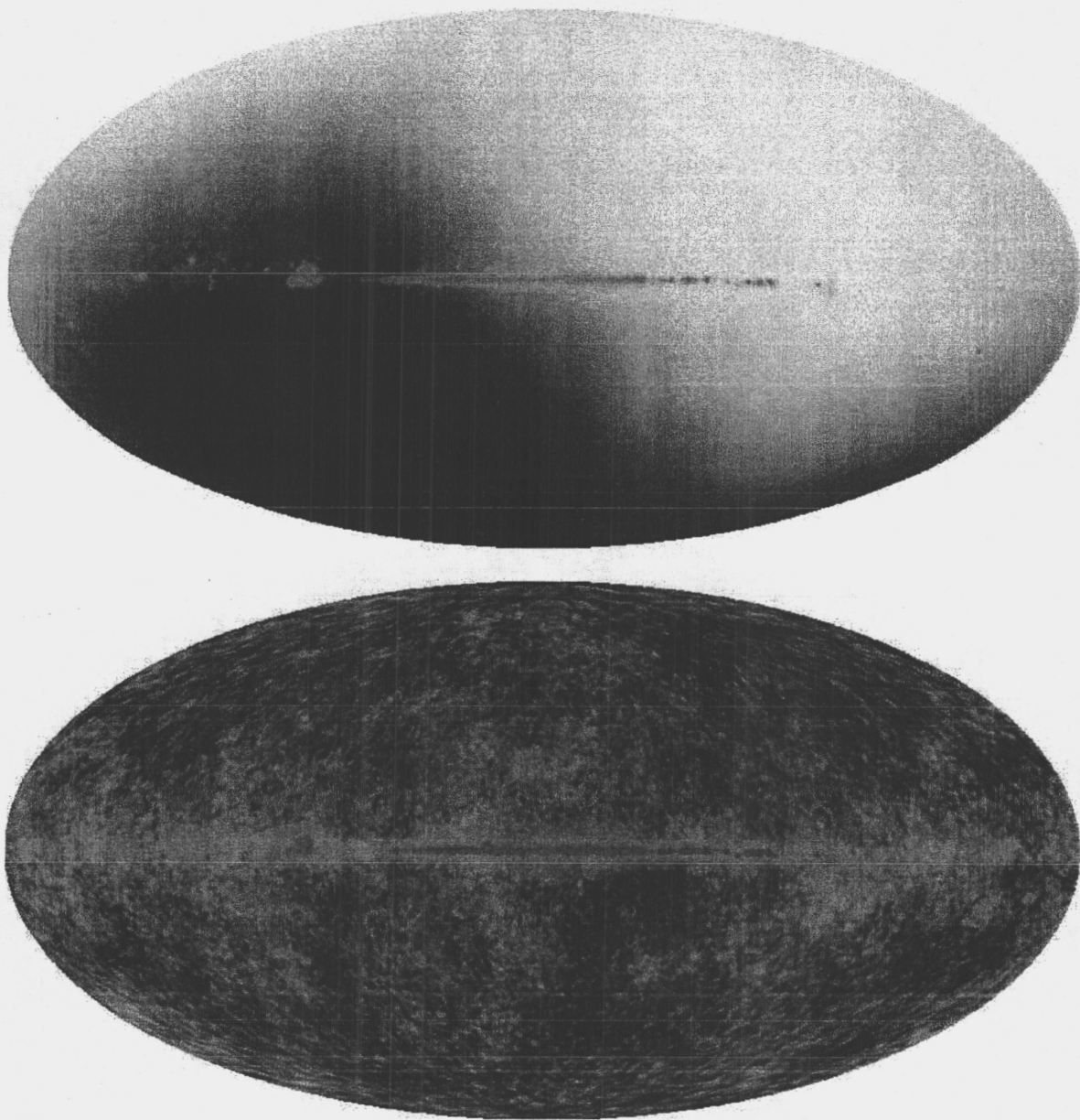
Fig. 10.— False color images represent the spectral information from multiple WMAP bands. Q-band is red, V-band is green, and W-band is blue. A CMB thermodynamic spectrum is grey. (top) A three color combination image from the Q-, V-, and W-band maps. The dipole and high Galactic latitude anisotropy are seen. (bottom) A similar false color image but with the dipole subtracted.
