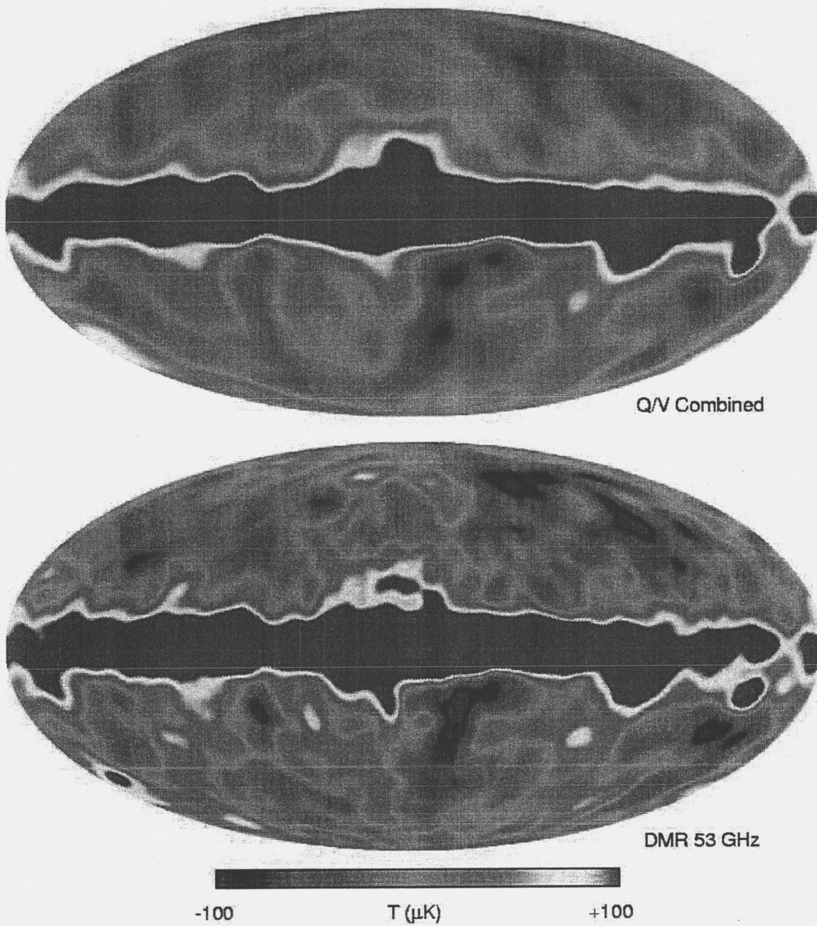
Fig. 8.— The COBE -DMR 53 GHz map (Bennett et al. 1996) is shown along with a map made with a linear combination of the Q-band and V-band WMAP maps to mimic a 53 GHz map. Note the strong similarity of the maps.
