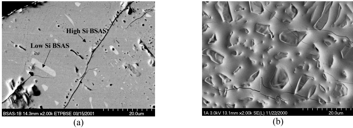
Figure 1.—(a) The BSAS coating was decomposed into low Si (bright second phase) and high Si (dark matrix) phases during initial laser thermal cyclic testing. (b) The higher Si phase became the glass phase and surface cracks were formed after 100 hour cyclic testing at the surface temperature of 1482 °C.
