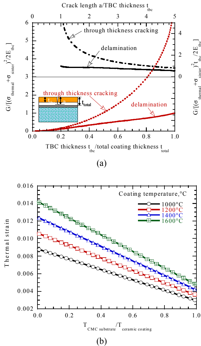
Figure 4.—(a) ZrO_2\text{-}Y_2O_3 TBC layer on mullite-BSAS EBC and CMC substrates, the coating surface cracking and delamination energy release rates can increase significantly with a relatively thick, and larger thermal expansion ZrO_2\text{-}Y_2O_3 TBC layer on mullite-BSAS EBC on CMC substrates. (b) The significantly larger thermal stresses/strains will be generated with increasing the thermal gradients (the temperature difference between the ceramic coating and the substrates).
