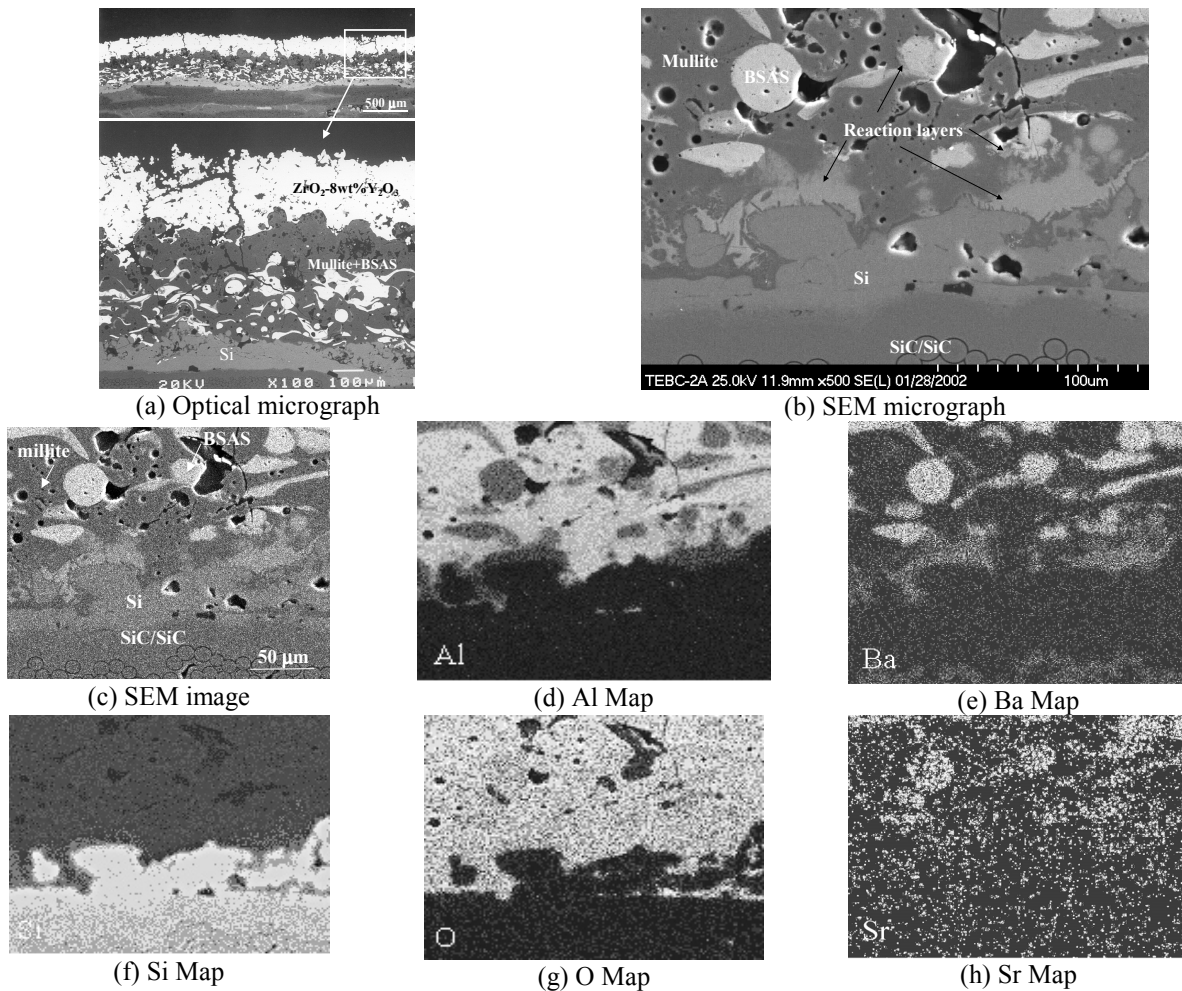
Figure 3.—SEM images and EDS element composition maps of the ZrO_2-8wt\%Y_2O_3/BSAS+mullite mixture/Si on SiC/SiC ceramic matrix composite substrates after laser testing, showing significant interface reactions between BSAS and bond coat Si layer, and the BSAS and mullite. (a) and (b) Optical and SEM micrographs of the coating after 100 hours testing, showing the surface cracking and interface reactions; and (c) to (h) SEM cross-section micrograph and the corresponding EDS elemental maps for the coating systems near the interface.
