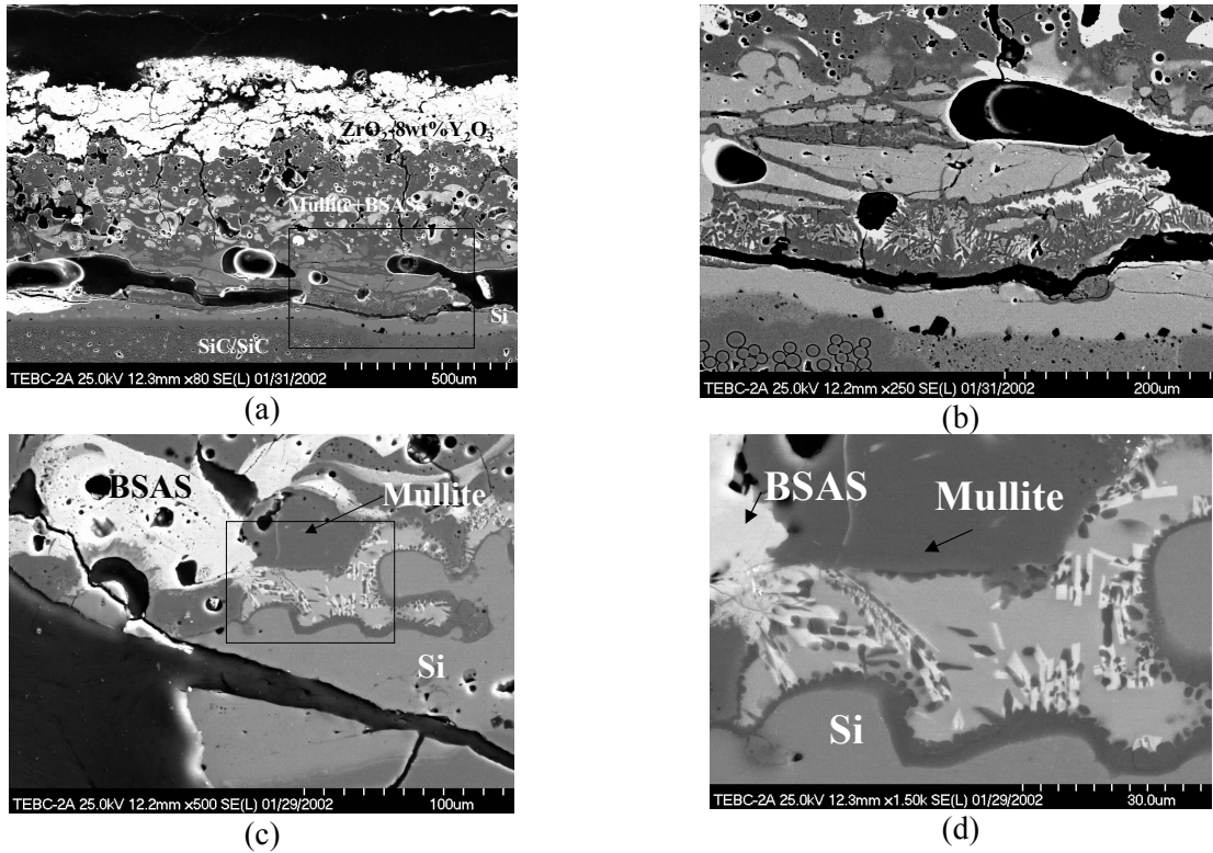
Figure 5.—SEM cross-section micrographs of the ZrO_2-8wt\%Y_2O_3/BSAS+mullite mixture/Si on a SiC/SiC ceramic matrix composite substrate, after total 400 hours testing in the combined laser thermal gradient and furnace water vapor cyclic testing. (a) Significant interfacial pore formation due to the water vapor attack through the vertical cracks under the thermal gradient cycling conditions. (b) Low melting eutectic phase was also observed near the BSAS-mullite-Si interfaces after the testing.
