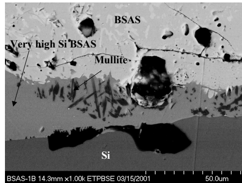
Figure 2.—SEM cross-section micrograph of the BSAS coating after 100 hour laser thermal gradient cycling test. The interface reactions resulted in a dark reaction BSAS layer with high Si concentrations. The mullite phase (very dark needle-shaped phase) precipitation was also found within the high Si reaction BSAS region.
