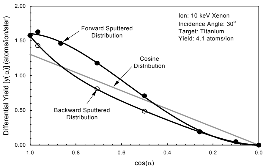
Fig. 4c Differential sputter yield measurements for 10 keV Xe ions on a Ti target (30° incidence)
