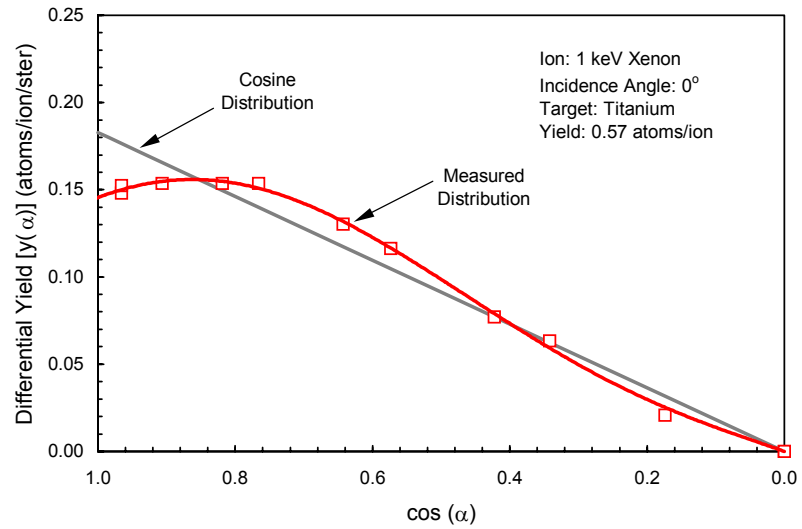
Fig. 2a Differential sputter yield measurements for Xe ions on a Ti target (normal incidence).
