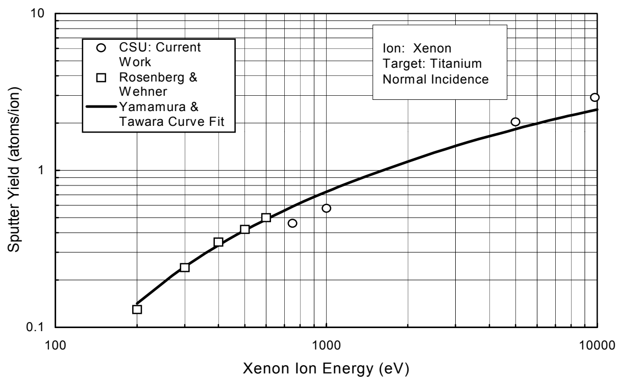
Fig. 5a Comparison of Ti sputter yield data to Rosenberg and Wehner
