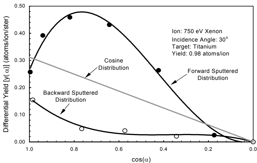
Fig. 4a Differential sputter yield measurements for 750 eV Xe ions on a Ti target (30° incidence)
