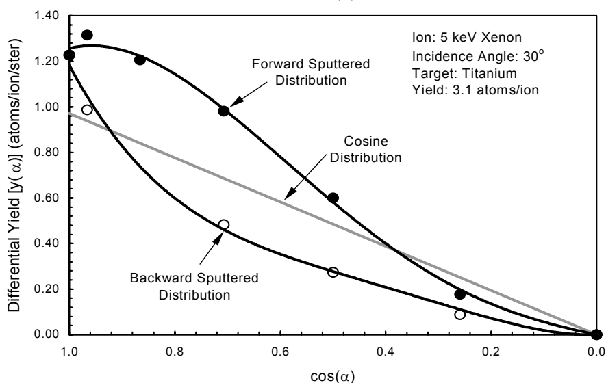
Fig. 4b Differential sputter yield measurements for 5 keV Xe ions on a Ti target (30° incidence)
