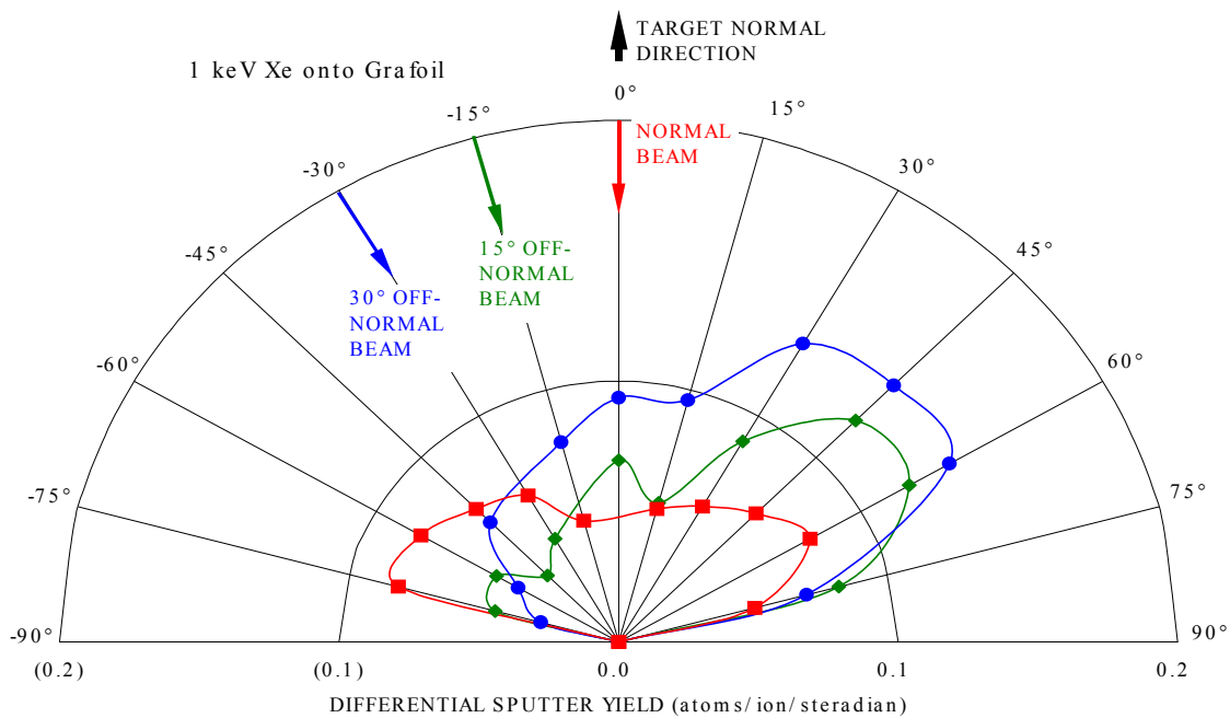
Fig. 7b Differential sputter yield measurements for 1 keV Xe ions on a flexible graphite (grafoil) target ( for 0°, 15°, and 30° incidence)
