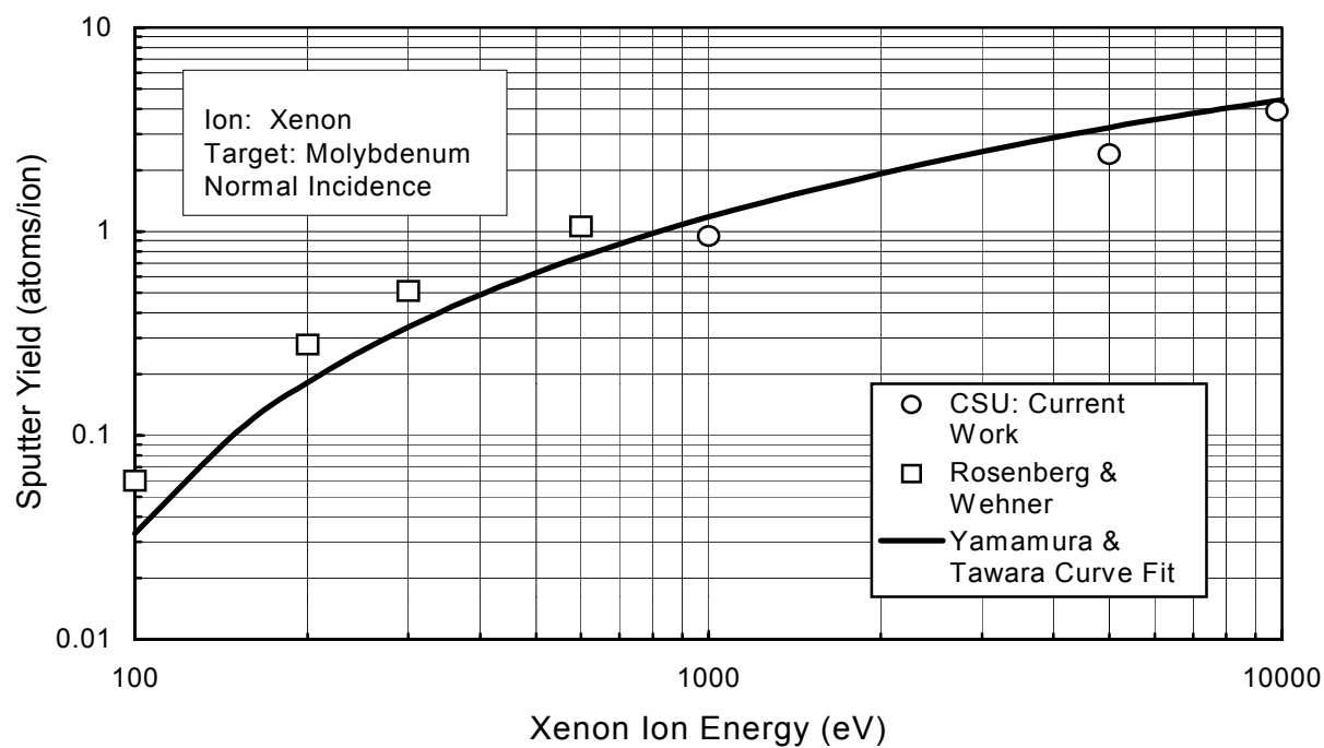
Fig. 5b Comparison of Mo sputter yield data to Rosenberg and Wehner
