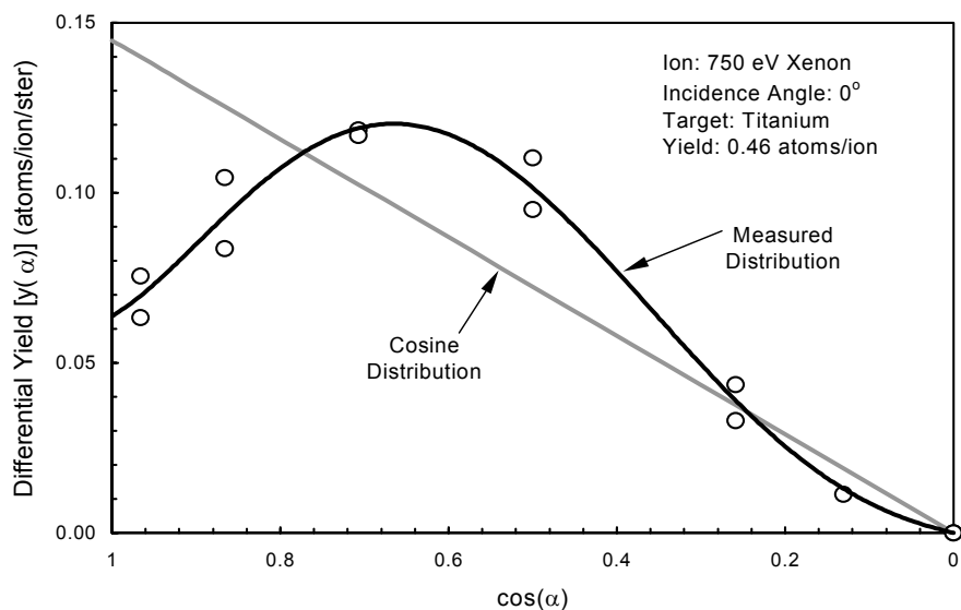
Fig. 3a Differential sputter yield measurements for 750 eV Xe ions on a Ti target (normal incidence)
