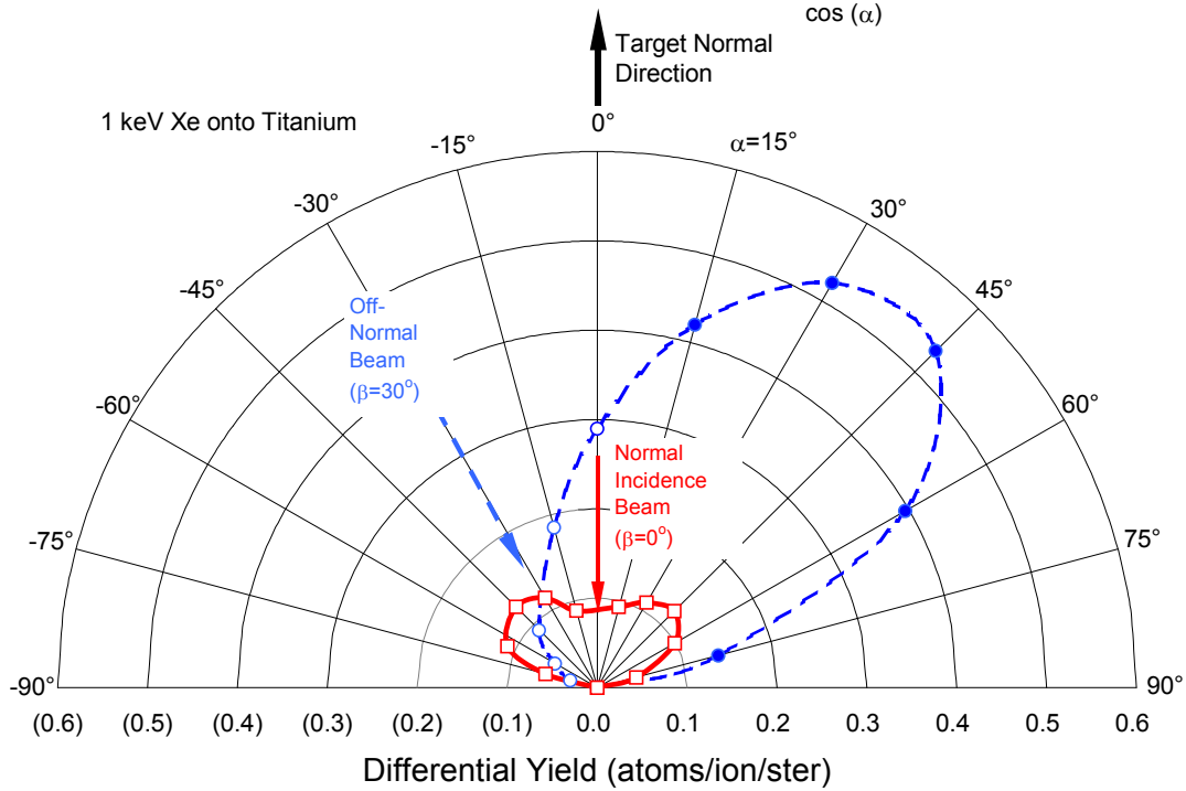
Fig. 2c Polar plot of differential sputter yield measurements for Xe ions on a Ti Target ( 0^\circ and 30^\circ incidence).
