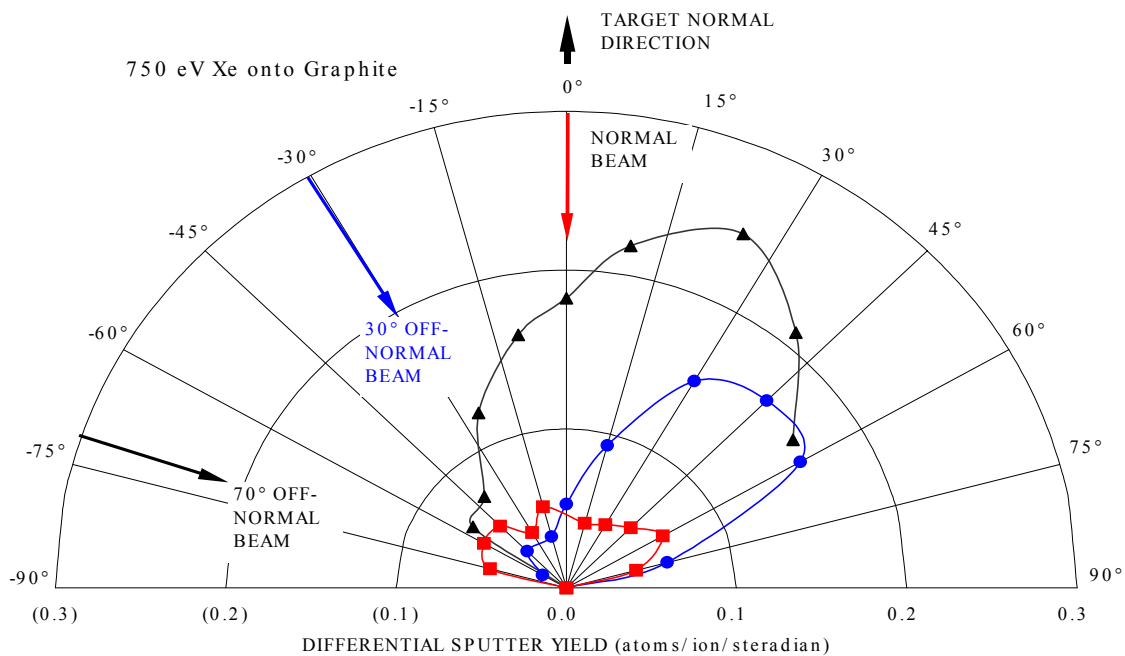
Fig. 7a Differential sputter yield measurements for 750 eV Xe ions on a Poco graphite target ( for 0°, 15°, and 30° incidence)
