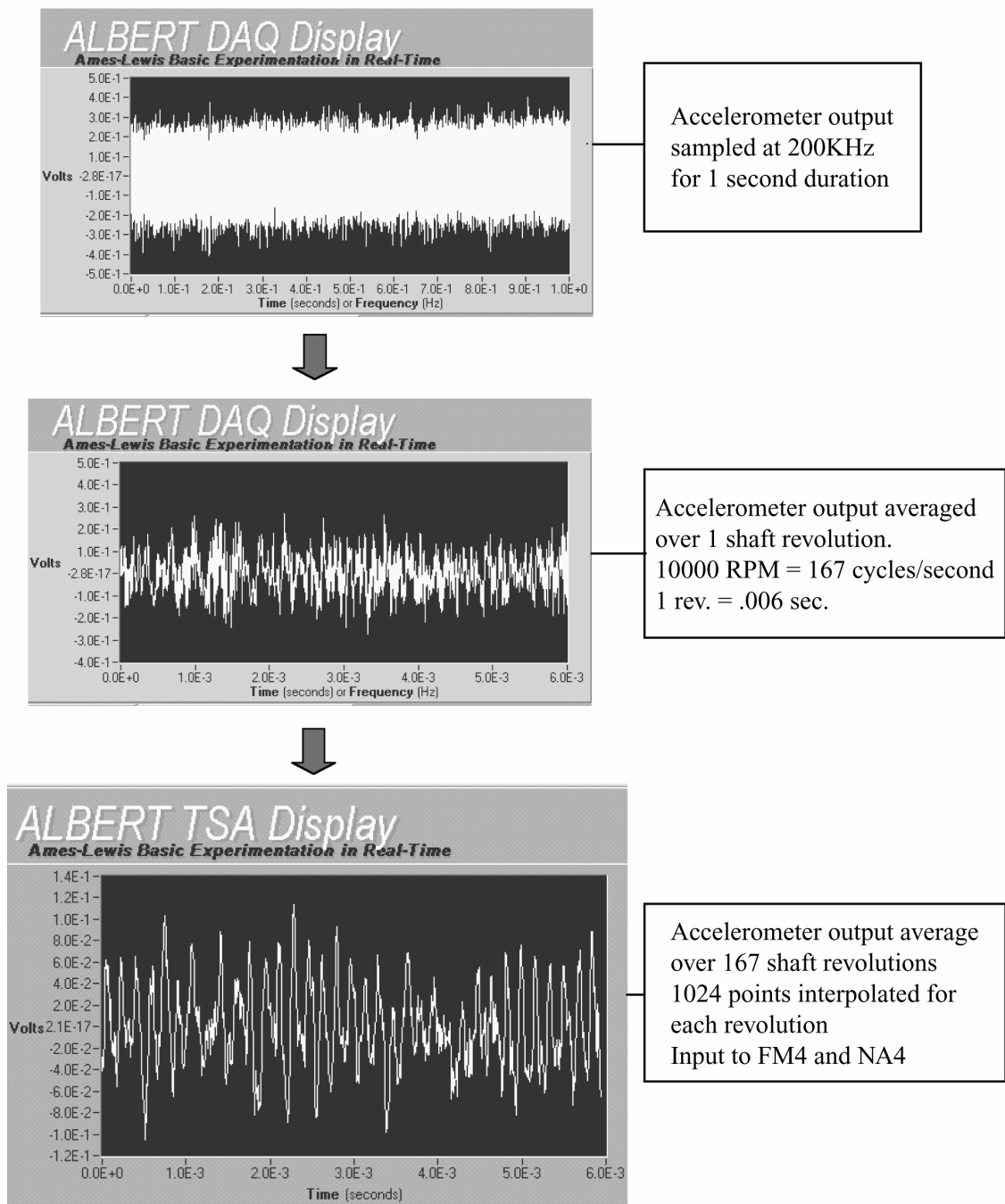
Figure 3.1.—Time synchronous averaging of vibration data.
