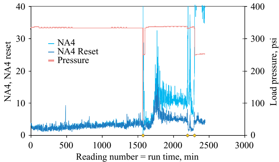
Figure 3.18.—Data from experiment 2 illustrating load effects.
