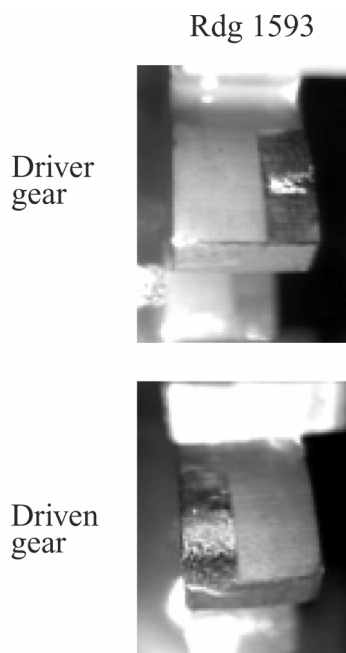
Figure 3.34.—Damage progression of driver/driven tooth 26 for experiment 20
