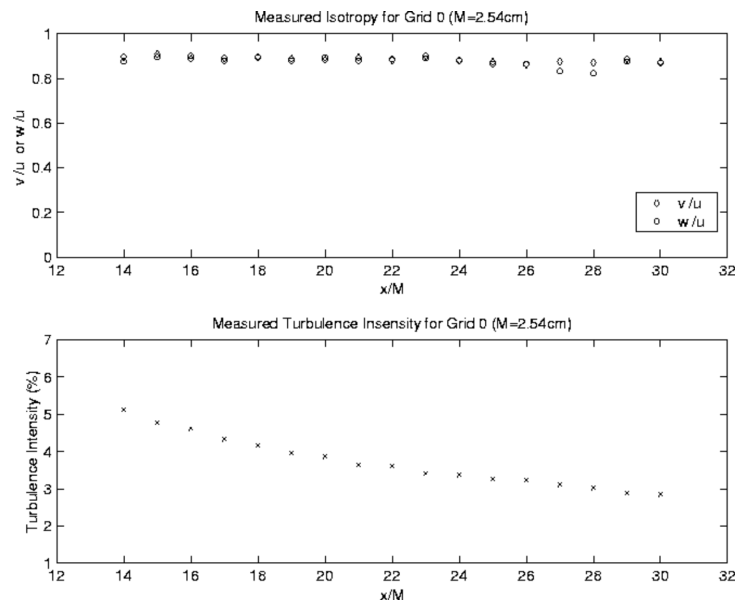
Figure 7: Turbulence intensity ( u'/U_\infty ) and isotropy ( v'/u' and w'/u' ) as a function of streamwise distance for “Grid 0”.
