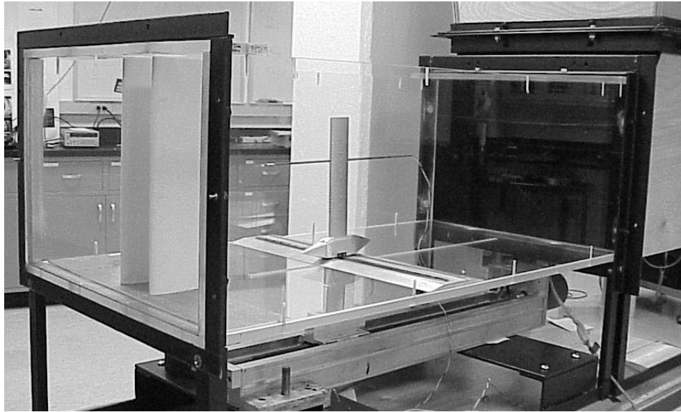
Figure 16: Photograph of tunnel test section which shows two of the airfoils used for the moving wake setup.
