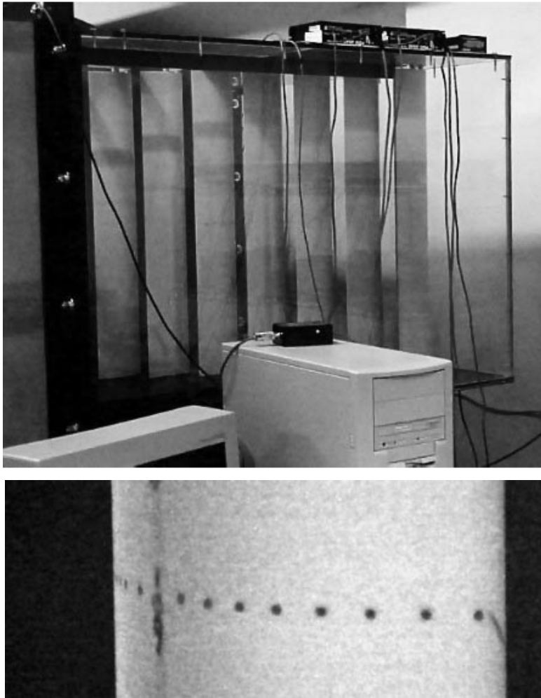
Figure 1: Photograph of Pak-B cascade and enlarged view of upper surface pressure ports.
