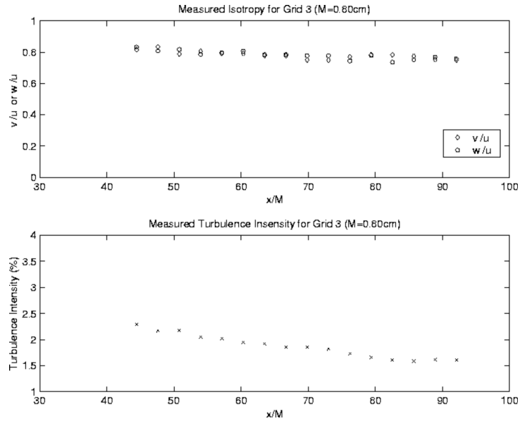
Figure 6: Turbulence intensity ( u'/U_\infty ) and isotropy ( v'/u' and w'/u' ) as a function of streamwise distance for “Grid 3”.
