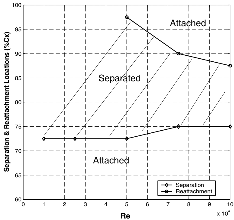
Figure 4: Blade separation and reattachment locations as a function of Reynolds number for lowest free-stream turbulence level ( u'/U_\infty = 0.08\% ).
