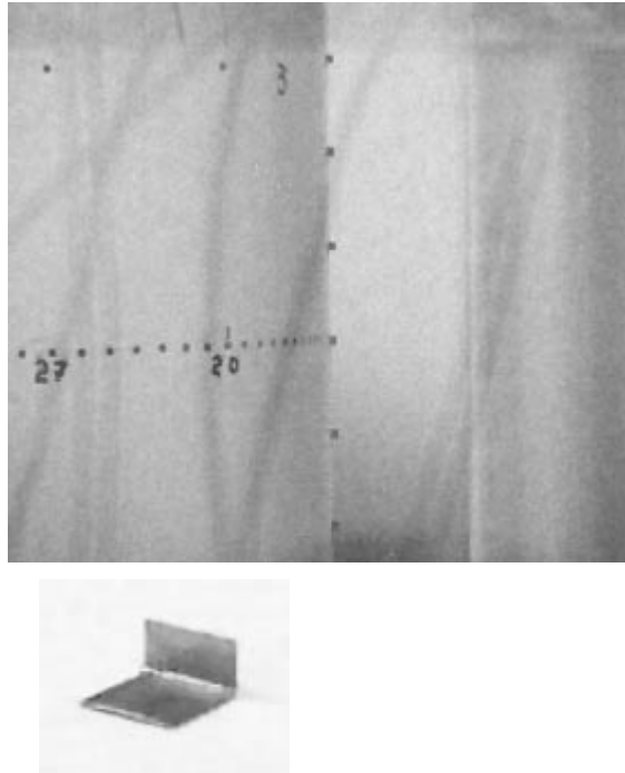
Figure 11: Photograph of vortex generators on center blade in cascade, and an individual vortex generator.
