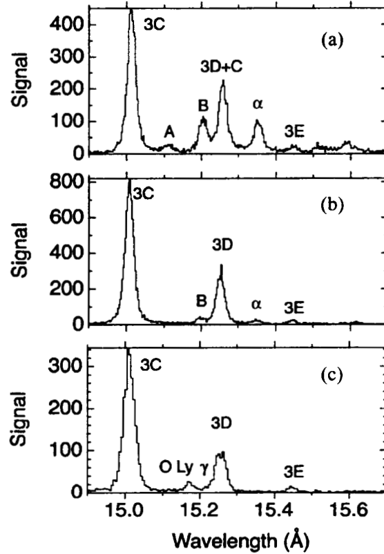
Fig. 1. Fe L-shell spectra measured for different ionization balances: (a) very low ionization balance; (b) low ionization balance (c) standard (equilibrium) ionization balance (typical for EBIT II) obtained by injection with the MeVVA. Lines 3C, 3D, and 3E are from Fe XVII. Lines A, B, and C are innershell satellites from Fe XVI, and line \alpha is an Fe XV innershell satellite. Although oxygen is a typical background gas in EBITs, O Lyman \gamma is not present in (a) and (b) because iron is continuously supplied to the trap as \text{Fe}(\text{CO})_5 and so it displaces the oxygen from the trap. However, when using a MeVVA, oxygen can accumulate because iron is only injected about once per second as in (c).
