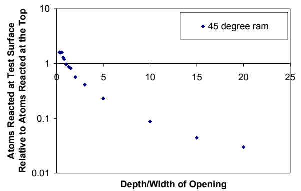
(b) Monte Carlo predictions.
