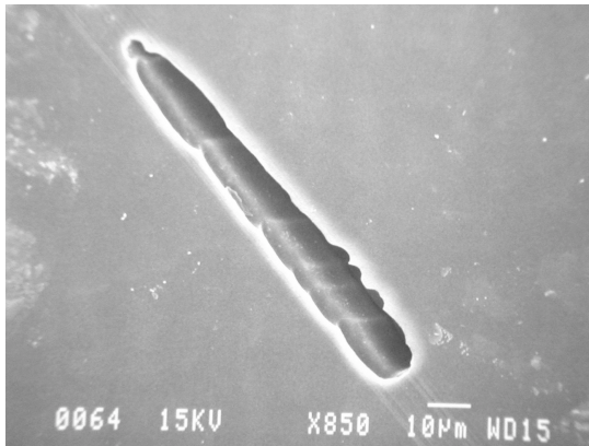
(b) Scanning electron photograph of undercut crack after removal of protective aluminum coating on Kapton.
