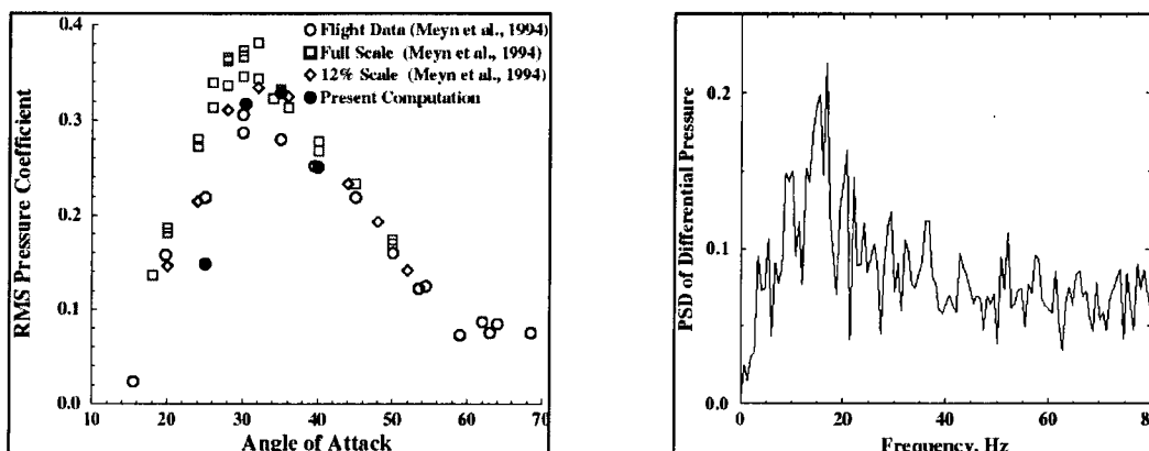
Figure 6. The RMS and PSD of differential pressure at 45% chord and 60% span point of the vertical tail.
