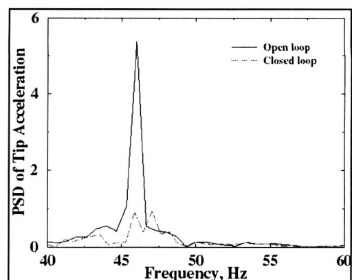
(b) PSD of tip acceleration at torsion mode
