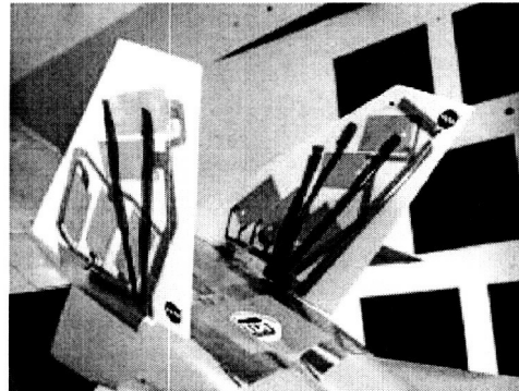
Figure 1. F/A-18 vertical tail with PZT actuators. 14
