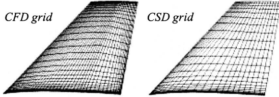
Figure 3. Surface grid of the vertical tail.
