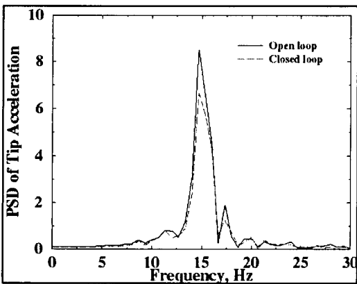
(a) PSD of tip acceleration at bending mode
