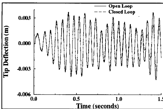
Figure 10. The time history of the tip deflection using feedback control to the root and tip PZT actuators.
