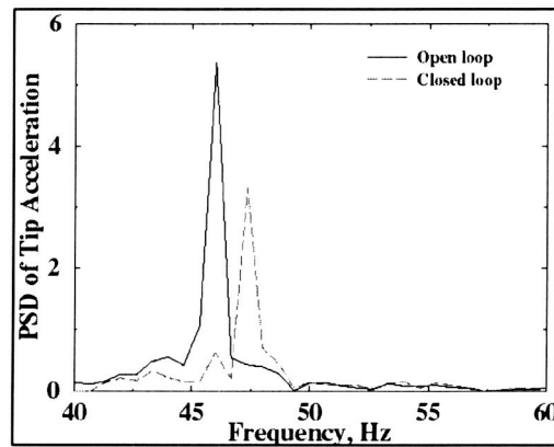
(b) PSD of tip acceleration at torsion mode.
