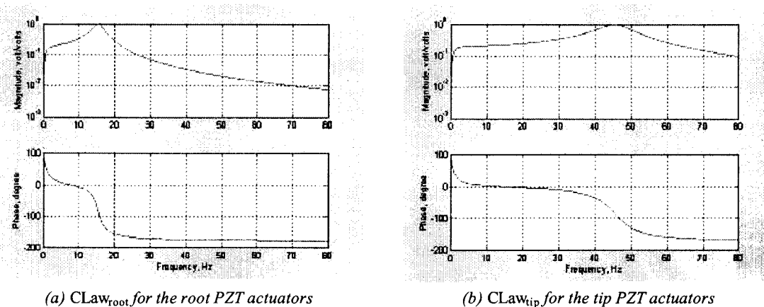
Figure 7. Frequency response of the controllers, CLaw_{root} and CLaw_{tip} .
