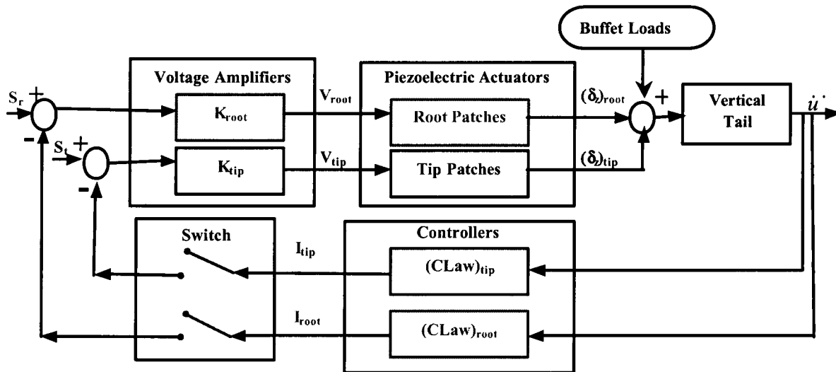
Figure 5. Active control system diagram for tail buffet alleviation.
