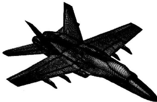
Figure 2. Surface grid of the F/A-18 aircraft.
