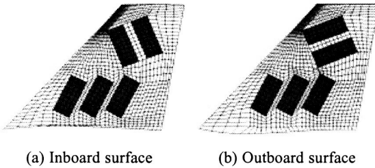
Figure 4. Aeroservoelastic model of the vertical tail
