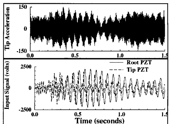
Figure 11. The time histories of tip acceleration and the input signal to the PZT actuators.
