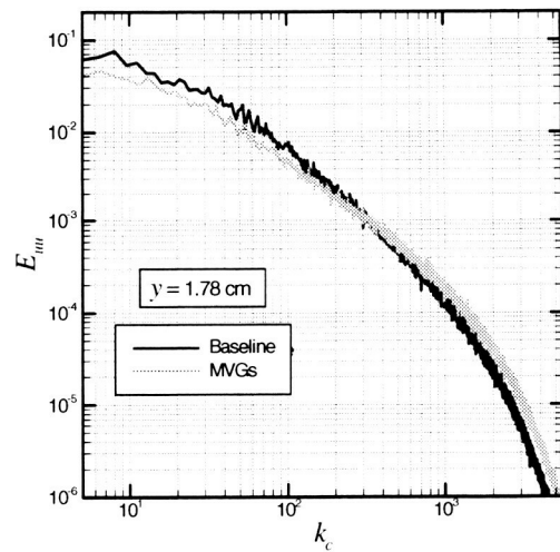
Figure 7(b). Turbulence power spectra at y = 1.78 cm.
