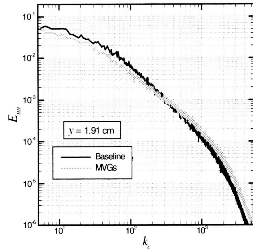
Figure 7(c). Turbulence power spectra at y = 1.91 cm.
