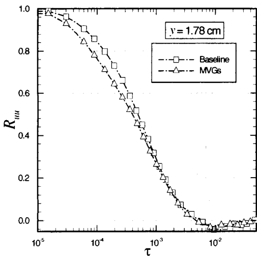
Figure 8(b). Velocity time correlations at y = 1.78 cm.
