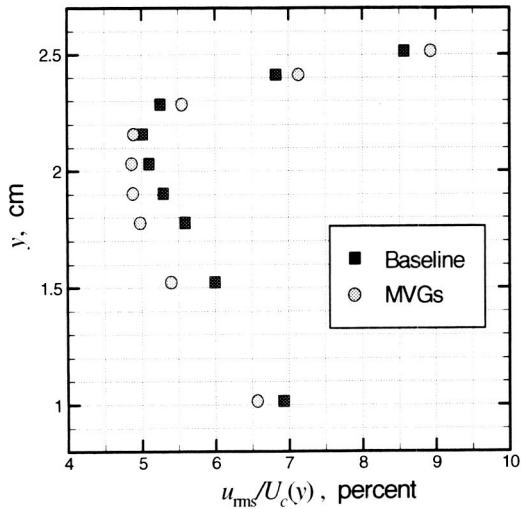
Figure 6. Local turbulence intensity at z = 0 .
