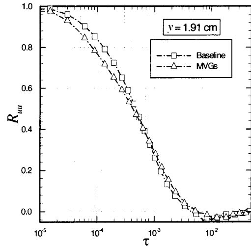
Figure 8(c). Velocity time correlations at y = 1.91 cm.
