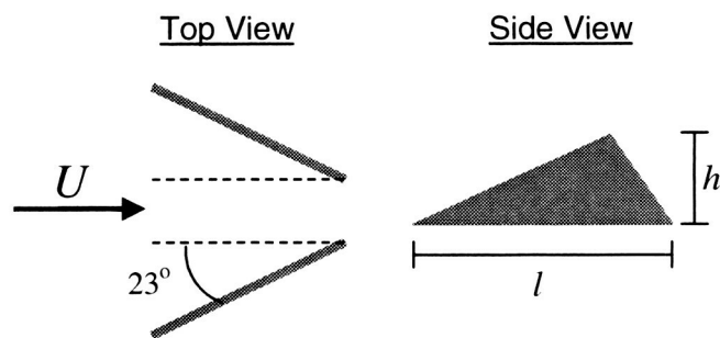
Figure 2. Delta-wing MVG geometry.
