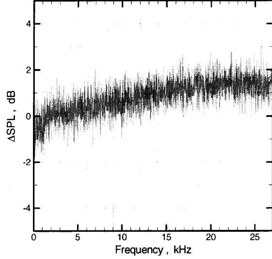
Figure 17. Difference in SPLs between the baseline flow and the flow with MVGs, as predicted by Eq. (30) with experimental input.
