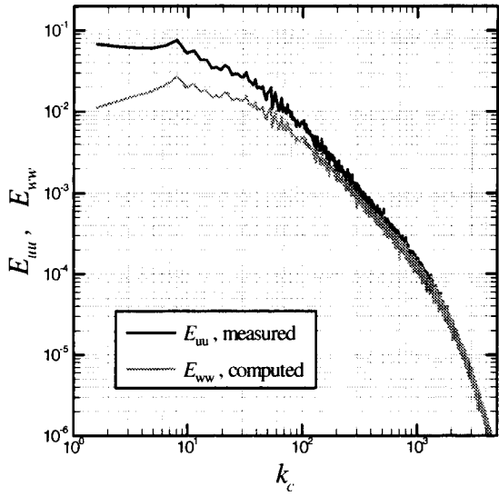
Figure 15. Measured streamwise PSD, at y = 1.78 cm; transverse PSD computed with scaling laws in Eqs. (7) and (8), and \alpha_y = 0.270 .
