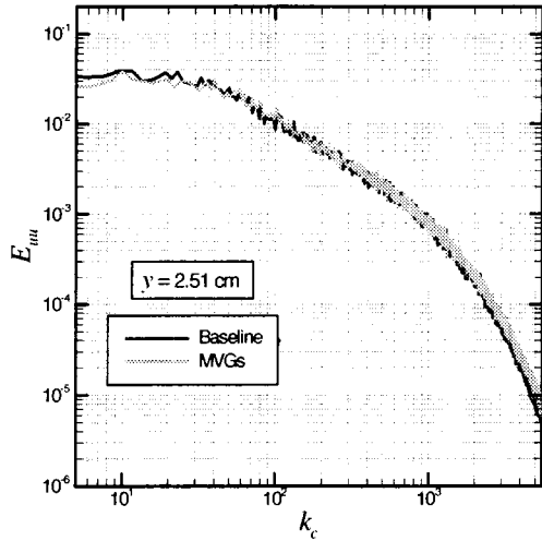
Figure 7(d). Turbulence power spectra at y = 2.51 cm
