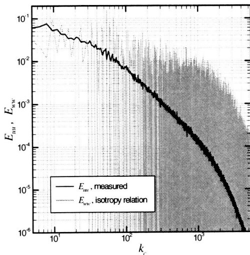
Figure 12. Streamwise spectrum as measured at y = 1.02 cm, and transverse spectrum as computed by the isotropic relation in Eq. (6).
