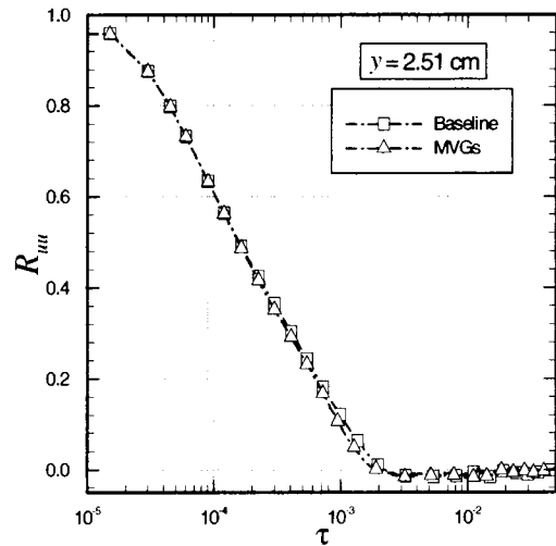
Figure 8(d). Velocity time correlations at y = 2.51 cm.
