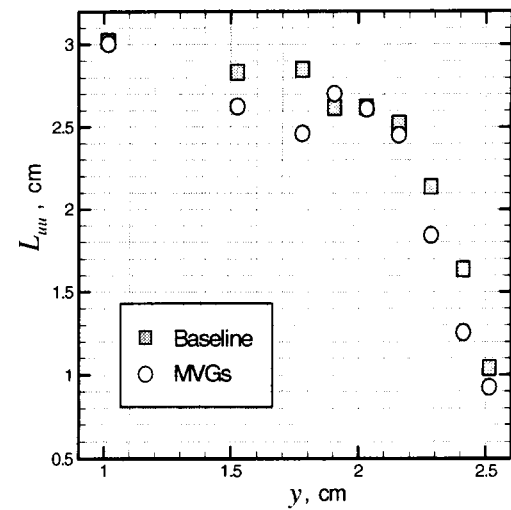
Figure 9. Streamwise integral length scales.
