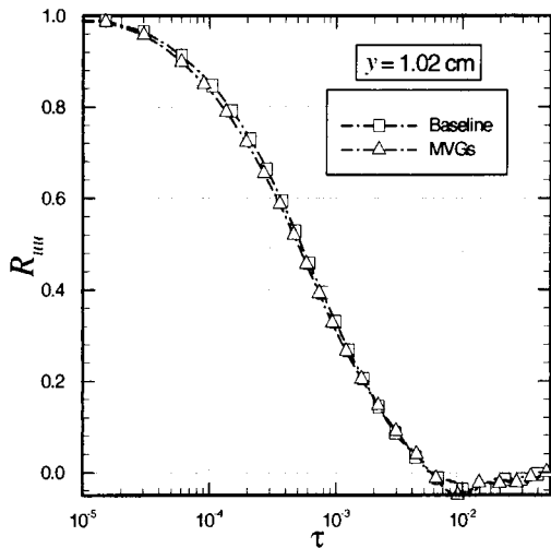
Figure 8(a). Velocity time correlations at y = 1.02 cm.
