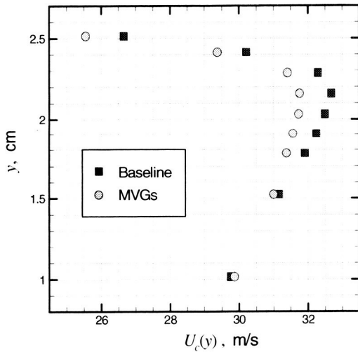
Figure 5. Mean flow at z = 0 .
