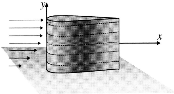
Figure 11. Strip theory schematic for stator surface pressure. Isotropy within a strip is assumed in the analysis.
