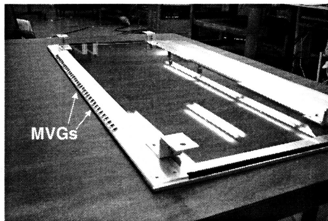
Figure 3. Underside view of nacelle model with MVGs.
