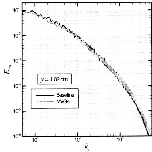
Figure 7(a). Turbulence power spectra at y = 1.02 cm.
