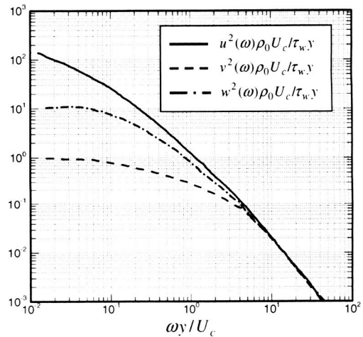
Figure 13. Streamwise, wall-normal, and transverse velocity spectra, scaled on inner variables. Data of Bradshaw and Ferriss [24], as interpreted by White [25].
