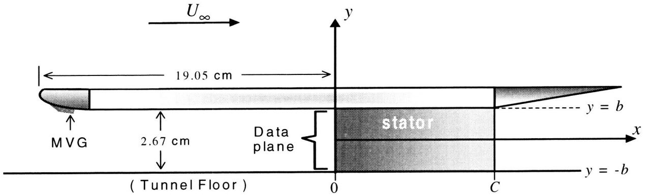
Figure 10. Placement of imaginary stator with leading edge at data measurement plane. Coordinate origin moved to stator leading edge for acoustic analysis.
