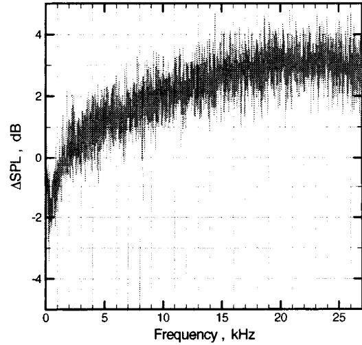
Figure 18. "Worst case" SPL differential, as predicted by Eq. (30) with experimental input only from measurement station y = 1.91 cm.
