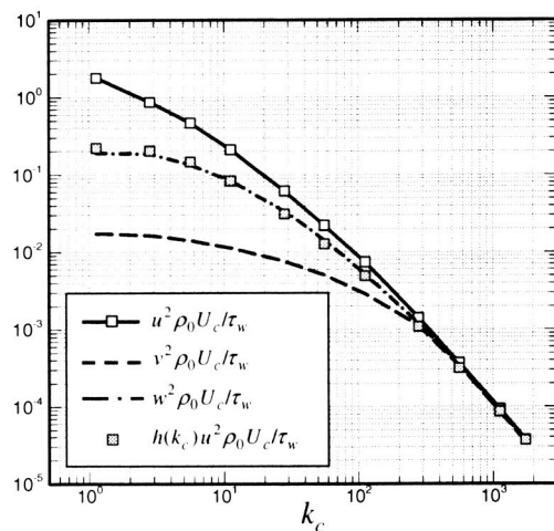
Figure 14. Scaled spectra from Fig. 13 with y = 1.78 cm and U_c = 31.91 m/s. Dark symbols are the streamwise spectrum scaled by h(k_c) in Eq. (8) with \alpha_y = 0.270 .
