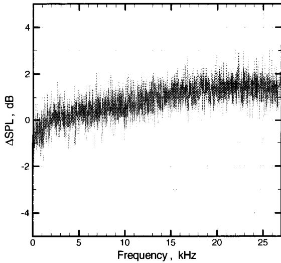
Figure 16. Difference in SPLs between the baseline flow and the flow with MVGs, as predicted by Eq. (28) with experimental input.
