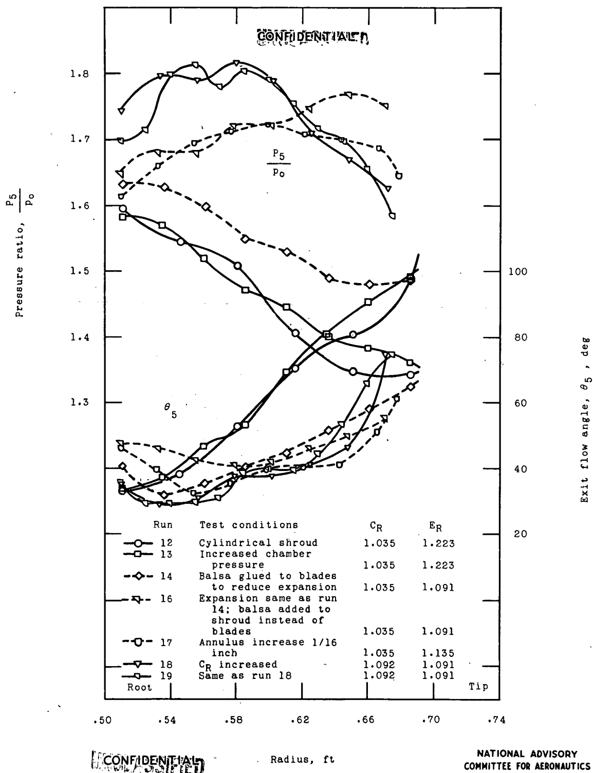
Figure 17.- Variation of total-pressure ratio and exit flow angle over rotor exit annulus for early exploratory tests. Rotational speed, 10,000 rpm.
