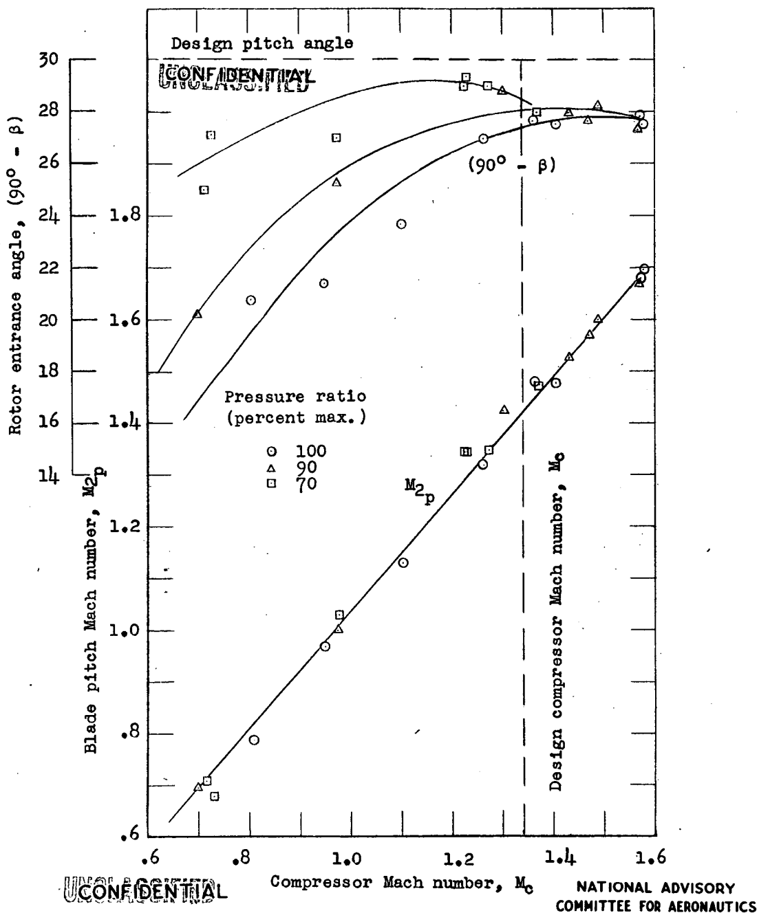
Figure 22.- Angle of flow (90^\circ - \beta) and blade pitch Mach number M_{2p} entering rotor at the pitch diameter against compressor Mach number M_c . For M_{2p} greater than about 1.53 (the design starting blade Mach number), the entrance angle is shown to be independent of throttle position as would be expected from the theory of the supersonic operating range. It is to be noted that in Freon-12, at the design value of M_c = 1.43 , the value of M_2 = 1.53 , whereas in air M_2 = 1.62 . (See appendix D.)
