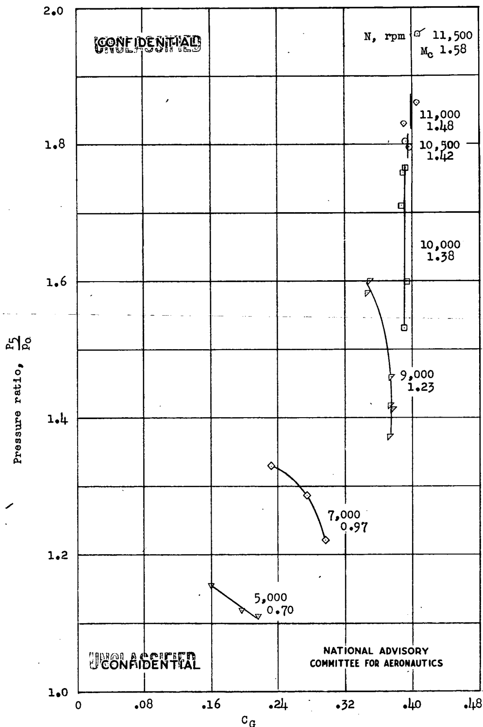
Figure 19.- Variation of mass-flow coefficient C_G with throttling and compressor Mach number. These data were obtained from surveys behind the rotor and therefore do not include any stator losses. (Flagged symbols represent 12-point survey test.)
