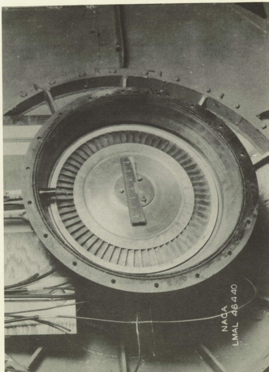
Figure 13.- Downstream view of the rotor showing the survey-instrument location and the balsa-wood inserts beneath the shroud. The cylindrical surfaces which form the aerodynamic passages following the rotor have been removed.
