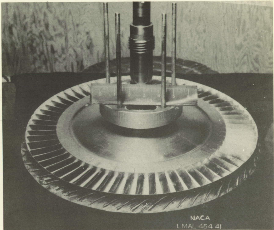
Figure 16.- Supersonic-compressor rotor and shaft. Lacquered balsa-wood inserts are shown on the rearward side of each blade. The blade-tip curvature may be seen on the outside of the shroud. The curvature is completely washed out at the blade pitch sections.
