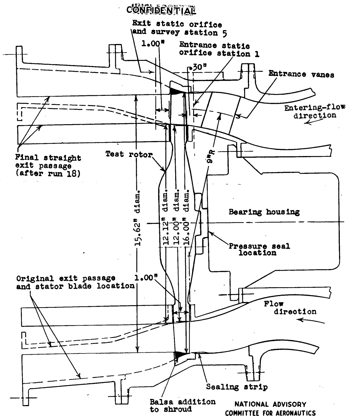
Figure 1.- Longitudinal section through the rotor showing aerodynamic passages. The original outward curvature of the shroud and exit passage are shown as dashed lines.
