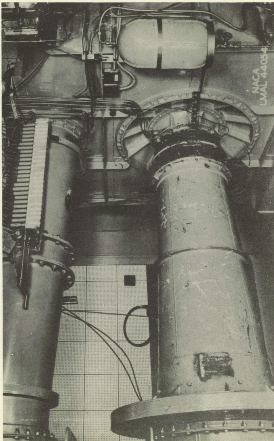
Figure 12.- Supersonic-compressor test setup. The throttling-valve lever and protractor are visible on the upper return section. The velocity-of-sound meter for determining the composition of the test fluid is shown at the upper right.
