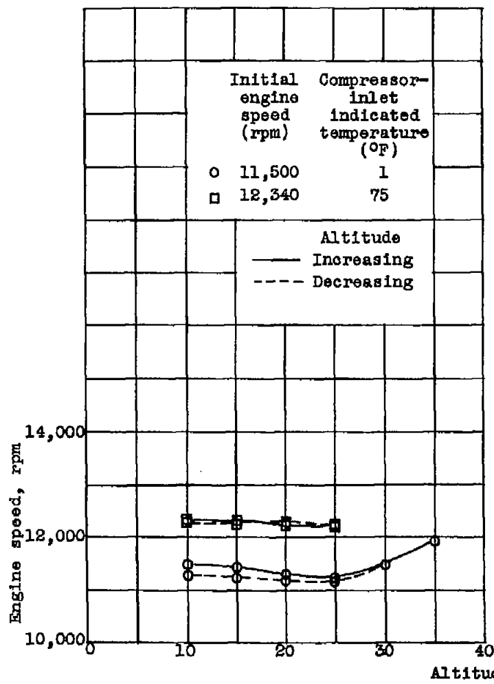
Figure 15. - Concluded. Effect of altitude on engine speed and fuel flow of modified engine with engine governor at constant throttle position.
