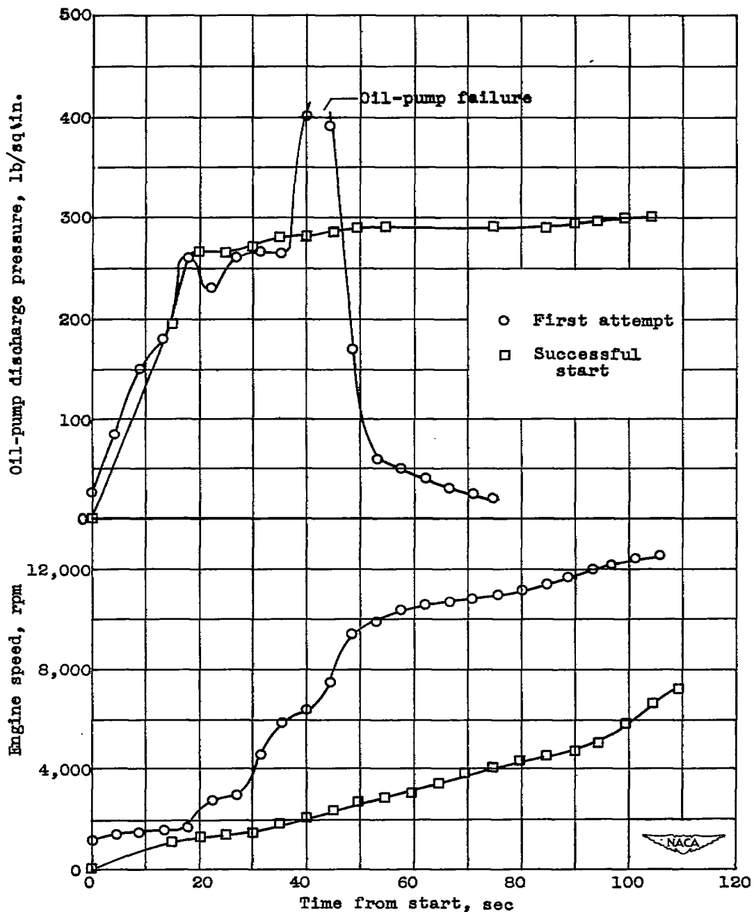
Figure 18. - Comparison of engine speed and oil-pump discharge pressure during two starts made at ambient-air temperature of -50^{\circ} F with static flight conditions at altitude of 2000 feet. Modified engine with special fuel-control system.
