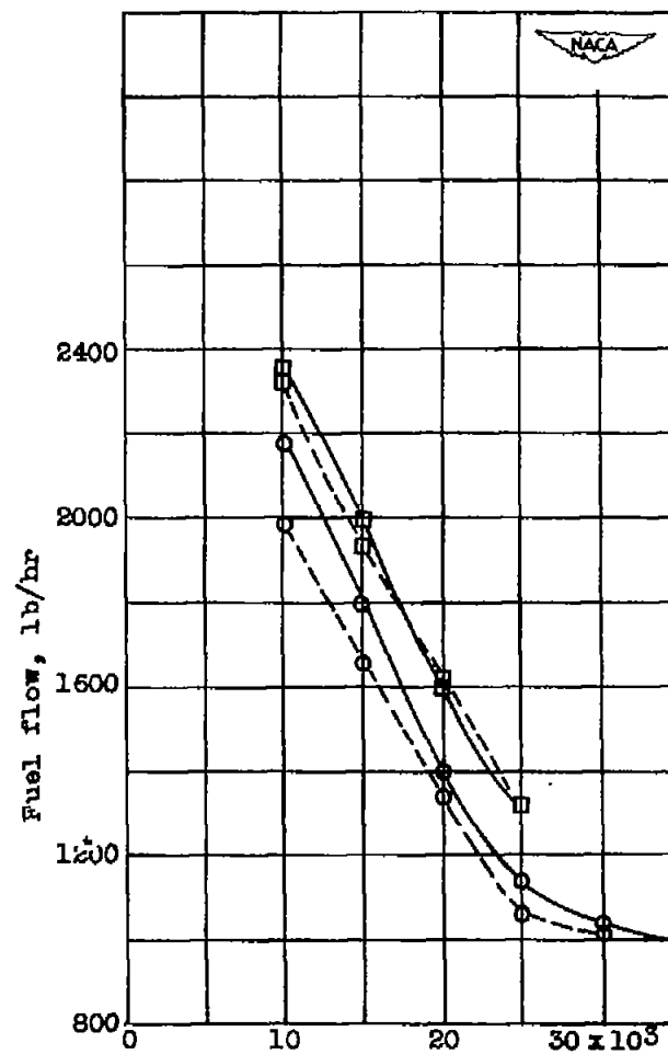
Figure 15. - Concluded. Effect of altitude on engine speed and fuel flow of modified engine with engine governor at constant throttle position.
