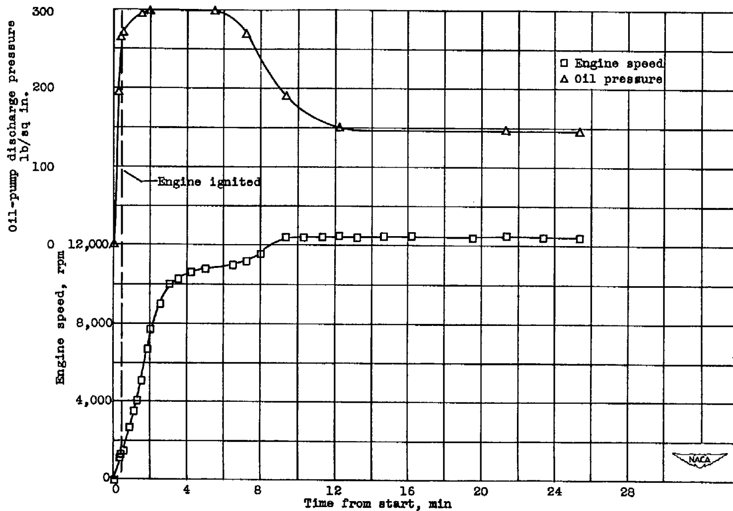
(a) Engine speed and oil-pump discharge pressure. Figure 19. - Variation of engine speed, oil-pump discharge pressure, and bearing temperatures with time during successful start at ambient-air temperature of -50^{\circ} F with static flight conditions at altitude of 2000 feet. Modified engine with special fuel-control system.
