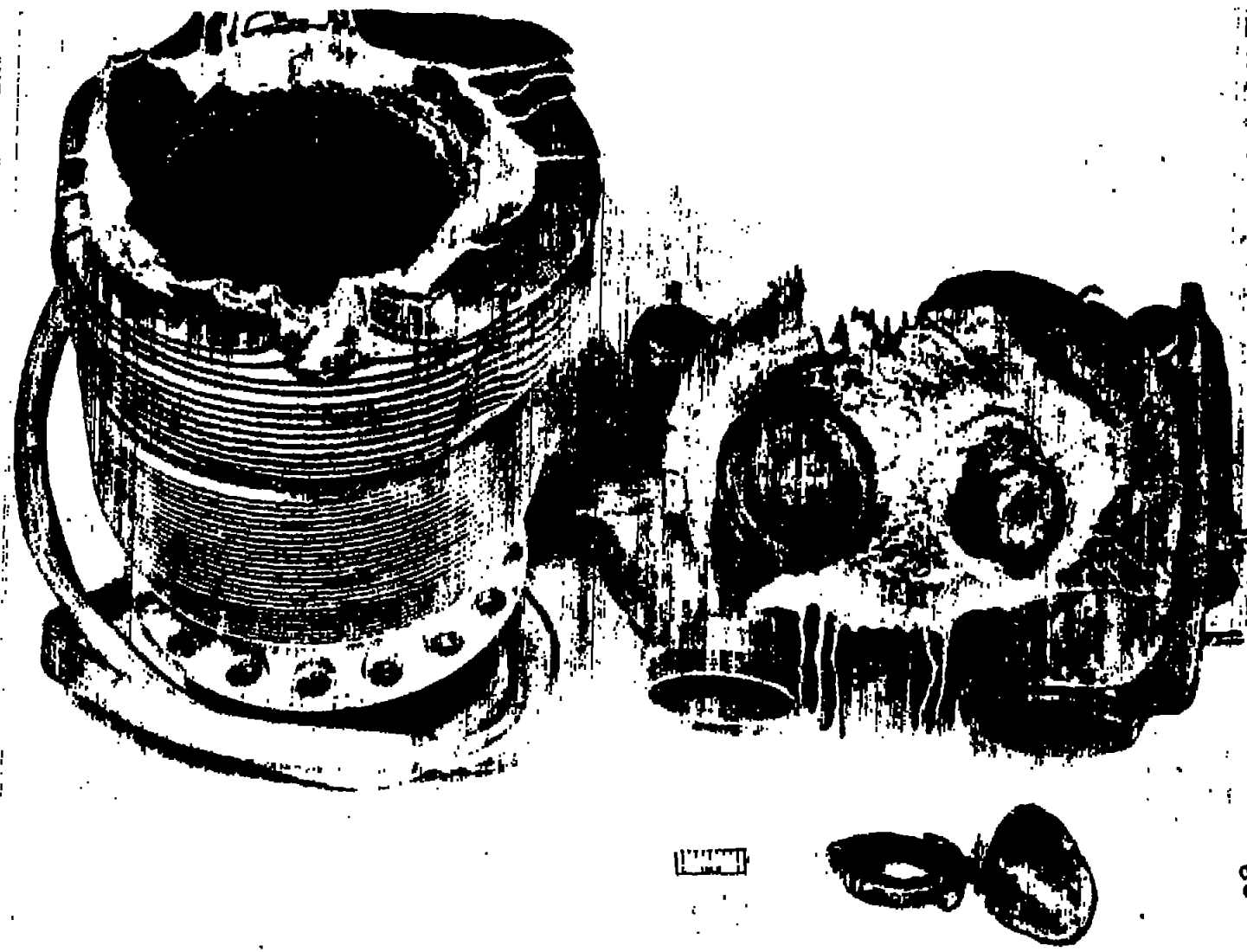
Figure 2. - Damaged cylinder resulting from exhaust-valve fracture. Rear-park-plug-gasket temperature, 550° F; engine speed, 2600 rpm.
