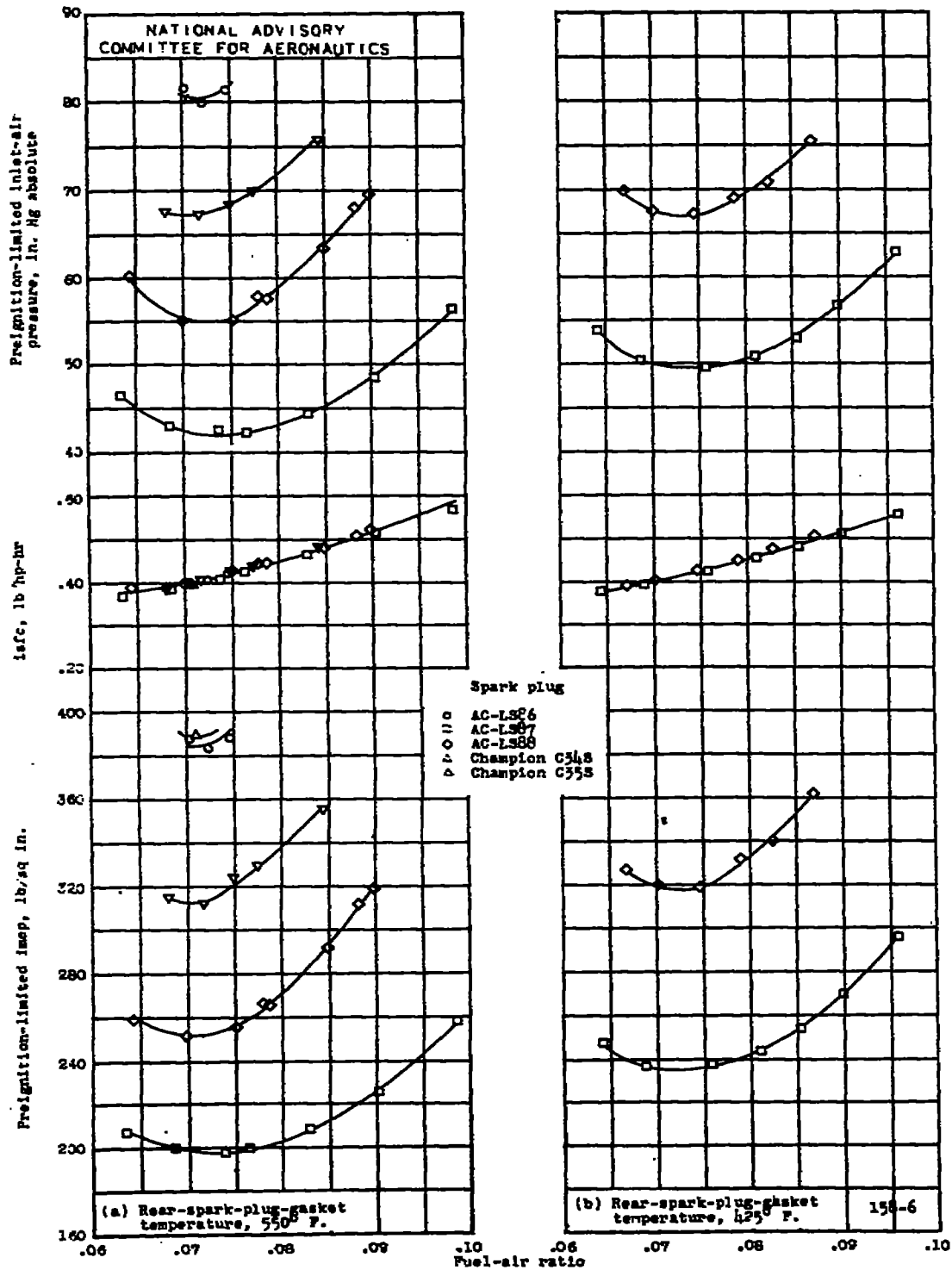
Figure 7. - Preignition-limited performance of R-2800 cylinder using five types of spark plug. Fuel, triptane + 4.0 ml TEL per gallon; compression ratio, 6.78; spark advance, 20° B.T.C.; engine speed, 2600 rpm; inlet-air temperature, 280° F.
