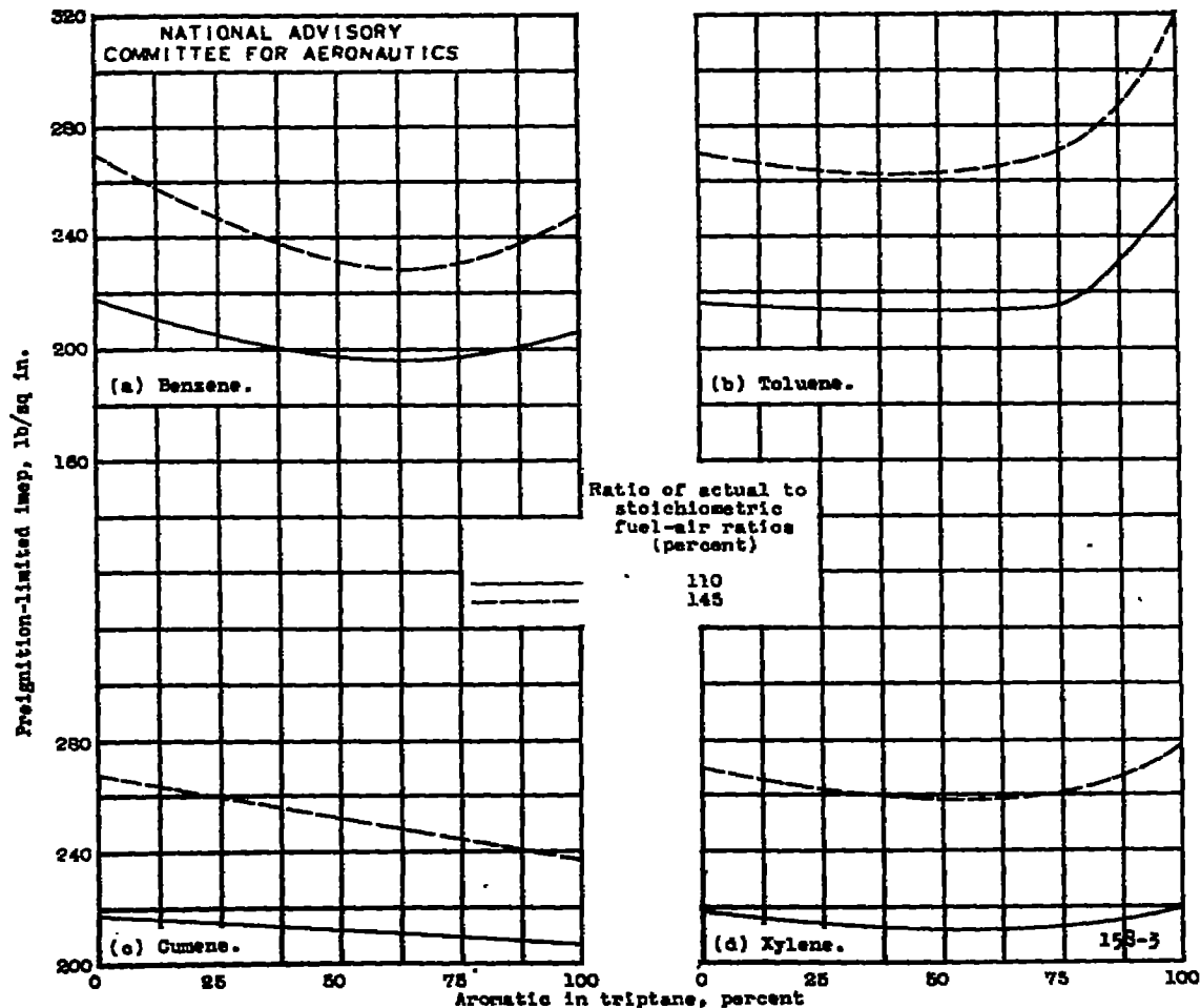
Figure 4. - Effect of aromatic content on preignition-limited indicated mean effective pressure at two mixture strengths. All fuels contain 4.0 ml TEL per gallon. R-2800 cylinder; compression ratio, 8.75; spark advance, 20° B.T.C.; engine speed, 2600 rpm; inlet-air temperature, 260° F; rear-spark-plug-gasket temperature, 425° F.
