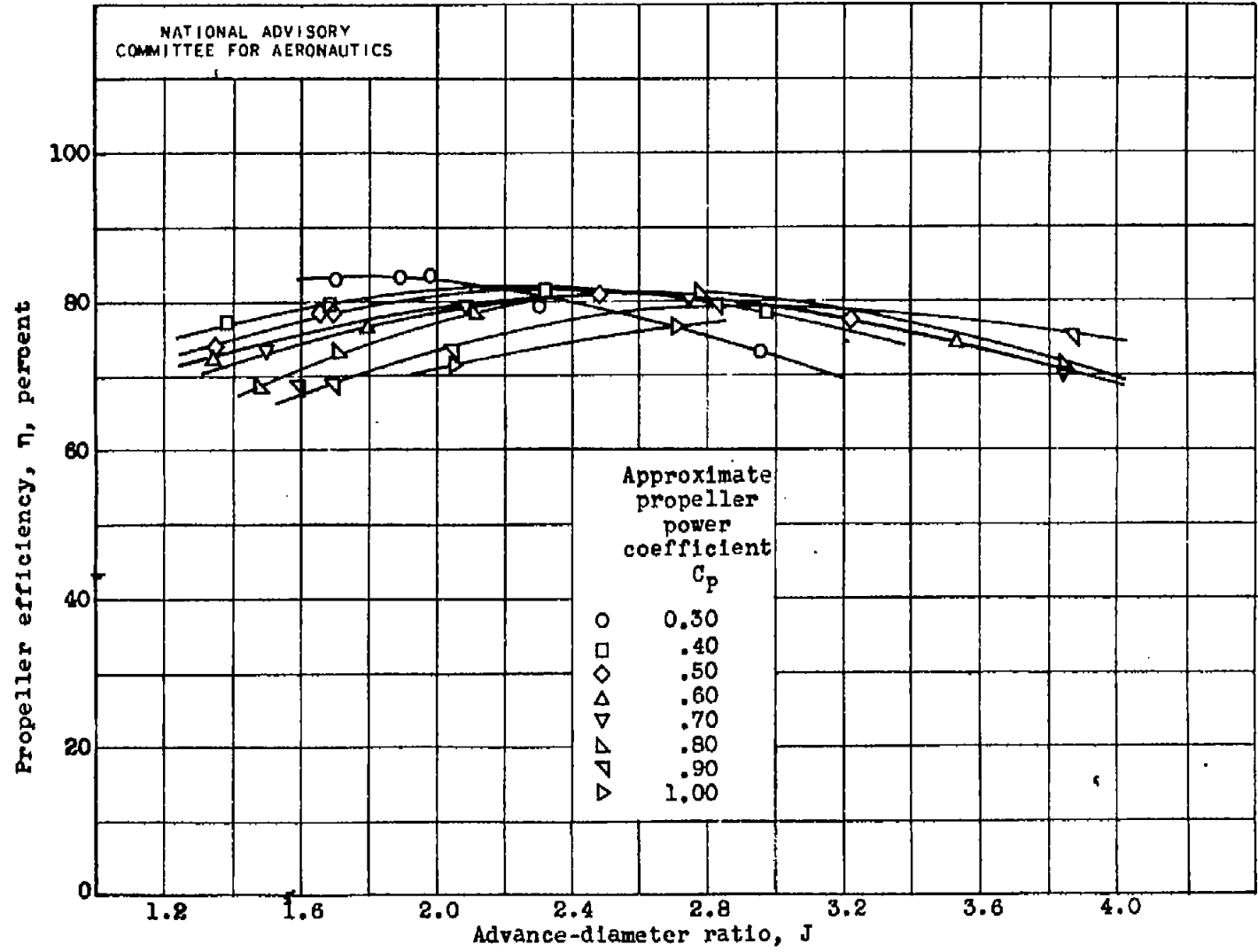
Figure 4.- Characteristics of Curtiss 732-1C2-0 four-blade propeller on YP-47M airplane at free-stream Mach number M_o of approximately 0.40.
