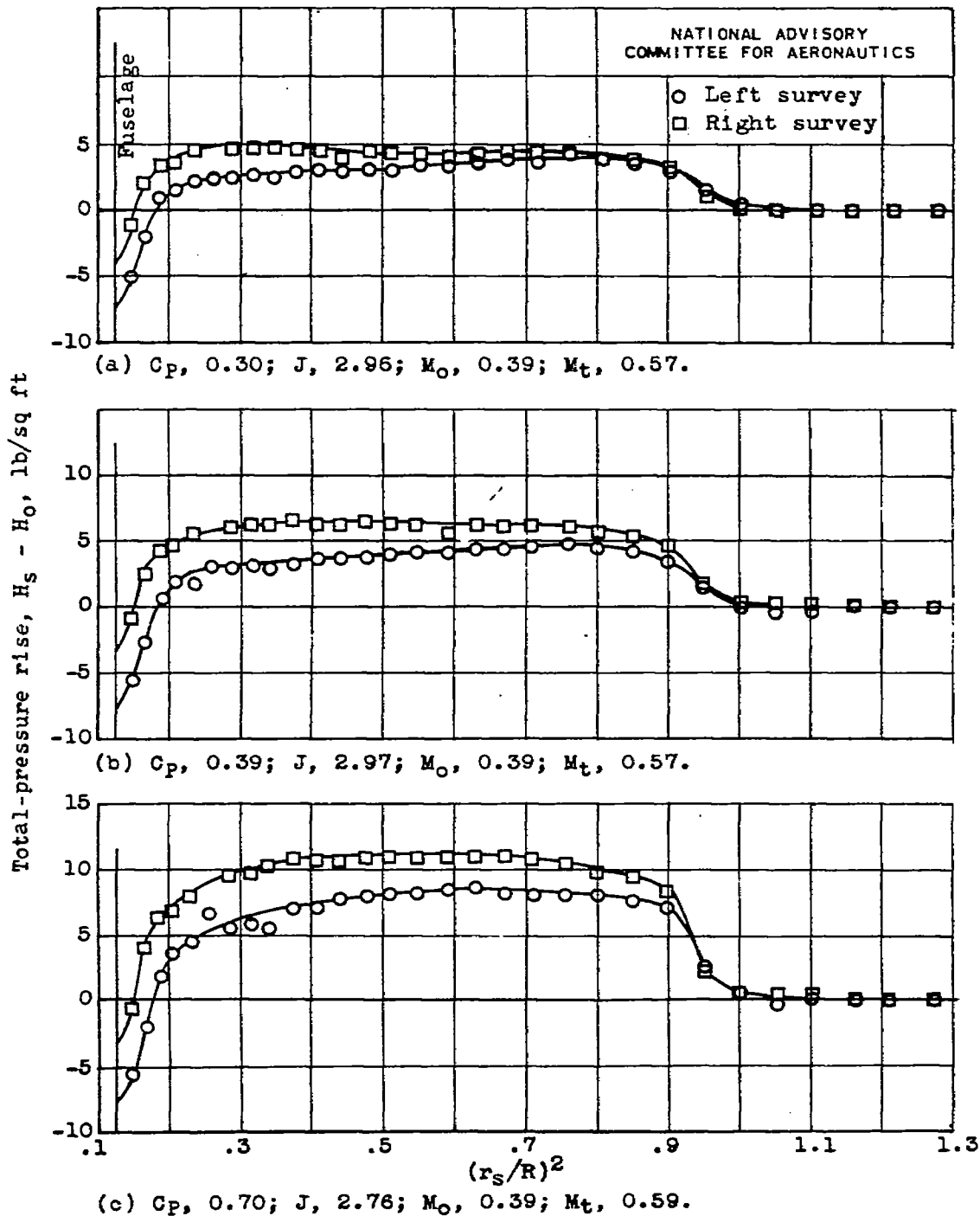
Figure 7.- Effect of power coefficient C_p on blade thrust load distribution at advance-diameter ratio J of approximately 2.80 and free-stream Mach number M_o of approximately 0.40. Curtiss 732-1C2-0 four-blade propeller.
