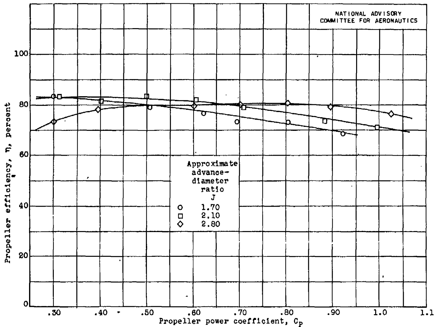
Figure 5.- Effect of power coefficient C_p on efficiency \eta of Curtiss 732-1C2-0 four-blade propeller at free-stream Mach number M_o of approximately 0.40.
