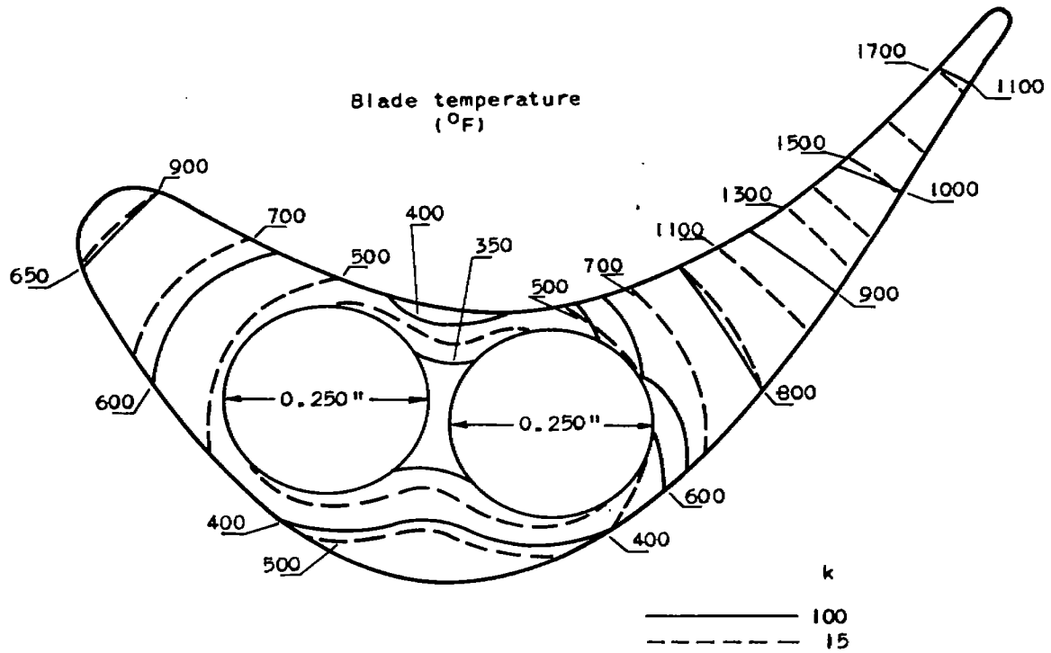
Figure 4. - Effect of variation of thermal conductivity k on temperature distribution through water-cooled turbine blade. Hot-gas-to-metal heat-transfer coefficient q_i , 217 Btu/(hr)(sq ft)(°F); effective gas temperature T_e , 2000° F; average water temperature T_w , 200° F.
