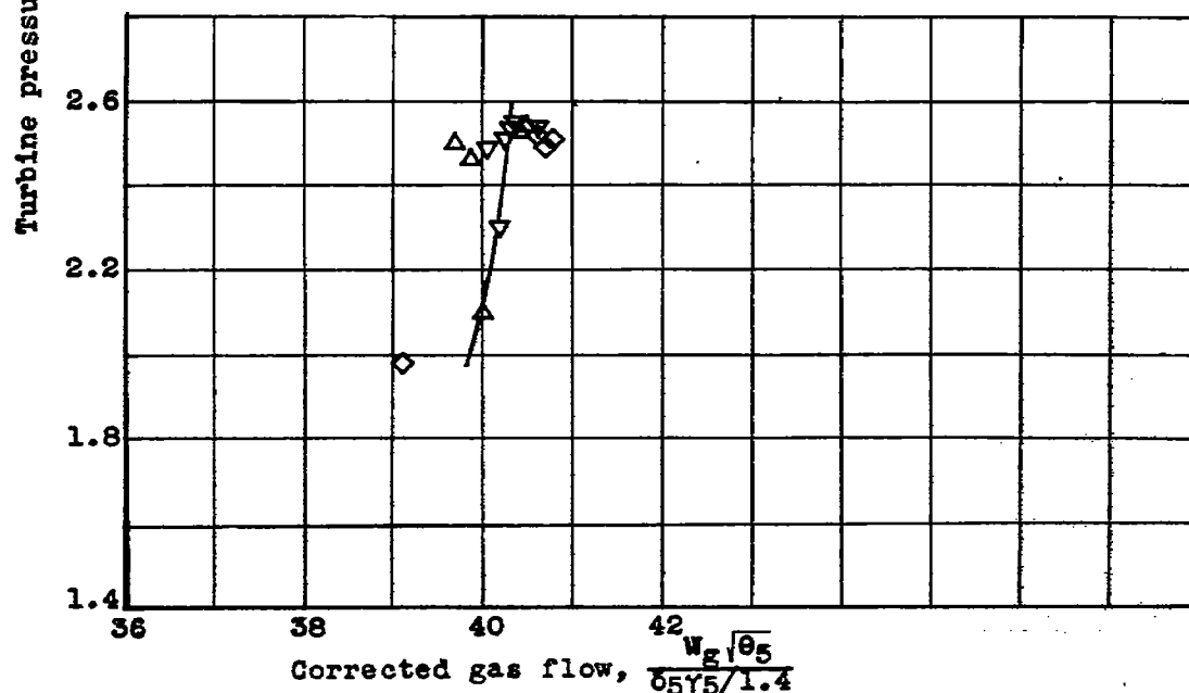
Figure 6.- Operating characteristics of turbine with large turbine nozzle, high-flow compressor, and 19 \frac{1}{2} -inch tail-pipe nozzle at ram-pressure ratio of 1.42. Turbine speed and gas flow corrected to NACA standard atmospheric conditions at sea level.
