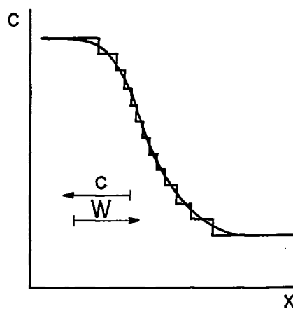
Figure 7.- Wave of finite amplitude.
