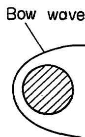
Figure 1.- Bow wave for high Mach number.
