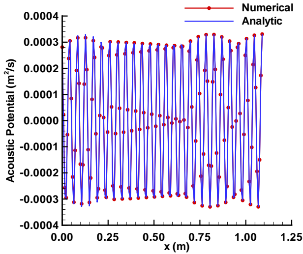
Figure 8 Real Part of Acoustic Potential - Upstream Propagation [ r = 0.308 m, \theta = 0 , M = 0.4 , 5000 Hz, (10, 1) mode].
