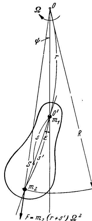
Figure 15.- Material pendulum.
