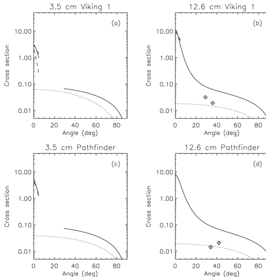
Figure 1. Radar scattering properties of the Viking 1, panels (a) and (b), and Mars Pathfinder landing sites, panels (c) and (d). Solid lines are OC polarization and dotted lines are SC polarization. The left-hand panels are for X-band and show GSSR quasi-specular delay-Doppler Hagfors model fits and G-VLA diffuse scattering cosine model fits. The dashed lines show the range of values from the GSSR fits. The right-hand panels are for S-band and show the Moore and Thompson [1] OC and SC scattering models for the units in which the MER landing ellipses are located. The points at \square \sim 30^\circ are SC cross section determinations by [2]. The Viking 1 dashed line data are (also) from [2].
