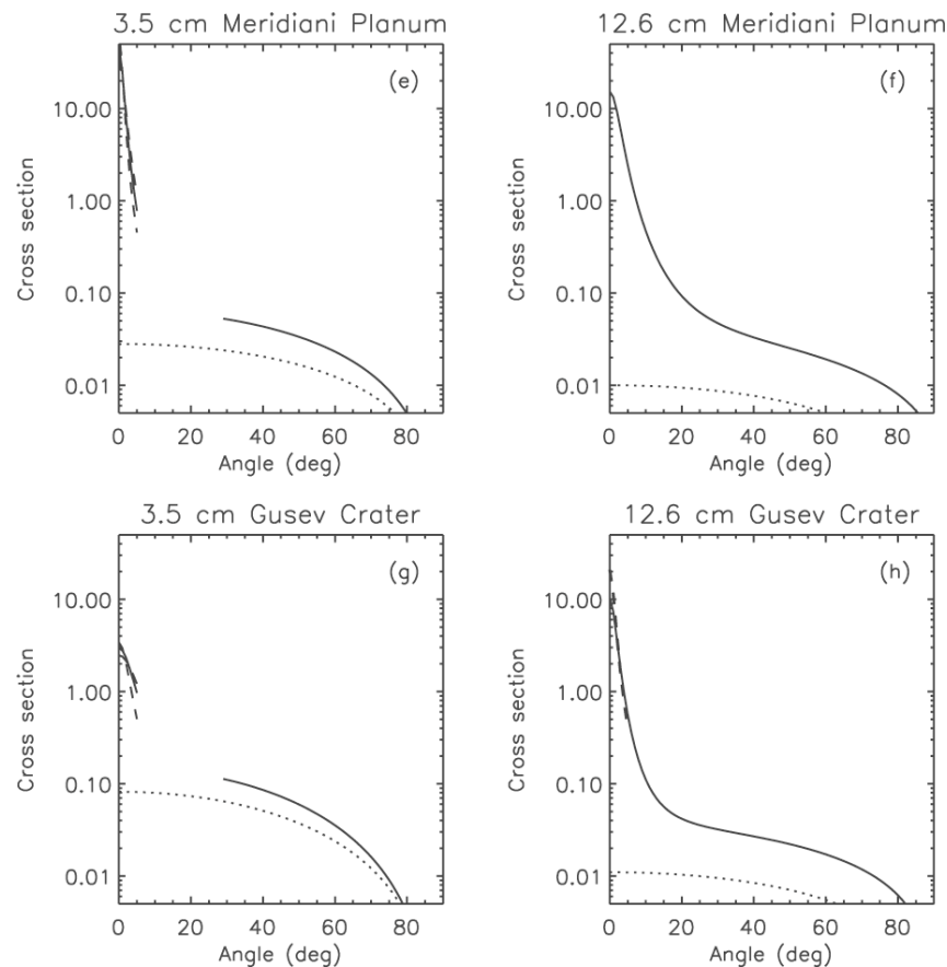
Figure 1. con't. Radar scattering properties of the Meridiani Planum, panels (e) and (f), and Gusev Crater, panels (g) and (h), MER landing sites. Solid lines are OC polarization and dotted lines are SC polarization. The left-hand panels are for X-band and show GSSR quasi-specular delay-Doppler Hagfors model fits and G-VLA diffuse scattering cosine model fits. The dashed lines show the range of values from the GSSR fits. The X-band GSSR data at Gusev crater are for the same geologic unit as the crater, but are not inside the crater. The right-hand panels are for S-band and show the Moore and Thompson [1] OC and SC scattering models for the units in which the MER landing ellipses are located. The dashed line quasi-specular data for Gusev crater is from GSSR [4].
