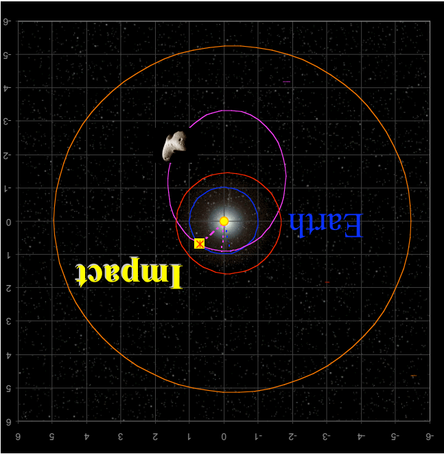
Figure 12 – M1999JT6 Orbit Plot
