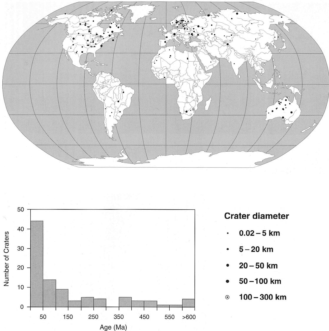
Figure 2 – Location of known impact craters noting diameters as of 1998. Age distribution of these craters is also included. 2
