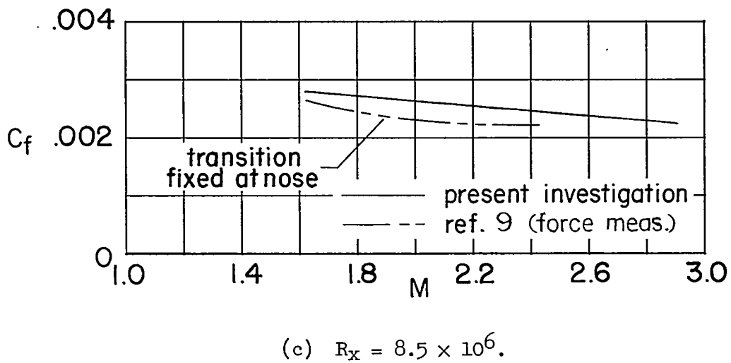
Figure 11.- Extension of present data compared with tunnel measurements.
