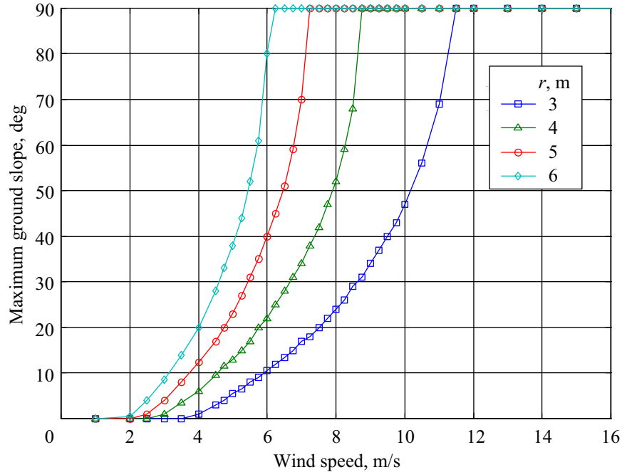
Figure 15. Maximum slope versus wind speed ( m = 10 kg, C_D = 1.0 , \mu_r = 0.1 ).
