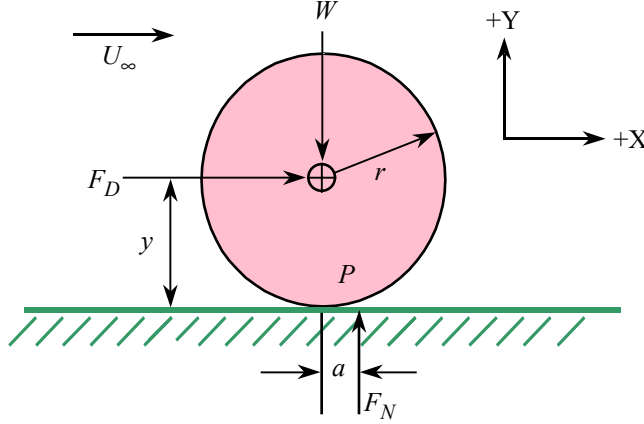
Figure 3. Forces acting on a Mars Tumbleweed.
