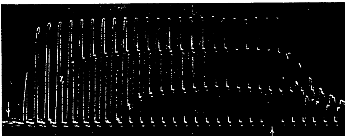
Figure X. - Photorecord of three transverse thermocouples in nonstationary regime. Arrows indicate instants of switching heater on and off. Duration of cycle of switching of galvanometer (distance between time marks) is equal to 7.5 \times 4 = 30 seconds. Model axis is inclined 45^\circ to vertical.
