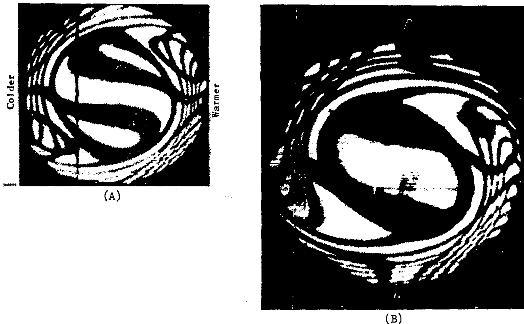
Figure 45. - Convection in cylindrical horizontal channel observed by lattice method: A, Heating from right, cooling from left; vertical line is plumb line. B, heating from right down, cooling from left up. Two pairs of mutually embracing isolines belong with isolines of equal vertical gradients. Isolines forming closed ovals in center belong with isolines of equal horizontal gradients.
