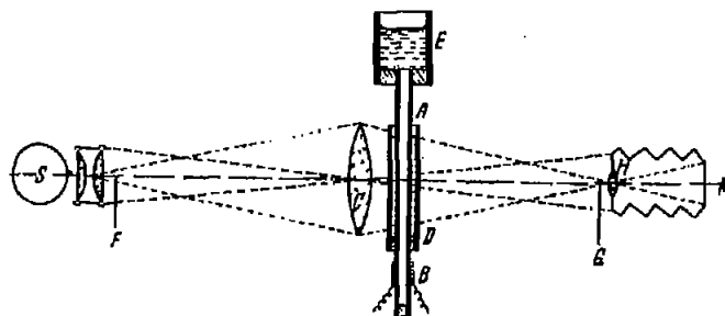
Figure 42. - Optical method of vertical deflections: S, Light source; C, large objective; H, photo objective; k, ground glass or graphic plate; F and G, horizontal knife edges; A, glass tube of model; D, prismatic vessel; B, heater; E, cold reservoir.
