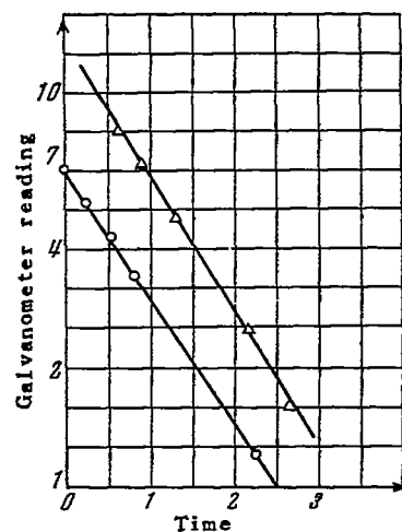
Figure 29. - Linear dependence of logarithm of steady temperature on time convective process takes to reach corresponding thermocouple.
