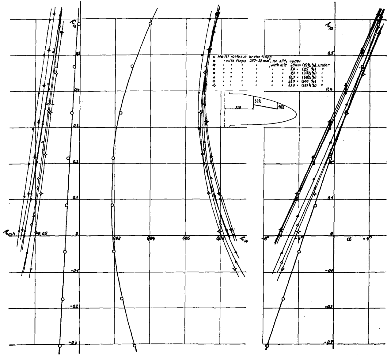
Figure 9.- Larger brakes with gap.
