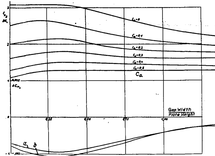
Figure 8.- Braking effect, change of zero lift direction and of diving moment with various gap widths. (to Fig. 7)
