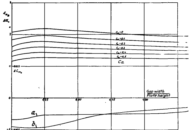
Figure 10.- Braking effect - change in zero lift direction and diving moment. (to Fig. 8)
