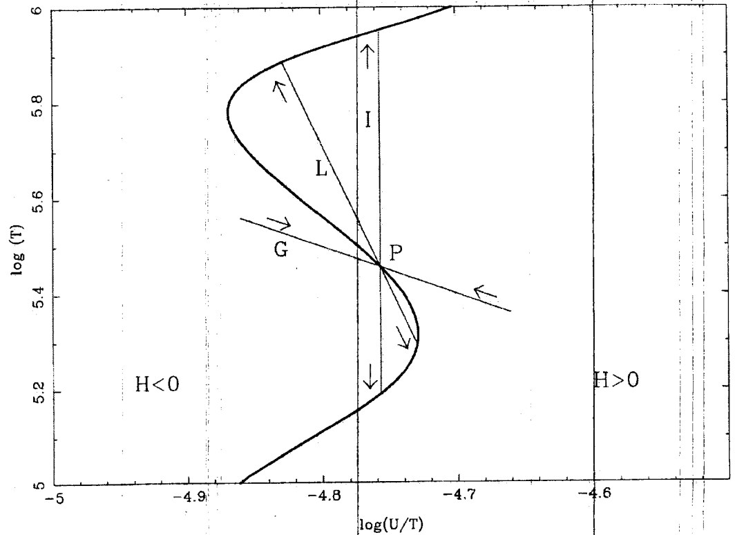
Figure 5: Schematic depiction of an unstable (to isobaric perturbations) portion of an S curve (from Bottorff, Korista, & Shlosman 2000). The region marked H < 0 or H > 0 are those where the cooling rate in the gas is greater than or less than the heating rate. Different perturbation paths (marked G, L, and I) are shown crossing the point P. Arrows show the direction gas will evolve along a constraint when perturbed off the point P. Path I corresponds to a thermally unstable isobaric perturbation. Path L has a slope less than the S curve at point P, hence perturbations constrained on this path are unstable. Path G has a slope greater than the S curve at P, hence perturbations constrained to this path are stable.
