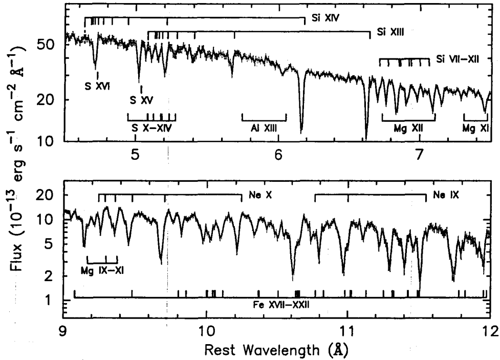
Figure 2: Two parts of the CXO /HEG+MEG spectrum of NGC 3783 (adapted from Kaspi et al. 2002). The upper panel shows the region containing lines due to K -shell transitions in Si. For each, the locations in the rest frame of the galaxy of the first nine lines in the He- and H-like K -shell series are marked (ie. n = 1 \rightarrow 2, 3 \dots from right to left), along with the bound/free edges. Many of these lines are clearly detected, as are several lines from less-ionized Si, and various Mg, Al and S ions. The lower panel shows several He- and H-like lines of Ne detected within a forest of lines due to various ionization states of Fe (see Kaspi et al. 2002 for details).
