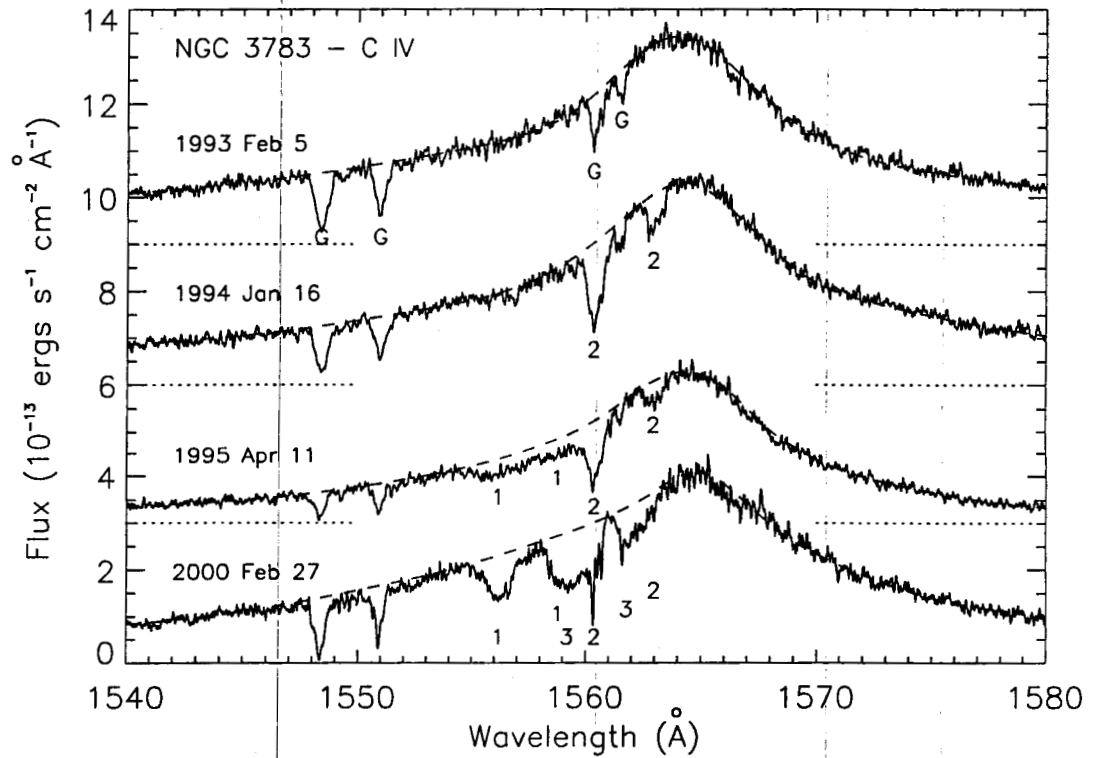
Figure 7: GHRM (top three plots) and STIS spectra (bottom plot) of the C IV region in NGC 3783. The zero flux levels are given by dotted lines. Galactic absorption lines (from C IV and C I) are indicated with a "G", and the three kinematic components of the intrinsic C IV doublet are numbered.
