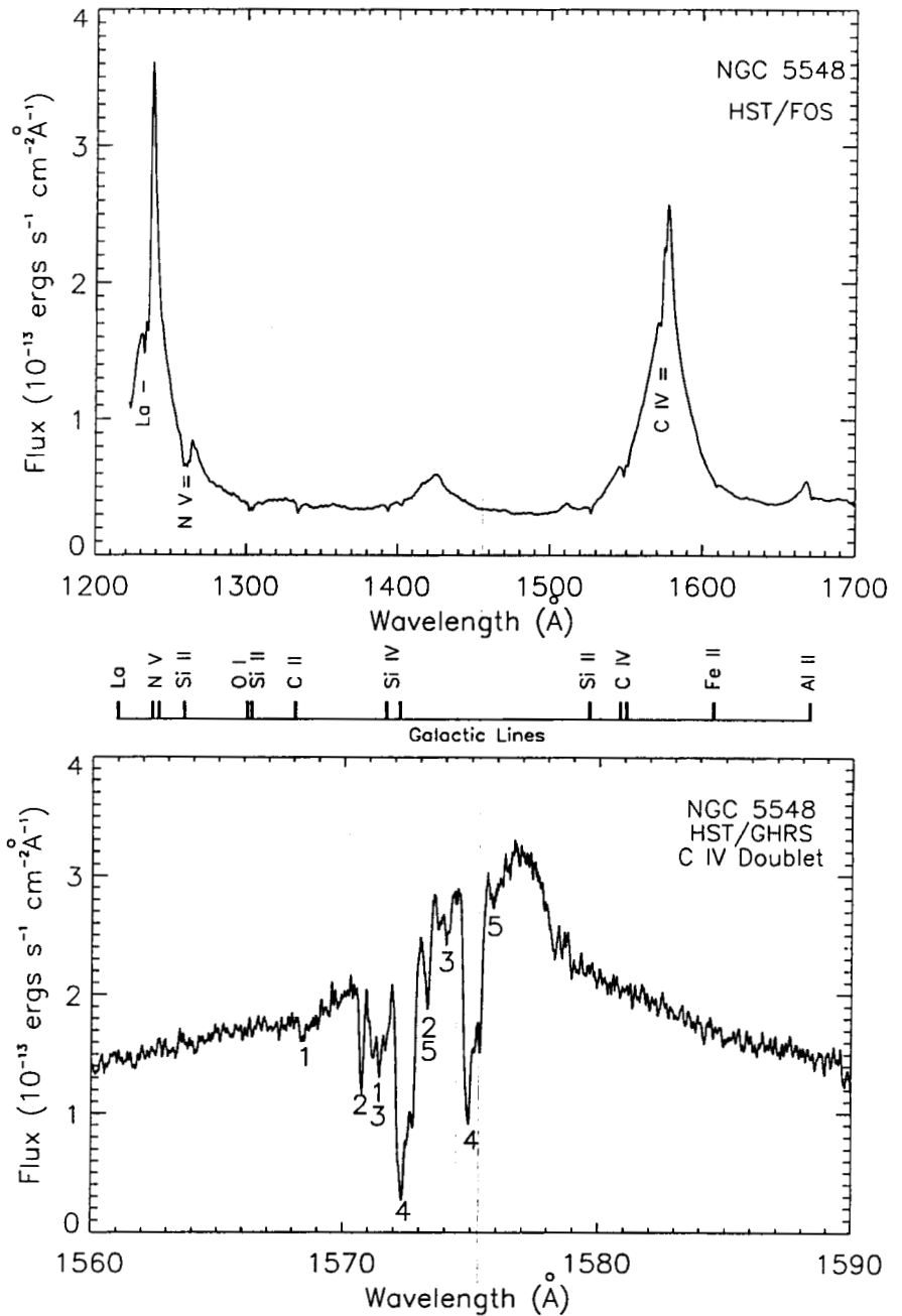
Figure 1: HST spectra of the Seyfert 1 galaxy NGC 5548. The top panel shows a spectrum from the FOS, and indicates the positions of intrinsic UV absorption by H I L\alpha , and the C IV and N V doublets. The middle panel shows the locations of interstellar absorption lines in the top panel due to our Galaxy. The bottom panel shows a high-resolution spectrum in the C IV region from the GHRS, and identifies five kinematic components of absorption in the C IV doublet.
