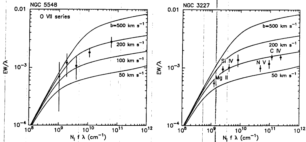
Figure 4: Left panel: Curves of growth based on the equivalent widths of O VII absorption lines in the CXO spectrum of NGC 5548 (Kaastra et al. 2002). A good match is obtained for N(\text{O VII}) = 4.0 (\pm 1.5) \times 10^{17} \text{ cm}^{-2} and b = 200 (\pm 50) \text{ km s}^{-1} . Right panel: Curves of growth based on the equivalent widths of absorption lines in NGC 3227 and predicted column densities from the photoionization models in Crenshaw et al. (2001). The EW s of the absorption lines are consistent with the models for a b value of 100 \pm 50 \text{ km s}^{-1} .
