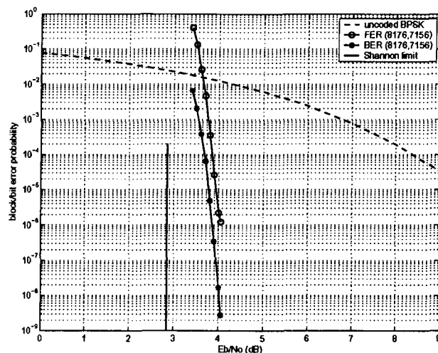
Fig. 6. EG-LDPC (8176, 7156) Iterative Convergence
