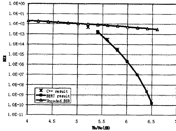
Fig. 4. Majority Logic Decoding Testing at 400 Mbps
