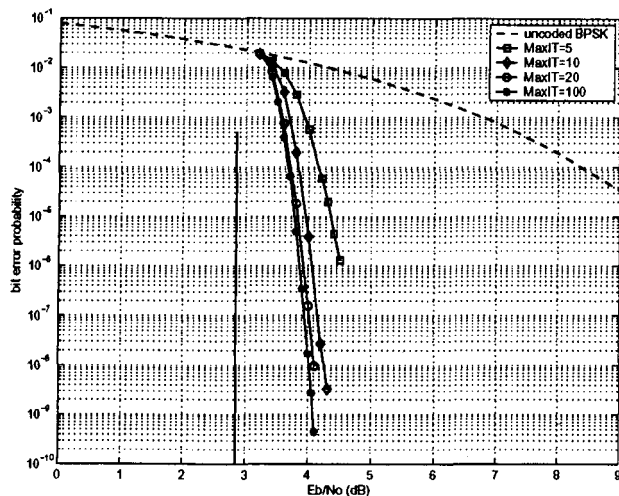
Fig. 5. EG-LDPC (8176, 7156) BER and FER Performance.
