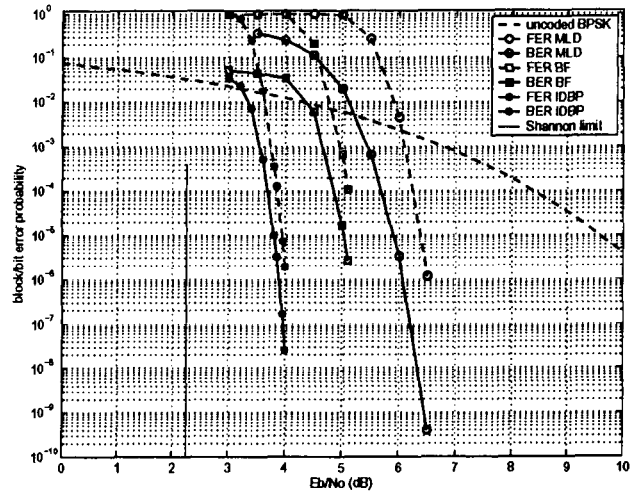
Fig. 2. EG-LDPC (4095, 3367) BER and FER Performance
