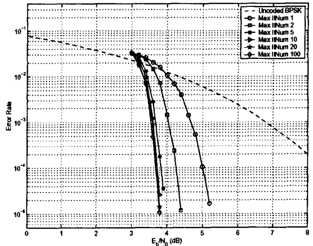
Fig. 3. EG-LDPC (4095, 3367) Iterative Convergence
