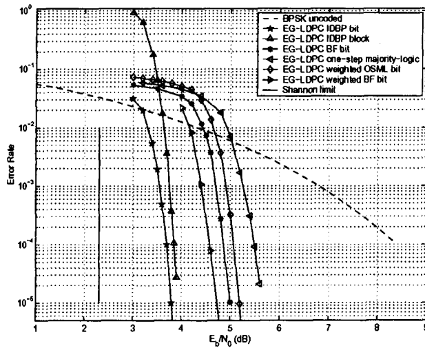
Fig. 1. EG-LDPC (4095, 3367) BER Performance with Various Decoding Options
