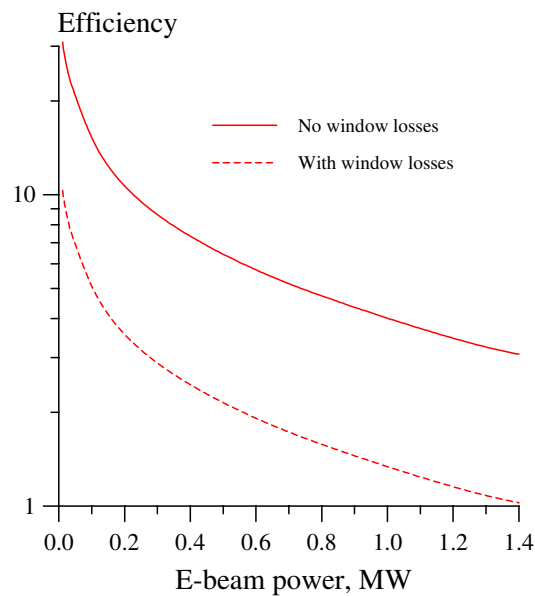
Figure 10.—Generator efficiency as a function of the absorbed e-beam power, with and without window losses. Faraday accelerator, K = 0.5
