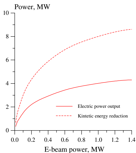
Figure 11.—Extracted electrical power and kinetic energy reduction as functions of the absorbed e-beam power. Faraday accelerator, K = 0.5
