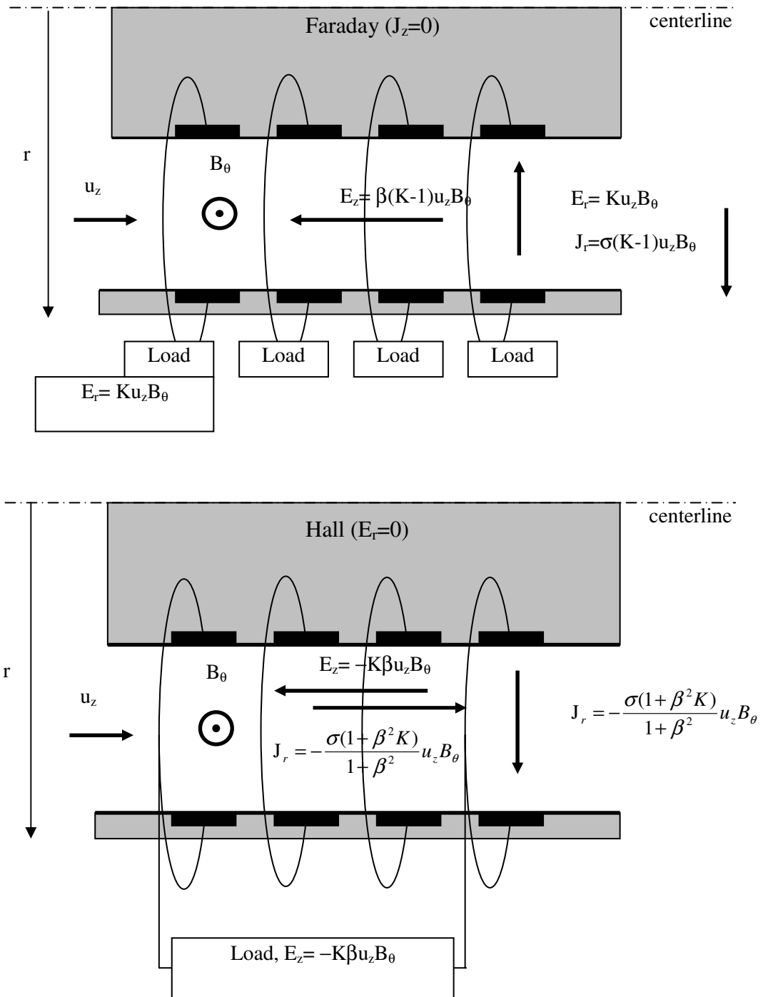
Figure 3.—Electrode configurations for the Faraday and Hall accelerators.
