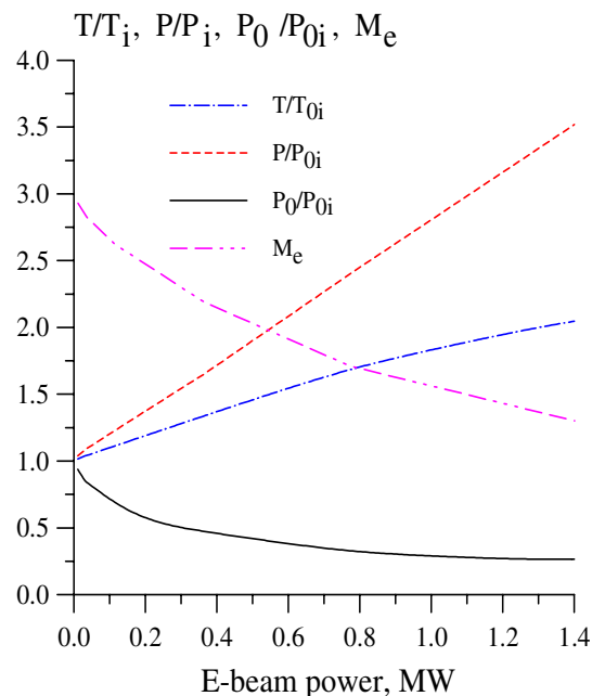
Figure 12.—Static temperature and pressure and stagnation pressure as functions of the absorbed e-beam power. Faraday accelerator, K = 0.5
