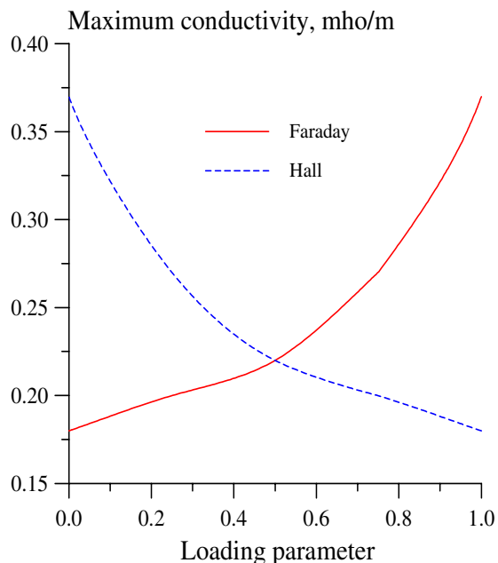
Figure 8.—Maximum electrical conductivity as a function of the loading parameter. E-beam load is 1 eV/molecule/sec
