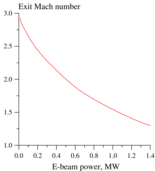
Figure 9.—Exit Mach number as a function of the absorbed e-beam power. Faraday accelerator, K = 0.5
