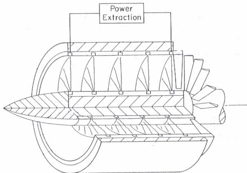
Figure 1.—Concept vehicle showing MHD energy bypass of a turbojet and potential energy management system.
