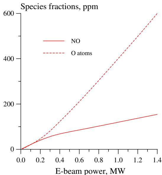
Figure 13.—Exit species concentrations as functions of the absorbed e-beam power. Faraday accelerator, K = 0.5
