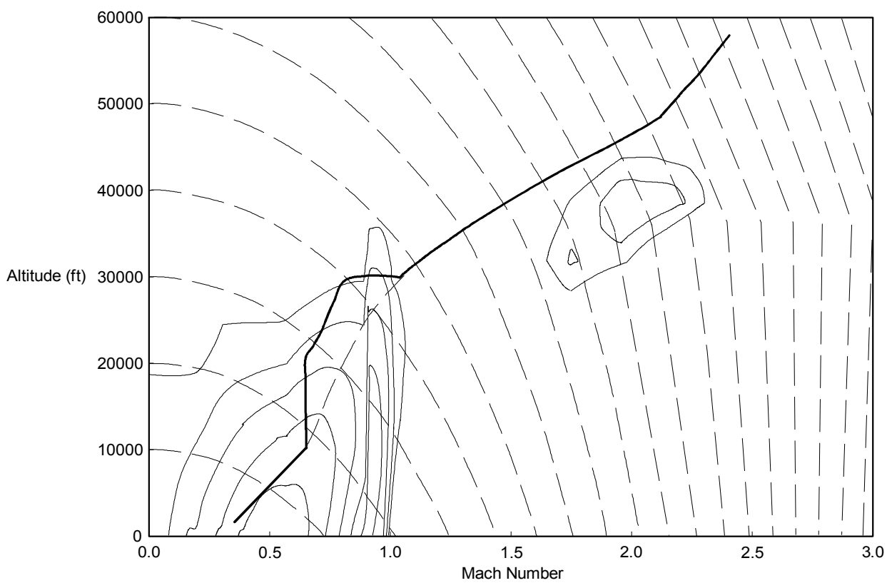
Figure 24: Lofted Trajectory with 747-400 L_5 Plus 5 dBA Noise Constraint
