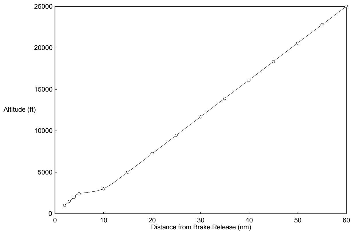
Figure 23: Typical B747-400/PW4056 Trajectory
