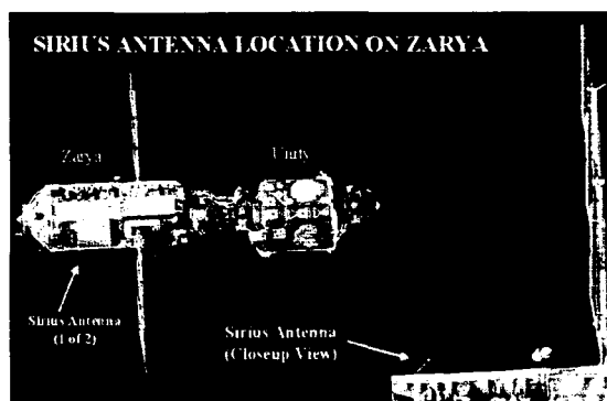
FGB 2 Meter Antenna Locations Figure 1
