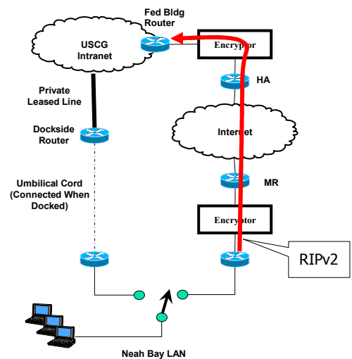
Figure 5. Dual Networks
