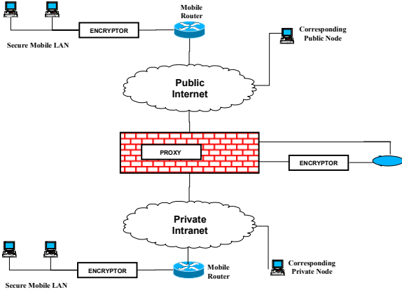
Figure 10. Mixing Private and Public Address Space
