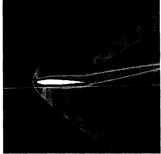
Figure 69: Mach Contours for Supersonic Viscous NACA-0012 Flow Curved Wall with Interpolated Reference Points
