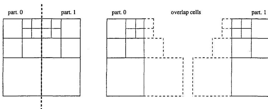
Figure 28: Overlapping Cell Configuration for flowCart
