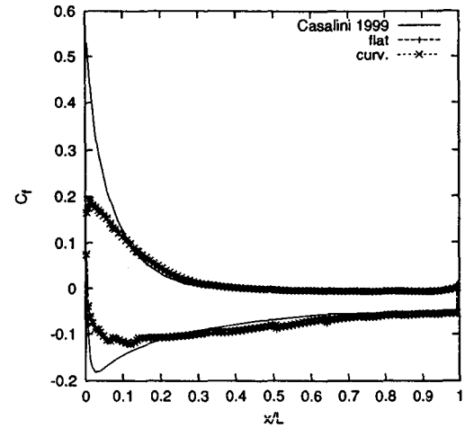
Figure 62: Subsonic Viscous NACA-0012 Skin Friction Coefficient Interpolated Reference Points
