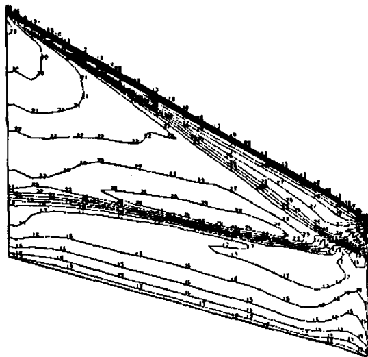
Figure 79: Transonic Inviscid ONERA M6 Upper Surface Mach Contours from [119]
