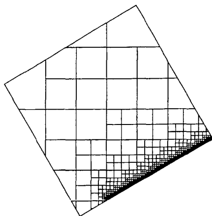
Figure 21: Grid from Coirier [38] for Rotated Blasius Flat Plate
