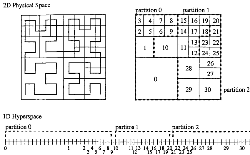
Figure 17: Two-Dimensional Mapping from Physical Space to Hyperspace
