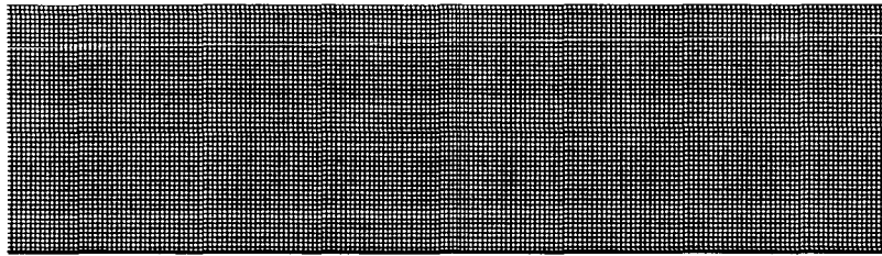
Figure 43: Final Computational Domain for Incompressible Flat Plate Flow
