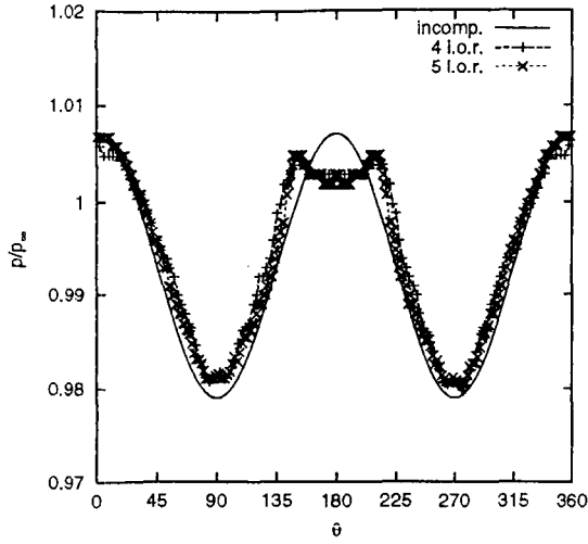
Figure 34: Fine Grid Incompressible Cylinder Surface Pressure Flat Wall with Interpolated Reference Points
