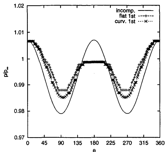
Figure 32: Incompressible Cylinder Surface Pressure 1st Order Solution with Interpolated Reference Points
