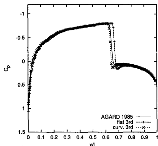
Figure 56: Transonic Inviscid NACA-0012 Lower Surface Pressure Coefficient with Interpolated Reference Points
