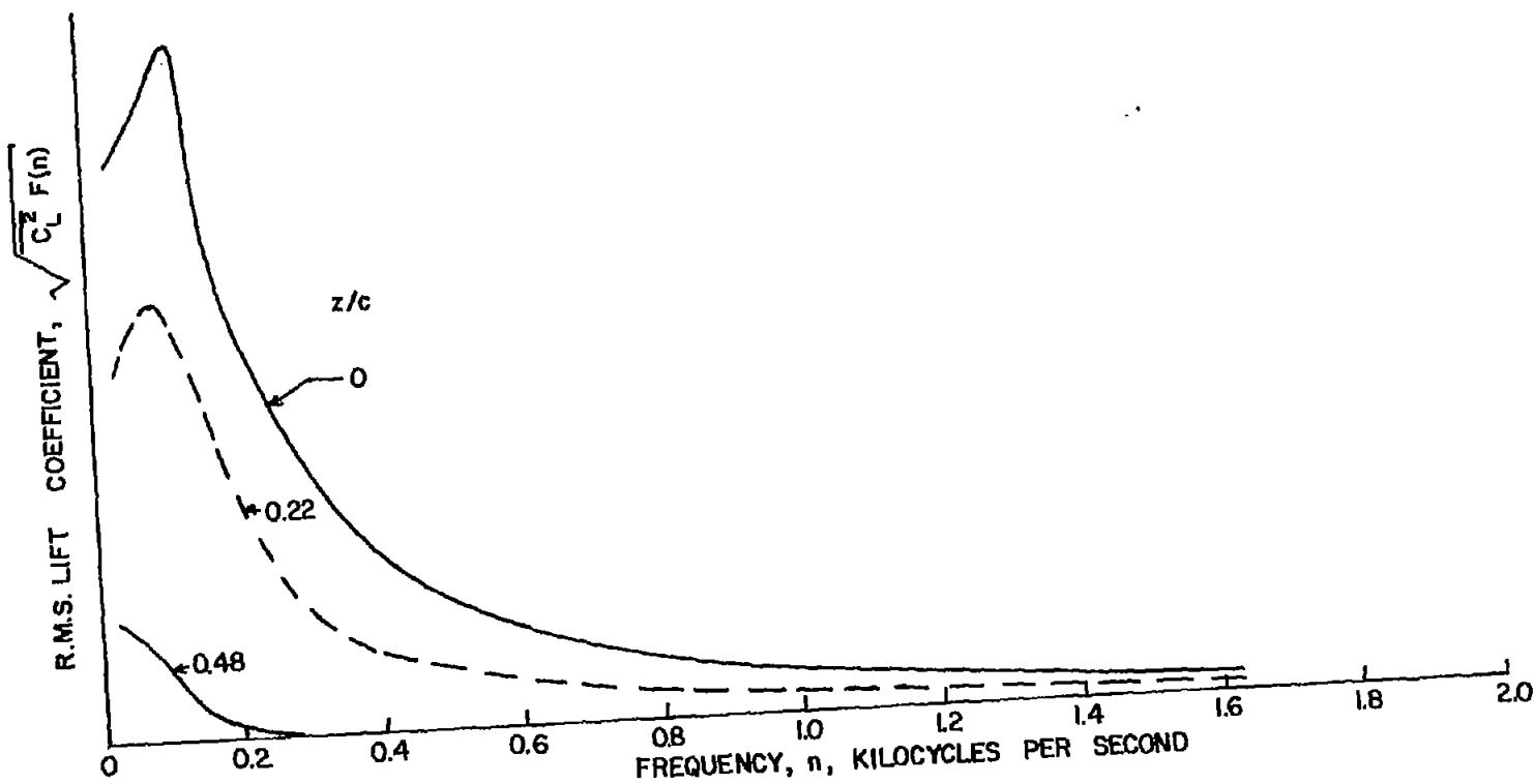
Figure 38.- Effect of tail height on the estimated frequency distribution of RMS lift on a 1.2 inch chord airfoil in the wake of a 6 inch chord airfoil; \alpha = 6^{\circ}20' , U_{\infty} = 53.5 fps, x = 1c , half band 30 cps.
