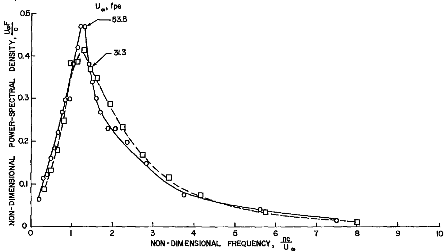
Figure 34.- Effect of free-stream velocity on the power spectrum of w^2 fluctuations; \alpha = 6^{\circ}20' , x = lc , z = 0 .
