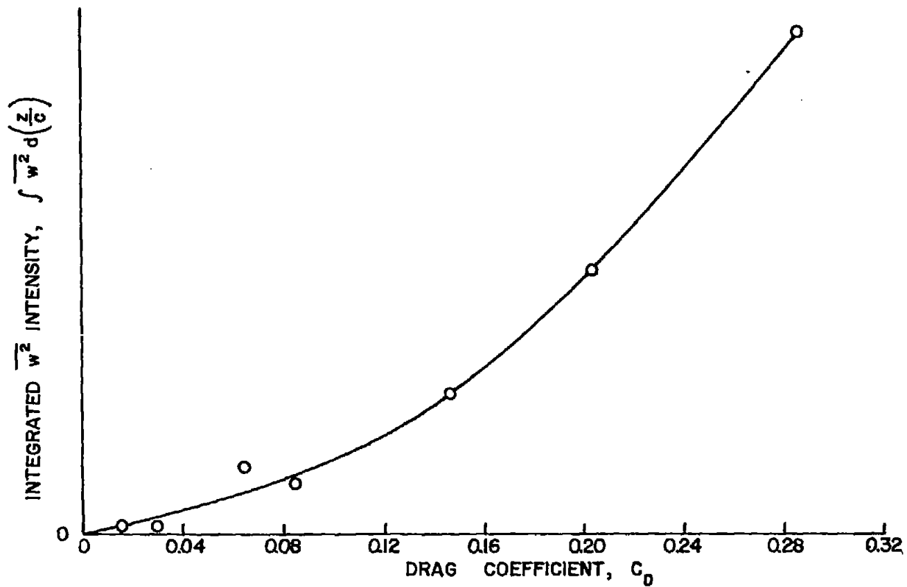
Figure 13.- Variation of integrated \overline{w^2} intensity with drag coefficient; x = 1c , U_\infty = 50 fps (nominal).
