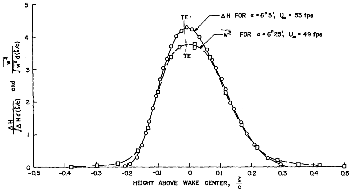
Figure 5.- Total-head and w^2 profiles measured 1 chord length behind wing trailing edge at nominal incidence of 6 degrees.
