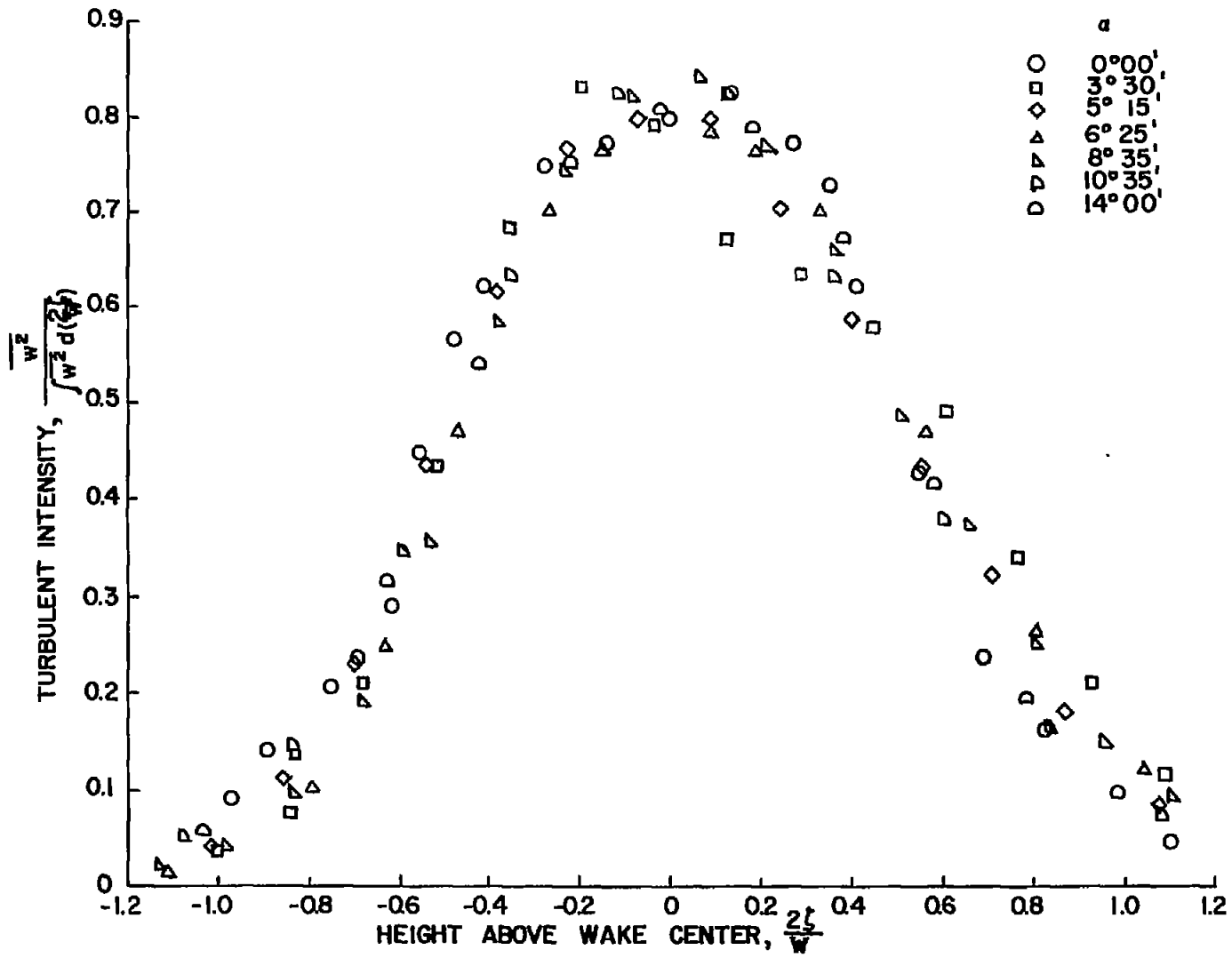
Figure 10.- Comparison of w'^2 profiles for several angles of attack; x = 1c , U_\infty = 50 fps (nominal).
