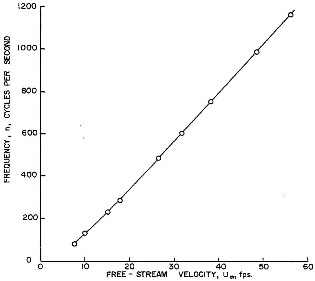
Figure 32.- Variation of frequency with free-stream velocity; \alpha = 0 , x = lc , z = 0 .
