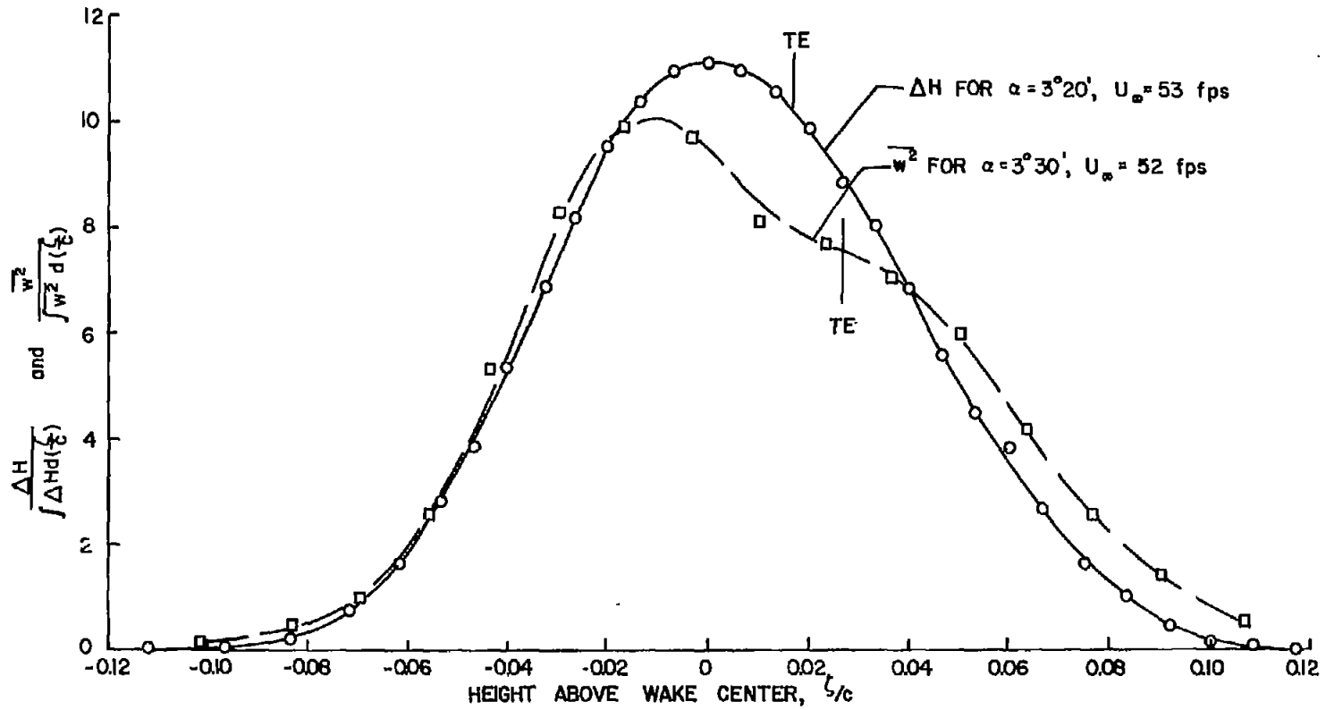
Figure 4.- Total-head and w^2 profiles measured 1 chord length behind wing trailing edge at nominal incidence of 3 degrees.
