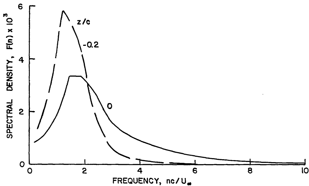
Figure 16.- RMS downwash intensity and w^2 power spectrum measured 1 chord length behind trailing edge; \alpha = 5^\circ 15' , U_\infty = 52 fps.
