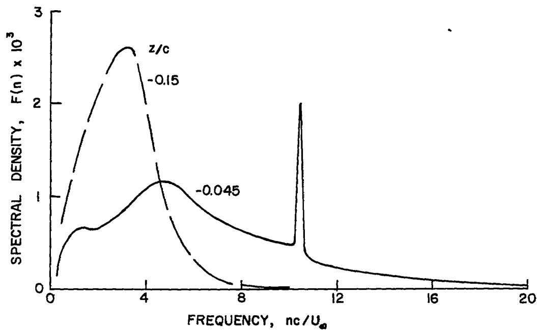
Figure 15.- RMS downwash intensity and w^2 power spectrum measured 1 chord length behind trailing edge; \alpha = 3^\circ 30' , U_\infty = 52 fps.
