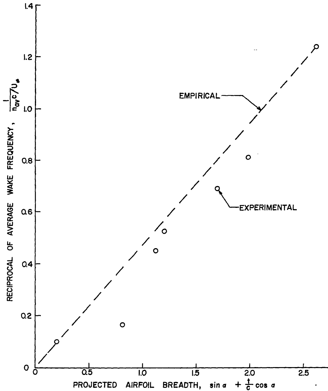
Figure 23.- Dependence of average wake frequency on projected airfoil breadth.
