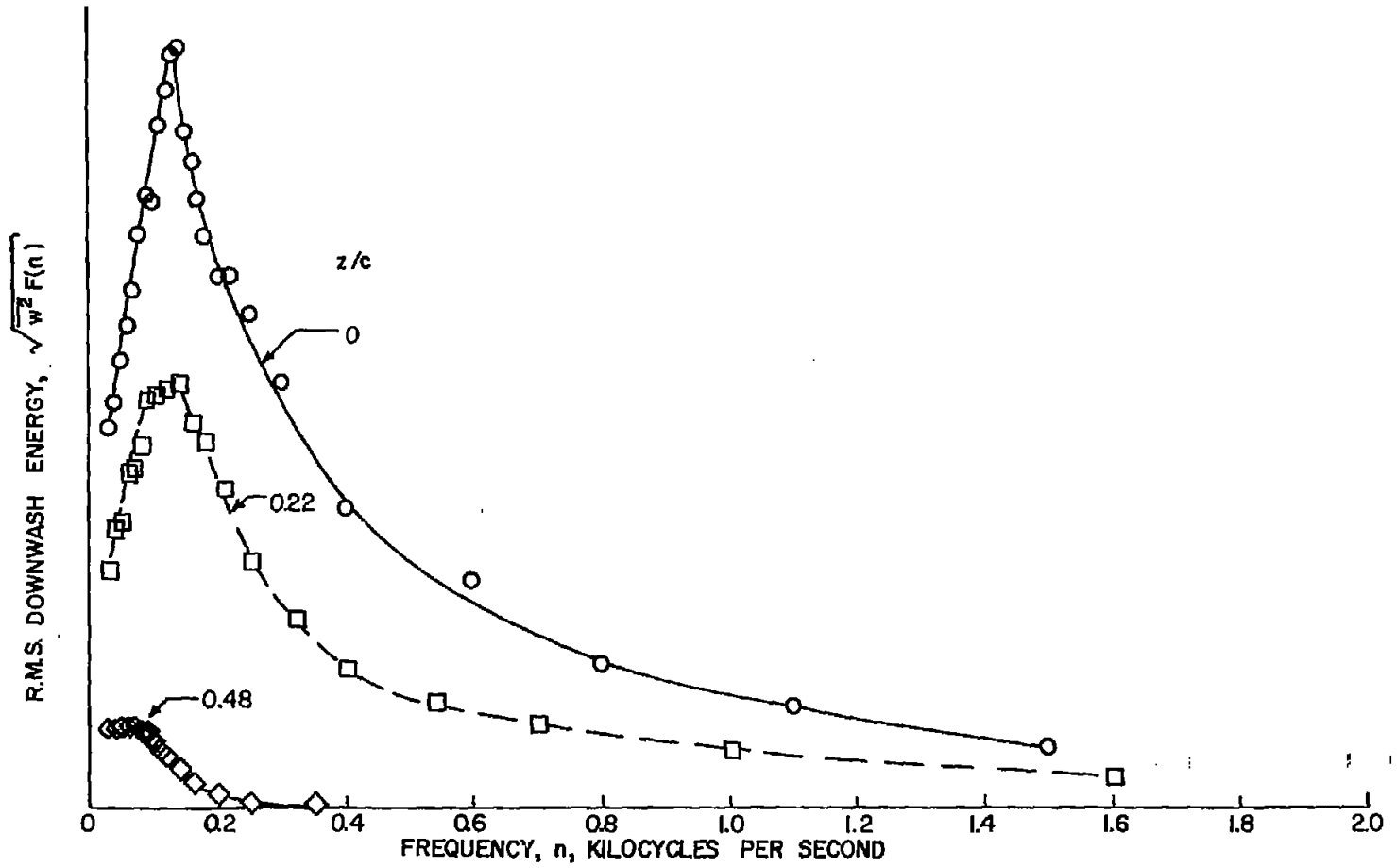
Figure 37.- Effect of tail height on the frequency distribution of RMS downwash energy; \alpha = 6^{\circ}20' , U_{\infty} = 53.5 fps, x = 1c , half band 30 cps.
