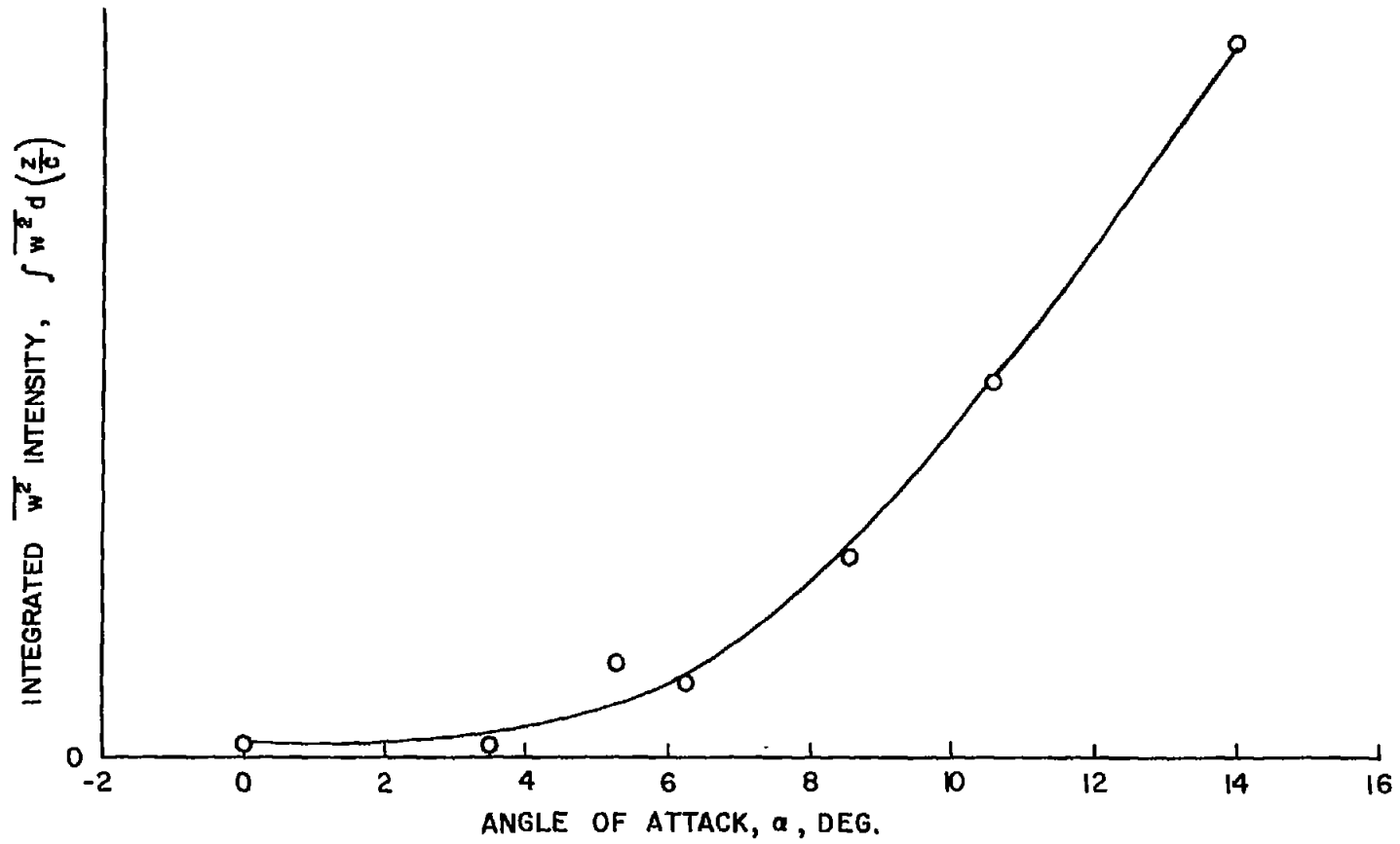
Figure 12.- Variation of integrated w^2 intensity with angle of attack, x = 1c , U_\infty = 50 fps (nominal).
