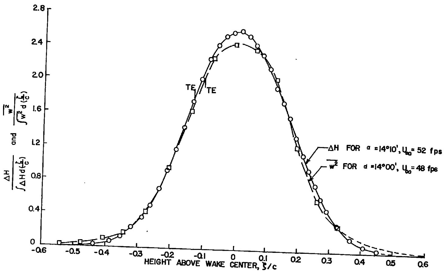
Figure 7.- Total-head and \overline{w^2} profiles measured 1 chord length behind wing trailing edge at nominal incidence of 14 degrees.
