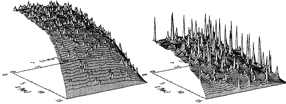
Figure 19. Simulated distribution of 1 GeV (left) and 1 TeV (right) protons at z = 0 . Adopted from Strong and Moskalenko (2001b).
