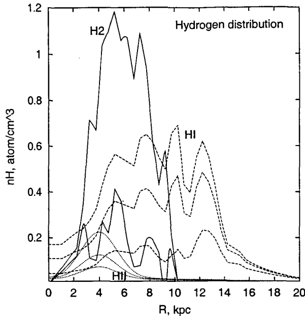
Figure 5 Number density distributions of 2\times H_2 (solid), H\ I (dashes), and H\ II (dots) in the Galaxy. Shown are the plots for z = 0, 0.1, 0.2 kpc (decreasing density). Number density of H_2 at z = 0.2 kpc from the plane is very low and is not shown in the plot. Adapted from Moskalenko et al. (2002).
