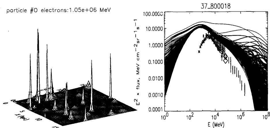
Figure 18. Simulated distribution of 1 TeV electrons at z = 0 (left) and spectral variations in 4 < R < 10 kpc (right) for t_{\text{SNR}} = 10^5 yr. Data points: locally measured electron spectra. Adopted from Strong and Moskalenko (2001a).
