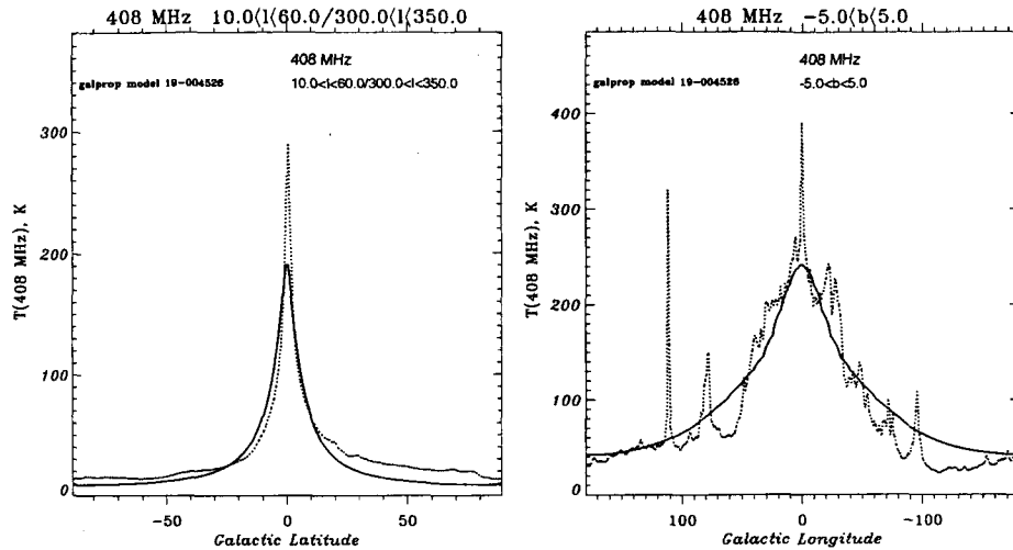
Figure 9. Intensity profiles of synchrotron emission at 408 MHz in latitude ( 10^\circ \leq l \leq 60^\circ , 300.0 \leq l \leq 350.0 ) and longitude as calculated in “hard electrons and modified nucleons” (HEMN) model. Data: Haslam et al. (1982). Adapted from Strong et al. (2000).
