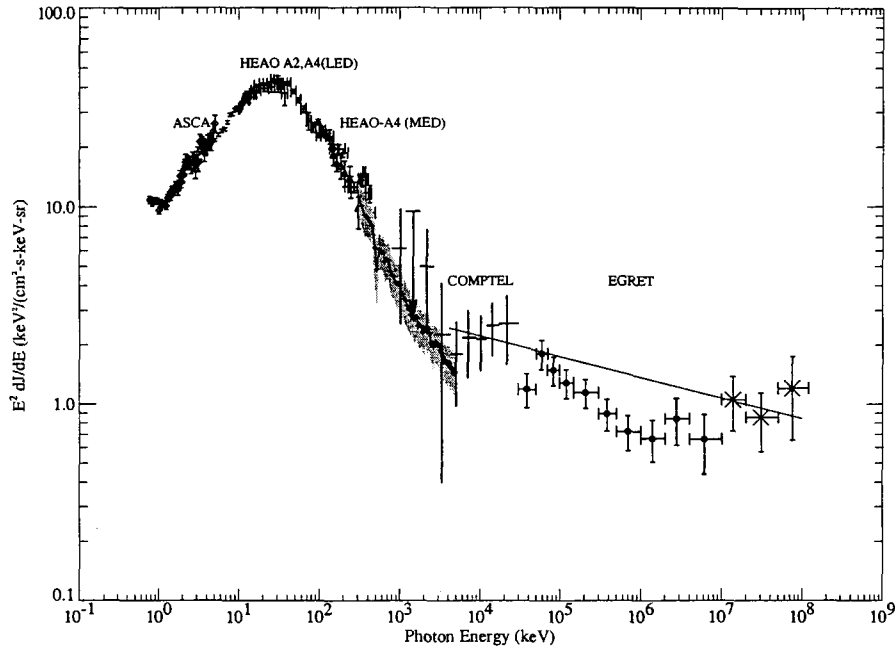
Figure 21. Spectrum of the extragalactic diffuse \gamma -ray emission. The solid line (a power-law fit with index -2.1) and three data points marked by cross in the EGRET energy range is the EGB as derived by Sreekumar et al. (1998). The closed circles with error bars below the line show our new determination of the EGB. Adapted from Strong et al. (2003b).
