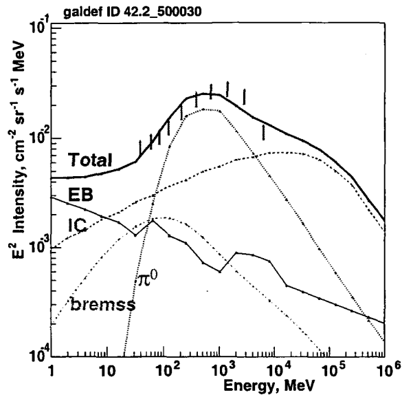
Figure 11 Spectrum of the Galactic diffuse \gamma -ray emission from the Galactic plane excluding the inner Galaxy ( 30^\circ < l < 330^\circ , |b| < 5^\circ ). The components shown are inverse Compton (IC), electron bremsstrahlung (brems), \pi^0 -decay ( \pi^0 ), extragalactic diffuse emission (EB). EGRET data are shown by error bars. Adapted from Strong et al. (2003a).
