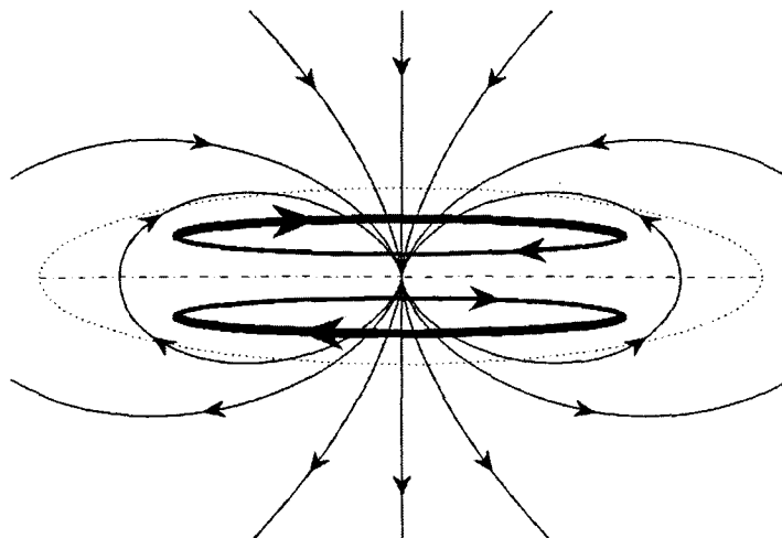
Figure 7. The rotation measures of extragalactic radio sources show the antisymmetric field structure of the Galactic halo (A0 dynamo). Adapted from Han (2003).
