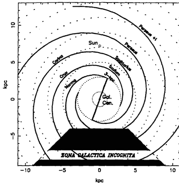
Figure 4 Model of logarithmic spiral arms. The sun is shown by the circled dot. Dots show the concentric circles at the Galactocentric radii 1, 3, 5, 7, 9, 11, 13 kpc. Adapted from Vallée (2002).
