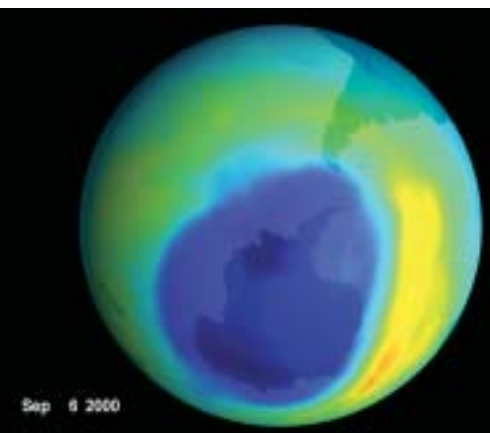
TOMS image of largest-ever ozone hole over Antarctica.
