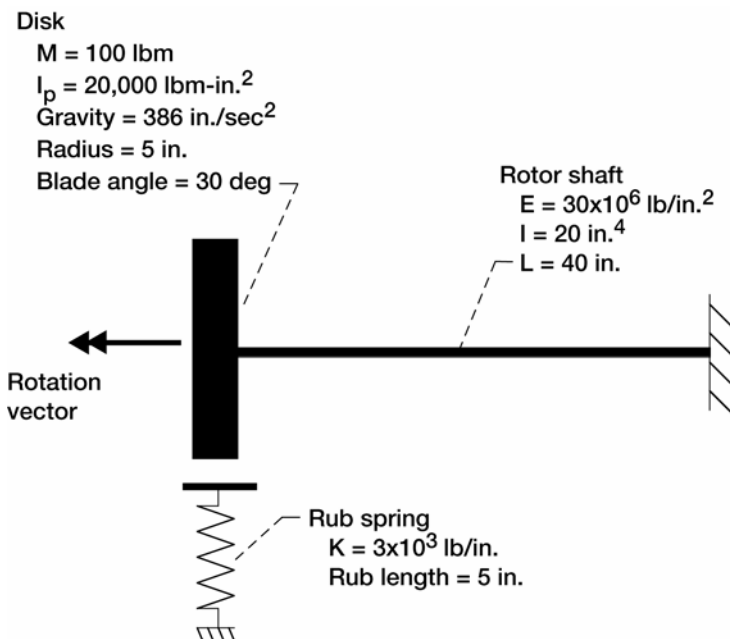
Figure 2.—Cantilever rotor.
