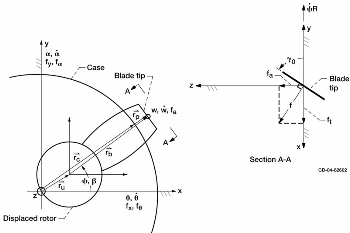
Figure 1.—Schematic of rotor blade, degrees of freedom and tip penetration.
