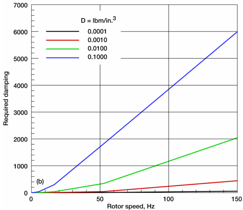
Figure 3.—Rotor stability. (a) Whirl frequency at stability/instability boundary. (b) Required damping at stability/instability boundary.
