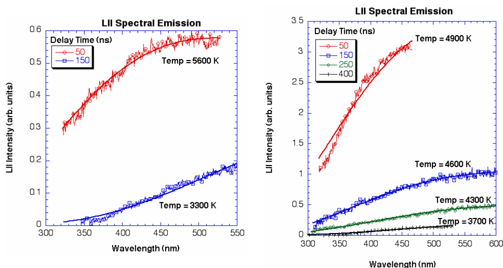
Figure 2.—Spectrally resolved emission signals collected at the indicated times after the excitation laser pulse. The blackbody curve fits are the solid lines.
