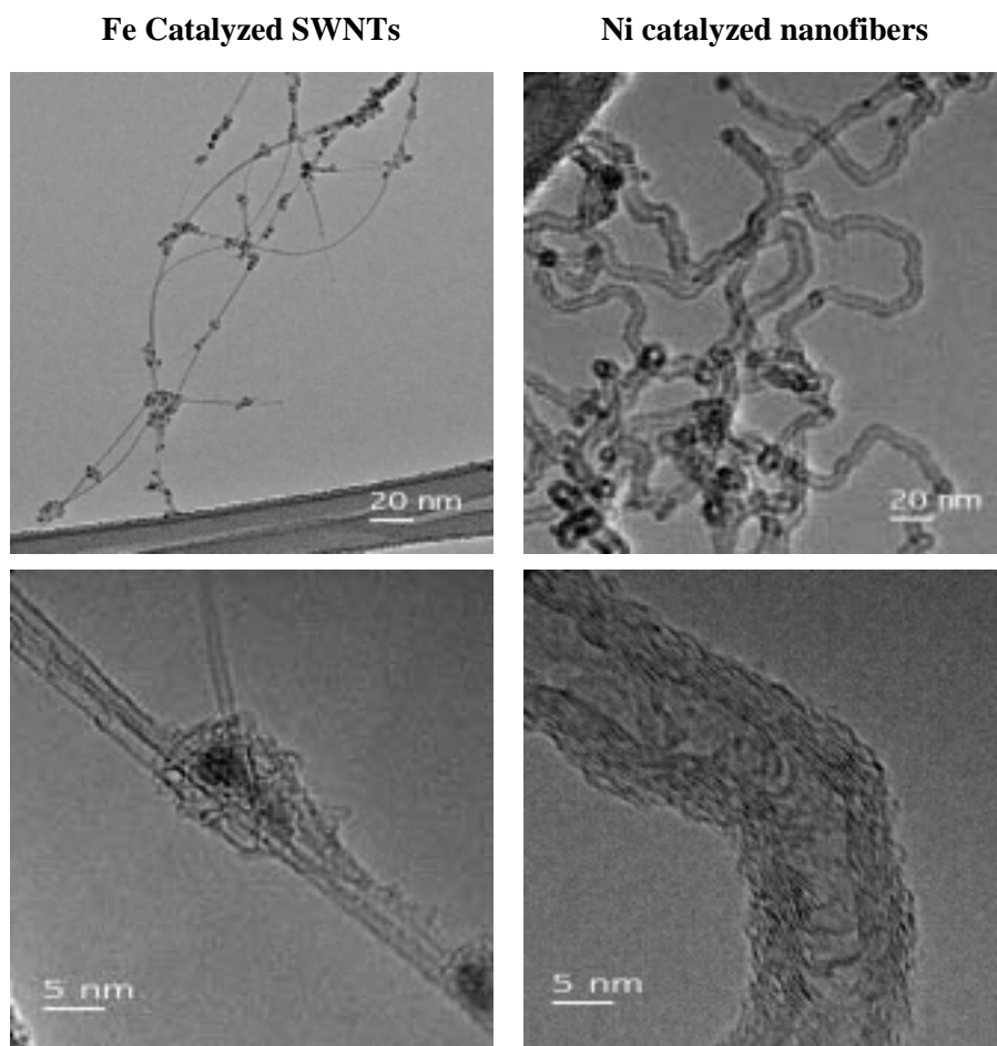
Figure 1.—HRTEM images of Fe catalyzed SWNTs and Ni catalyzed nanofibers collected from the pyrolysis flame. The images show the material as sampled directly from the flame, without purification or processing.
