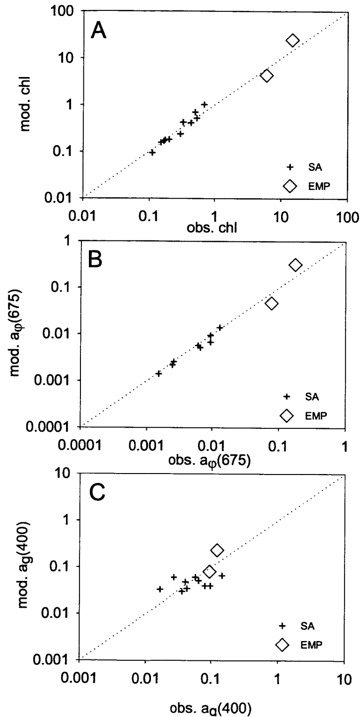
Figure 16. Algorithm performance for domain-sorted California upwelling data (Ca19704) (a) observed versus modeled [chl a ], (b) observed versus modeled a_{\phi}(675) , and (c) observed versus modeled a_g(400) . The lines are one-to-one lines, SA (+) indicates points that are calculated semi-analytically or by a blend of semi-analytical and empirical values, while EMP ( \diamond ) indicates points that are calculated empirically.
