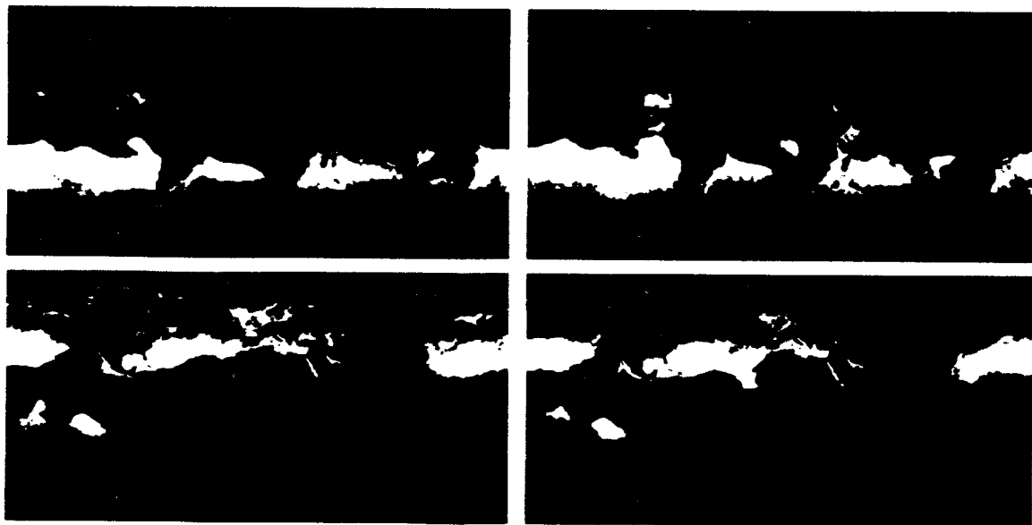
Fully-packaged SST-NDT > -1^{\circ}\text{C} Transitional 1 -1^{\circ}\text{C} > \text{SST-NDT} > 1.5^{\circ}\text{C} Transitional 2 1.5^{\circ}\text{C} > \text{SST-NDT} > 4^{\circ}\text{C} Unpackaged SST-NDT > 4^{\circ}\text{C}
