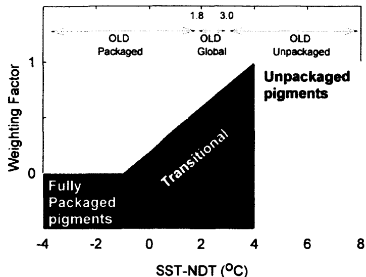
Figure 26. Comparison between previous blending mechanism (Section 5.1) for transitioning between unpackaged and packaged pigment domains and current blending mechanism (Section 6.2).
