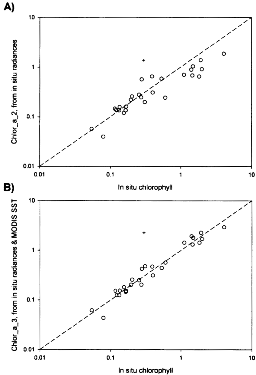
Figure 27. Relationships between in situ [Chl a ] ( \text{mg m}^{-3} ) and a) Chlor_a_2 ( \text{mg m}^{-3} ) and b) Chlor_a_3 ( \text{mg m}^{-3} ) derived from shipboard in situ radiance data. One erroneous point (+) from the February 2002 Plumes and Blooms experiment was omitted due to strong vertical structure in chlorophyll. The dashed line is the one-to-one line.
