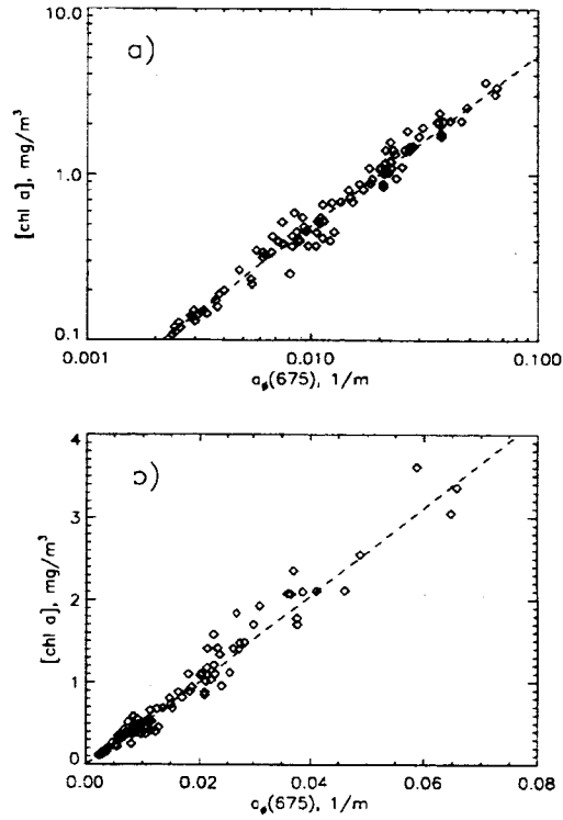
Figure 4. The [\text{chl } a] versus a_p(675) in (a) logarithmic scaling and (b) normal scaling. In both charts the dashed line is the equation [\text{chl } a] = 56.8 [a_p(675)]^{1.03} , which is the result of linear regression on the log-transformed values ( n=96 , r^2=0.97 ).
