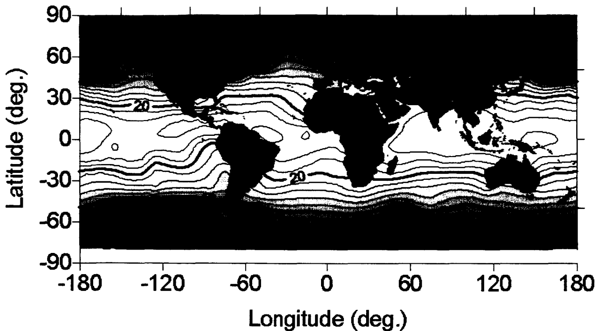
Figure 25. Global plot of nitrate depletion temperatures ( ^{\circ}\text{C} ) contoured using combined kriging and variogram (nugget effect set to 1/8^{\text{th}} of original value) approach with changes made to original [Kamykowski et al. , 2002] data.
