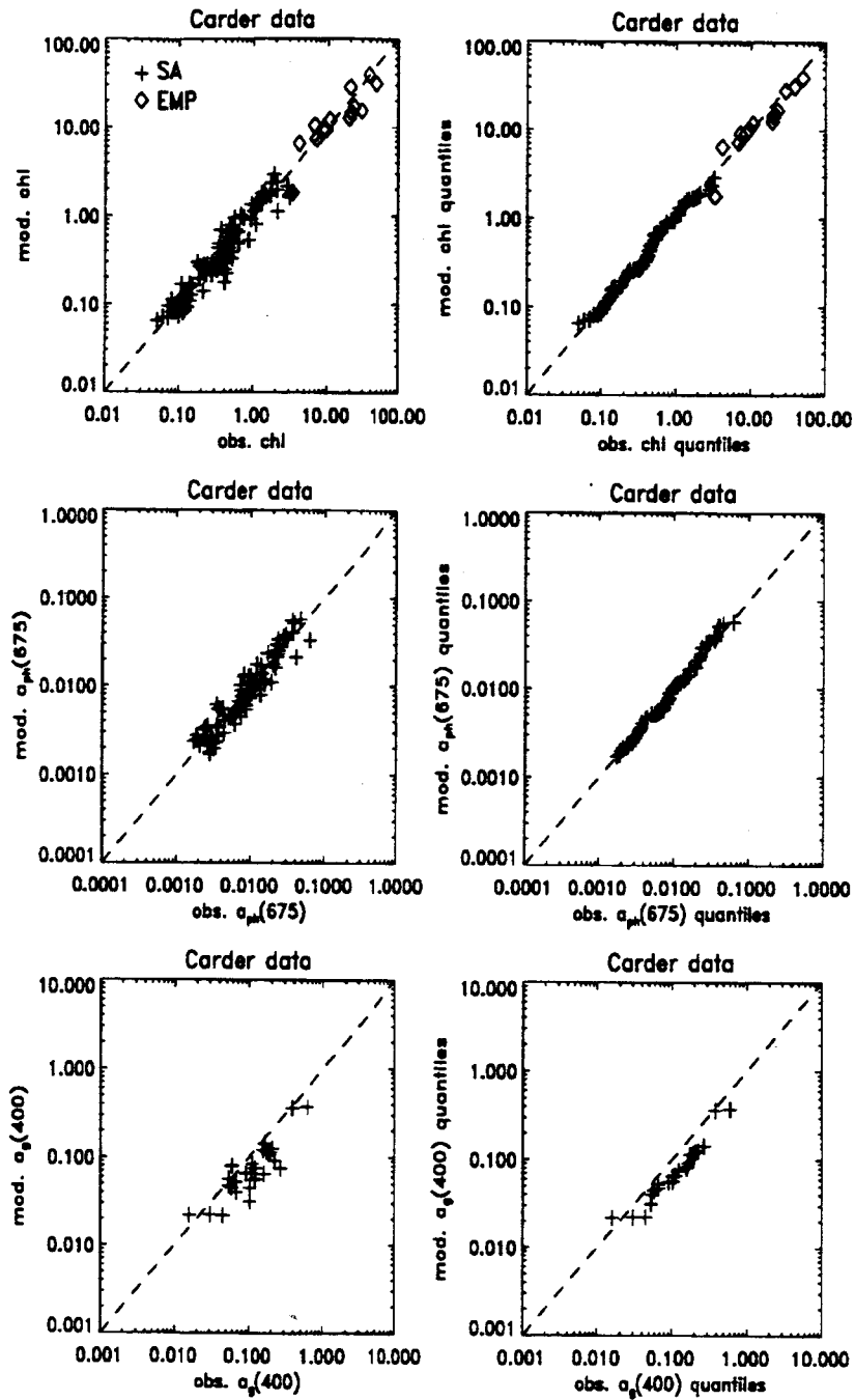
Figure 6. Algorithm performance for Carder data set, top observed versus modeled chl a, middle observed versus modeled a_{pb}(675) , and bottom observed versus modeled a_g(400) in left scatterplots and right quantile-quantile plots. The lines are the one-to-one lines, SA (crosses) indicates points that are calculated semianalytically and EMP (diamonds) indicates points that are calculated empirically.
