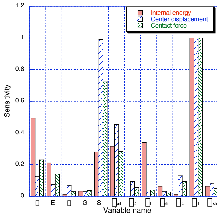
Figure 10. Normalized sensitivity of responses based on 500 Monte Carlo simulations.
