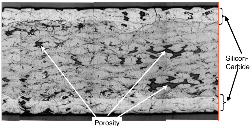
Figure 1. Micro-graph cross-section of 19-ply RCC material.
