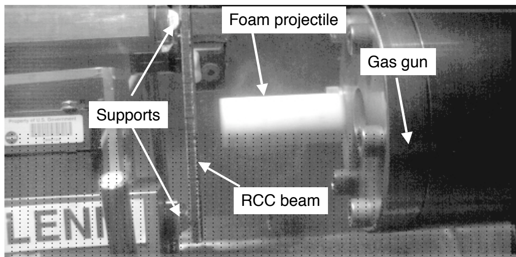
Figure 2. Photograph of beam test set-up just prior to foam impact.
