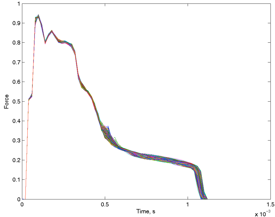
Figure 8. Contact force (non-dimensional) for 500 Monte Carlo simulations.
