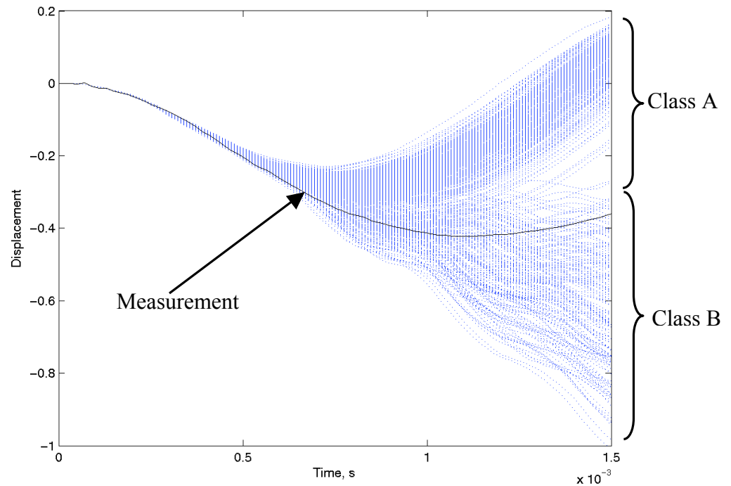
Figure 6. Measured and predicted center displacements (non-dimensional) for 555 ft/s impact.
