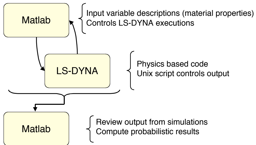
Figure 5. Schematic of probabilistic analysis.
