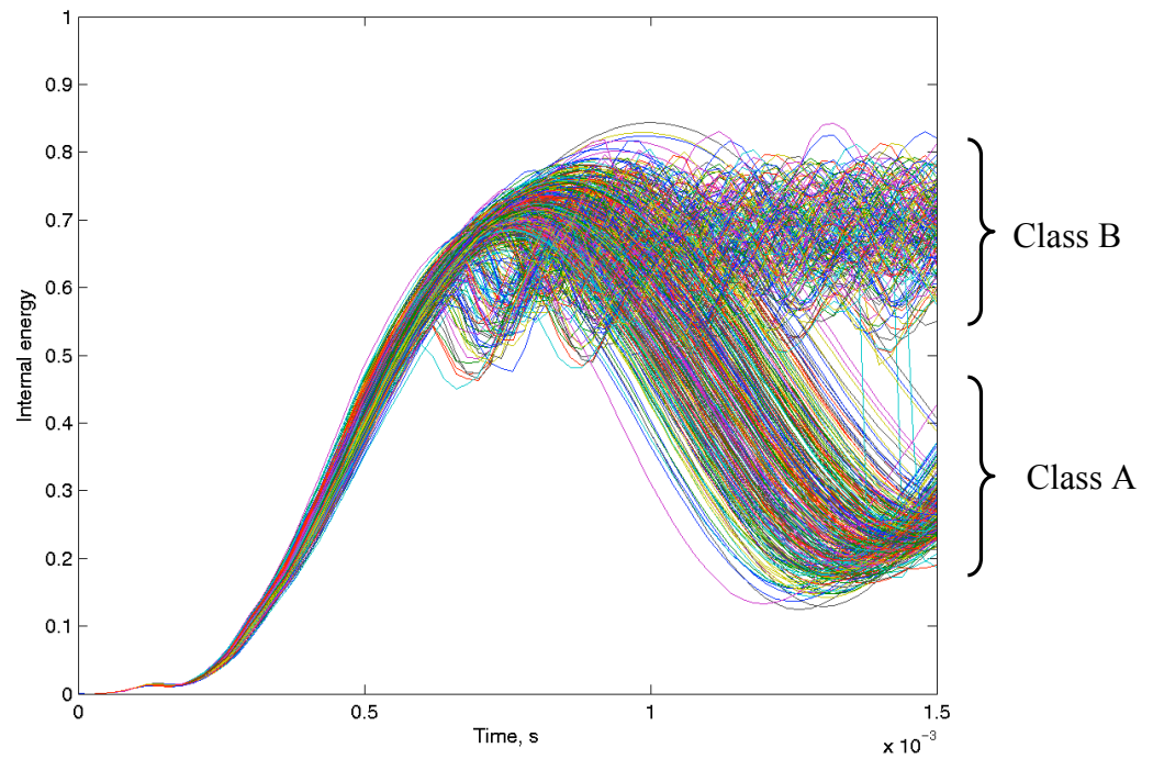
Figure 7. Beam internal energy (non-dimensional) for 500 Monte Carlo simulations.
