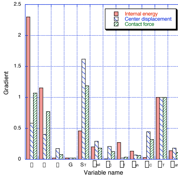
Figure 9. Normalized gradient of responses based on 500 Monte Carlo simulations.
