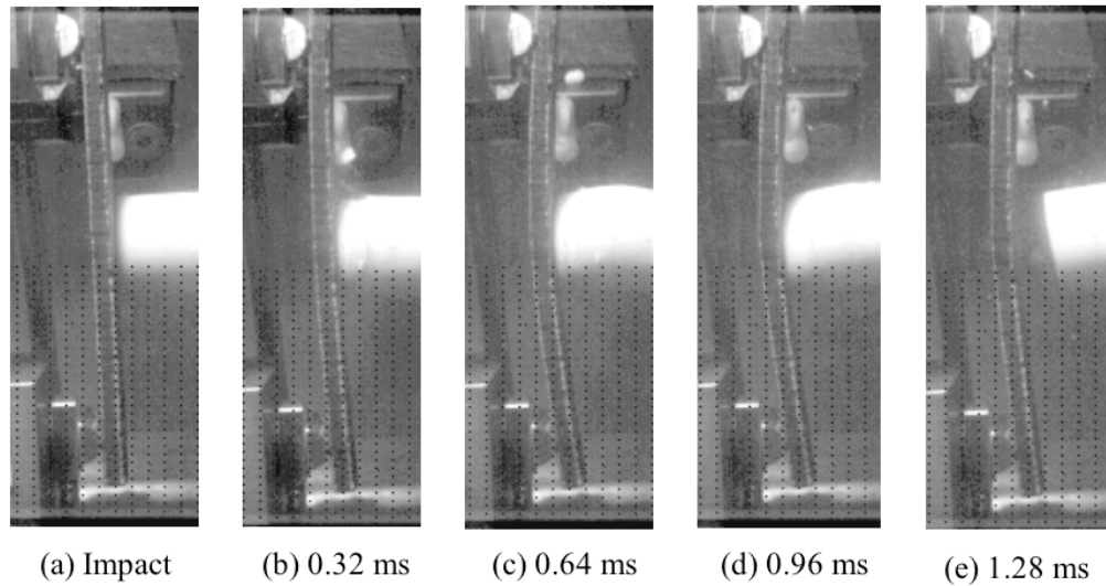
Figure 3. Series of photographs showing panel impacted by foam cylinder.
