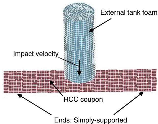
Figure 4. Finite element model.
