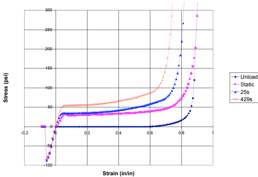
Figure 5. BX-250 Foam Model Stress Strain Curves.
