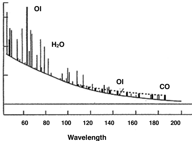
Figure 3. Predicted far infrared spectrum of a collapsing cold cloud core, from Ceccarelli, Hollenbach, and Tielens. The spectrum is dominated by [OI] and complexes of CO and H O.
