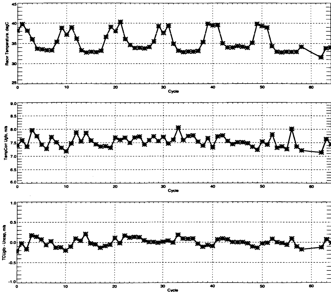
Figure 4-2 Plots of Temperature and Temperature Corrected Windspeed
