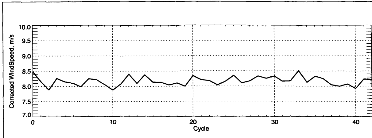
Figure B-4 Cycle-Averages Corrected Windspeed in Meters Per Second
