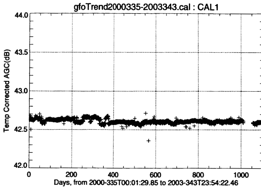
Figure 2-2 CAL-1 AGC for the First 65 Cycles
