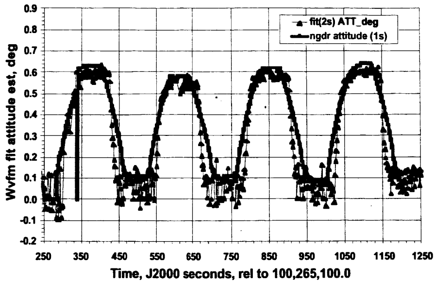
Figure 4-3 GFO Waveform Fit Attitude & NGDR Attitude in 2003/03/06 ABCAL
