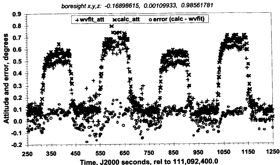
Figure 4-5 Waveform Fit & Calculated Attitudes in 2003/0710 ABCAL from WFF Boresight Vector Solution
