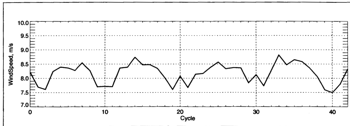
Figure B-2 Cycle-Averages Windspeed in Meters Per Second
