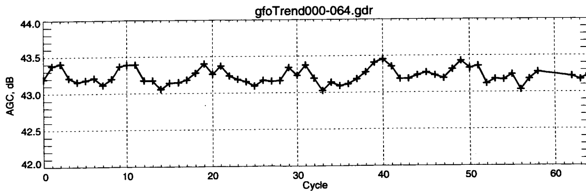
Figure 2-5 AGC Cycle-Averages in dB
