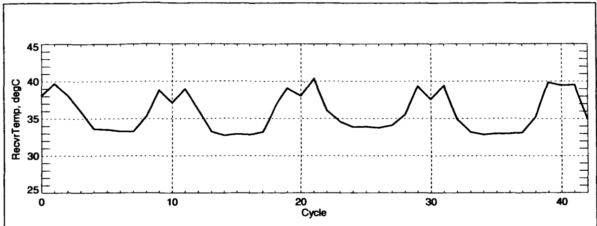
Figure B-3 Cycle-Averages Receiver Temperature in Celsius Degrees
