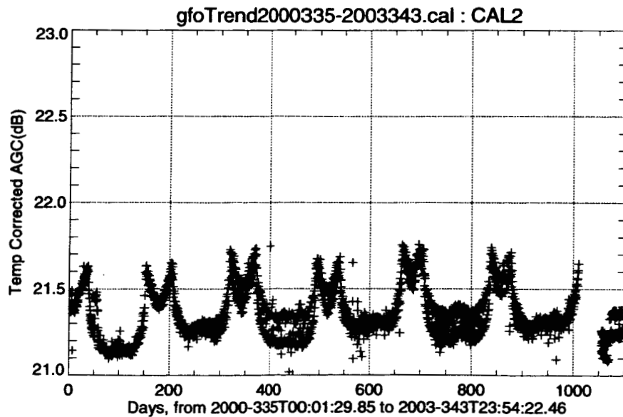
Figure 2-3 CAL-2 AGC for the First 65 Cycles
