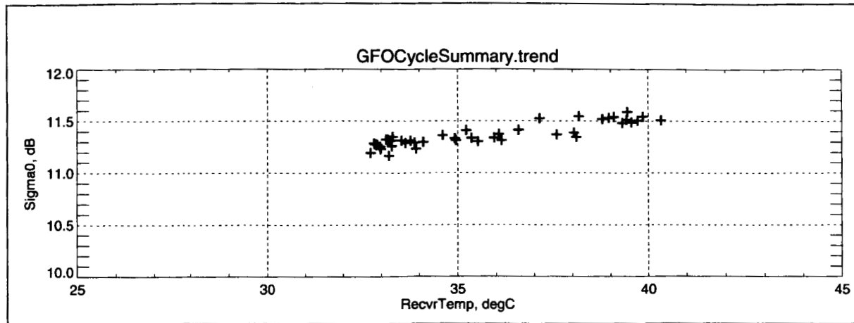
Figure B-1 Cycle-Averages Sigma0 vs. Temperature
