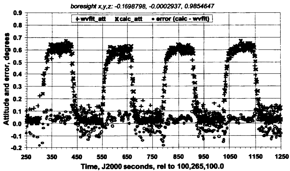
Figure 4-4 Waveform Fit & Calculated Attitudes in 2003/03/06 ABCAL from WFF Boresight Vector Solution
