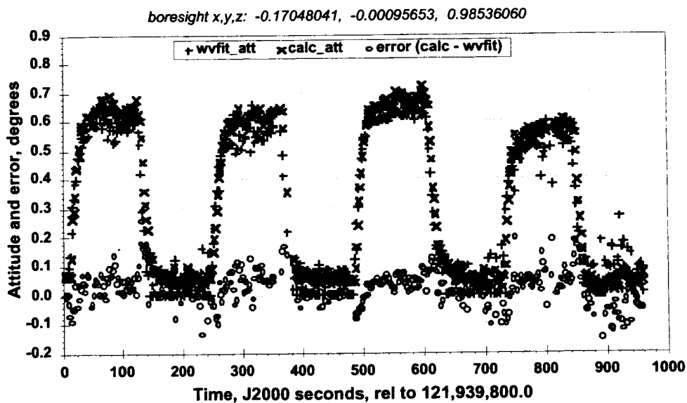
Figure 4-6 Waveform Fit & Calculated Attitudes in 2003/11/12 ABCAL from WFF Boresight Vector Solution
