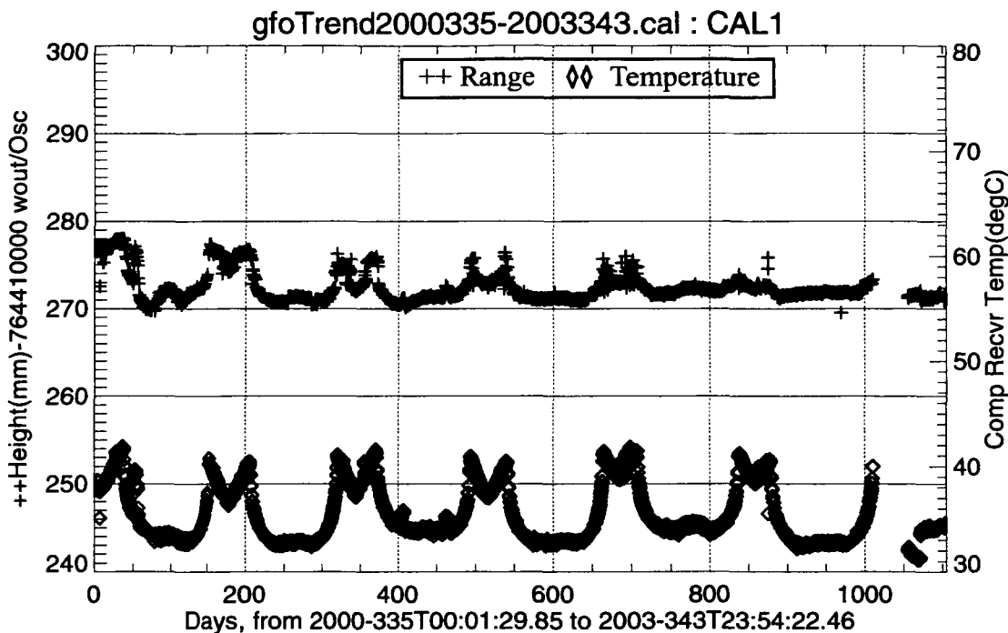
Figure 2-1 CAL-1 Range/Temperatures for the First 65 Cycles
