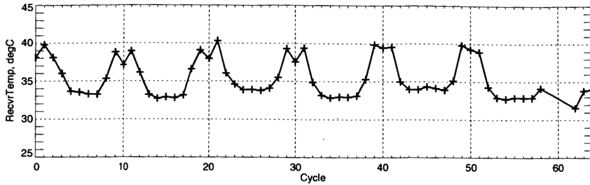
Figure 2-8 Cycle-Averages Receiver Temperature in Degrees Celsius
