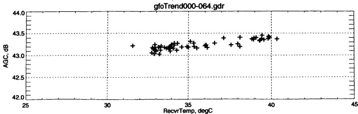
Figure 2-12 Cycle-Averages AGC vs. Temperature
