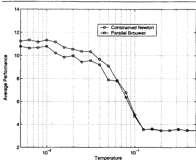
Figure 2. Comparison of RL-based and PD theory-based equilibration methods for the Bar problem. Performance is measured at the end of the run. Higher is better.
