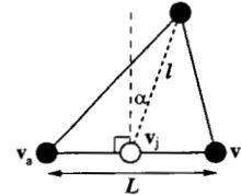
Fig. 3. Local deformation of the mesh around a wavelet coefficient as the midpoint of the edge a_1 a_2 : definition of the lengths L and l , skew angle \alpha .
