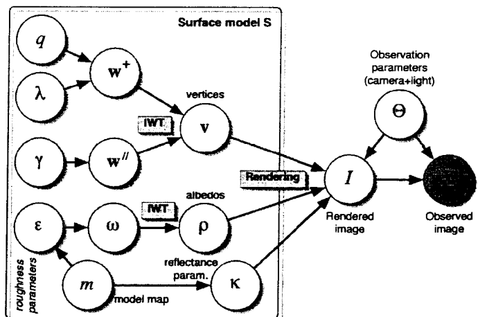
Fig. 1. Graphical model, or hierarchy of the random variables in the proposed generative model, including rendering and inverse wavelet transform (IWT).
