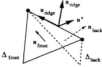
Fig. 7. Let \mathbf{u}_{\text{ridge}} be the oriented edge (according to the front-face triangle) and the ridge normal the average \mathbf{n}_{\text{ridge}} = (\mathbf{n}_{\text{front}} + \mathbf{n}_{\text{back}})/2 . The front-facing triangle \Delta_{\text{front}} is closest to the camera \Leftrightarrow |\mathbf{u}_{\text{ridge}}, \mathbf{u}^*, \mathbf{n}_{\text{ridge}}| > 0 .
