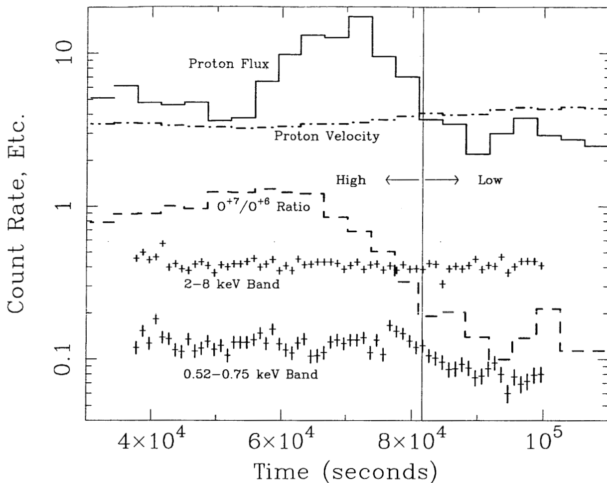
Fig. 1.— Light curves for the observation affected by the SWCX emission (HDF-N #4). The dot-dash curve shows the hourly ACE SWEPM proton velocity data in units of 100 \text{ km s}^{-1} . The solid curve shows the hourly ACE SWEPM proton flux data in units of 10^8 \text{ cm}^{-2} \text{ s}^{-1} . The dashed curve shows the hourly ACE SWICS \text{O}^{+7}/\text{O}^{+6} ratio data smoothed with a five hour running average. ACE data have not been adjusted for travel time from the L1 point to Earth (a delay of \sim 4000 \text{ s} ). The upper set of points shows the XMM-Newton MOS1 light curve for the 2–8 keV band in counts \text{s}^{-1} . The lower set of points shows the light curve for the 0.52–0.75 keV band in counts \text{s}^{-1} , which includes the O VII and most of the O VIII line emission. Periods of soft proton-flaring have been removed. The time used to separate the spectra with and without the SWCX emission is shown by the vertical line. The X-ray count rates do not have the particle background subtracted.
