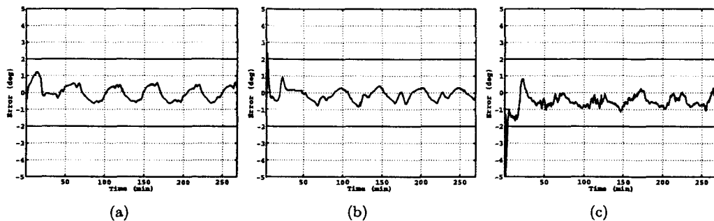
Figure 1 Attitude Errors for Day 68 of 2002 with 2 Degree Limit, (a) X Axis, (b) Y Axis (c) Z Axis
