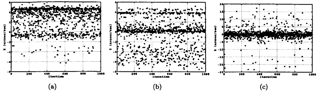
Figure 15 True Rates After 60 Minutes. (a) X Axis, (b) Y Axis, (c) Z Axis
