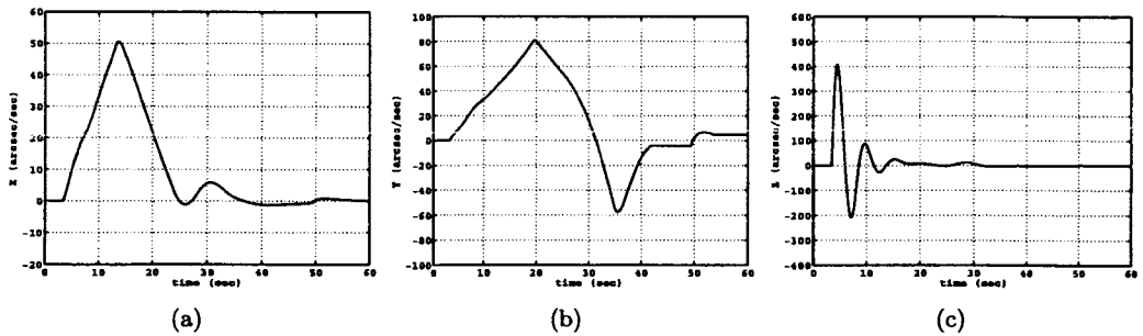
Figure 17 True Rates for 20 Degree Attitude Maneuver. (a) X Axis, (b) Y Axis, (c) Z Axis
