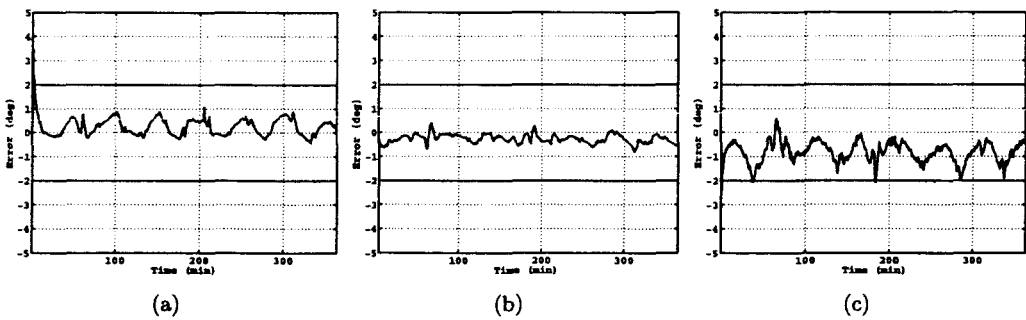
Figure 4 Attitude Errors for Day 80 of 2002 with 2 Degree Limit, (a) X Axis, (b) Y Axis (c) Z Axis
