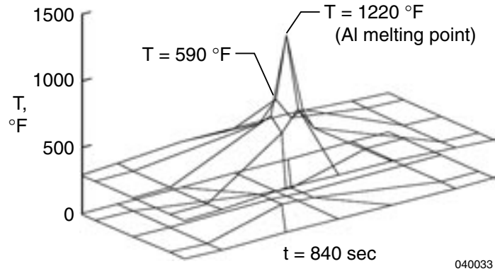
Figure 22. Windward aluminum skin temperature distributions with one missing central TPS tile (100 percent eroded, h/h_o = 0 ); modified STS-5 heating (transition at t = 800 sec).
