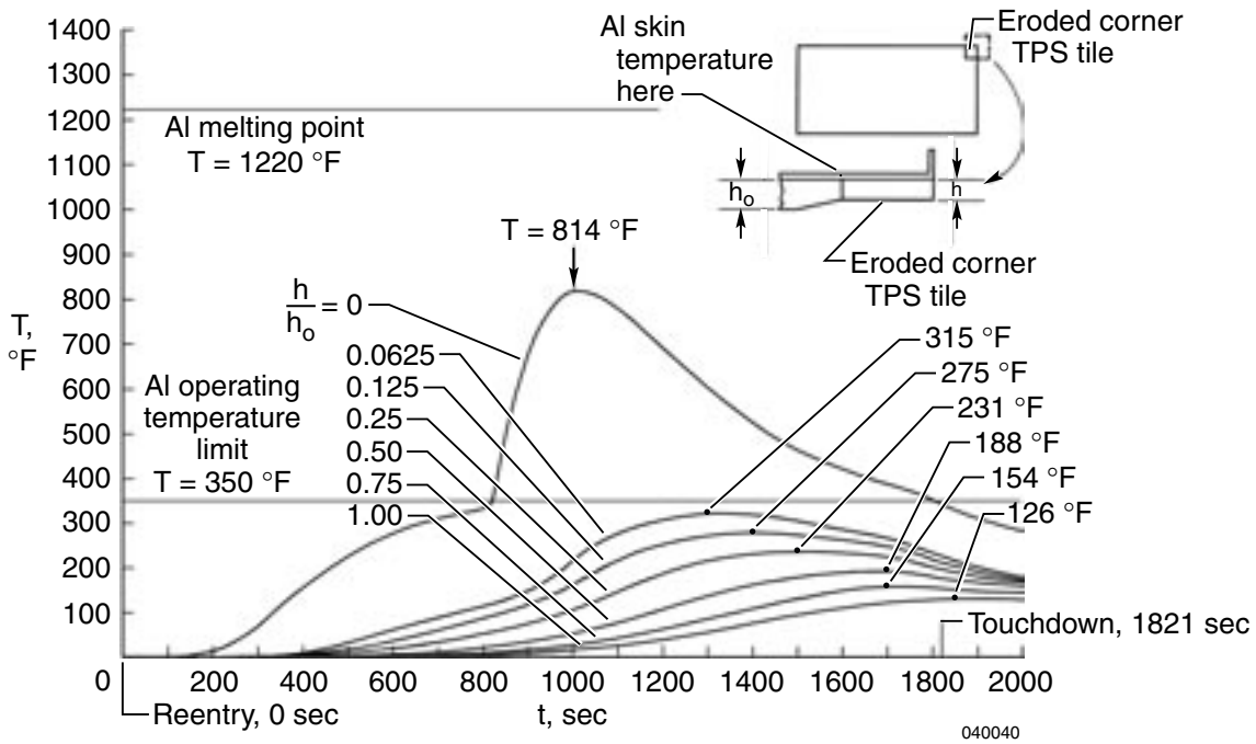
Figure 28. Variation of aluminum skin temperature with thickness of an eroded corner TPS tile; modified STS-5 heating (transition at t = 800 sec).
