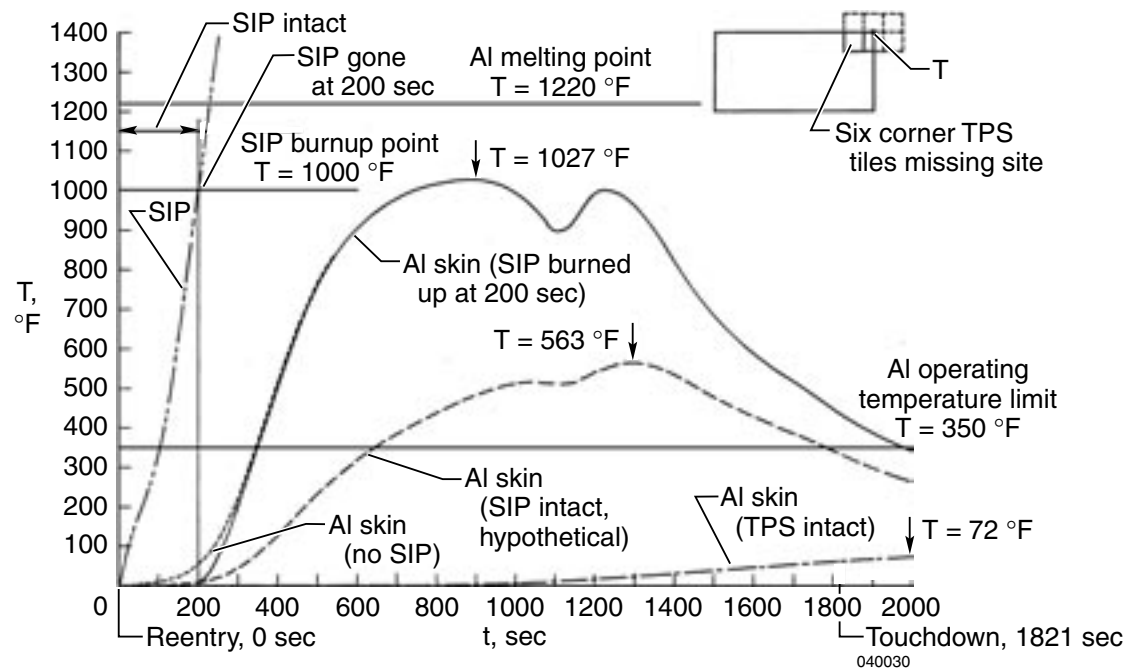
Figure 19. SIP and aluminum skin temperatures at panel corner; six corner TPS tiles missing; STS-5 heating (transition at t = 1100 sec).
