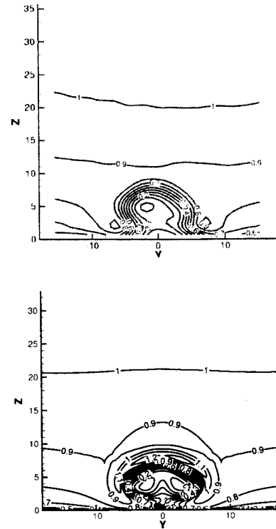
Figure 20. Example contours of phase-averaged u-velocity, 1D downstream, \text{phase}=120^\circ ; (a) PIV experiment, (b) NASA-cfi3d-sa(fine).
