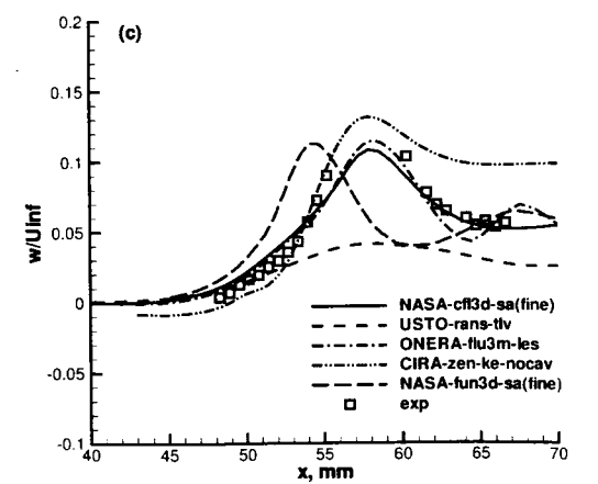
Figure 15. Case 2 average w-velocity; (a) z=10\text{mm} 1D downstream, (b) z=0.4\text{mm} and y=0 , (c) z=10\text{mm} and y=0 .
