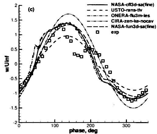
Figure 13. Case 2 time histories at x=50.63\text{mm} , y=0 , z=0.4\text{mm} : (a) u -velocity, (b) v -velocity, (c) w -velocity.
