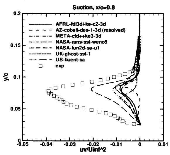
Figure 27. Sample of case 3 suction condition results at x/c=0.8 (inside separation bubble); (a) u-velocity, (b) turbulent shear stress.
