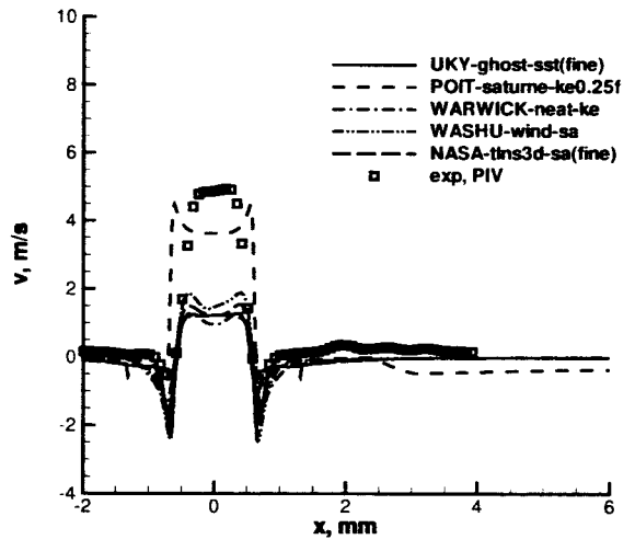
Figure 5. Case 1 average v-velocity profiles at y=0.1\text{mm} .
