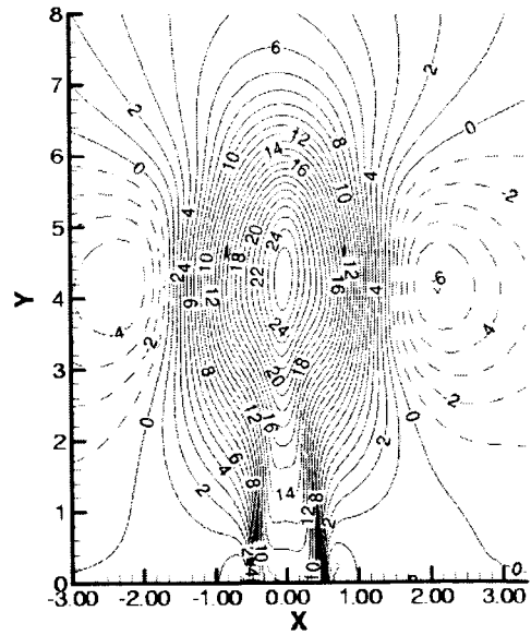
Figure 11. Case 1 contours of v-velocity, phase=135°; (a) PIV experiment, (b), NASA-tlms3d-sa(fine).
