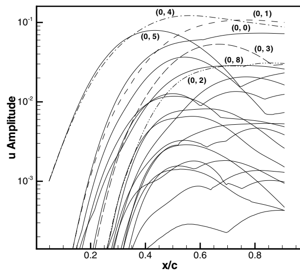
Figure 35: Evolution of disturbance amplitudes for Mach 2, 80^\circ swept wing boundary layer; nonlinear interaction of stationary crossflow instability with \lambda_z = 8 for (0, 5) mode and \lambda_z = 10 for (0, 4) mode.
